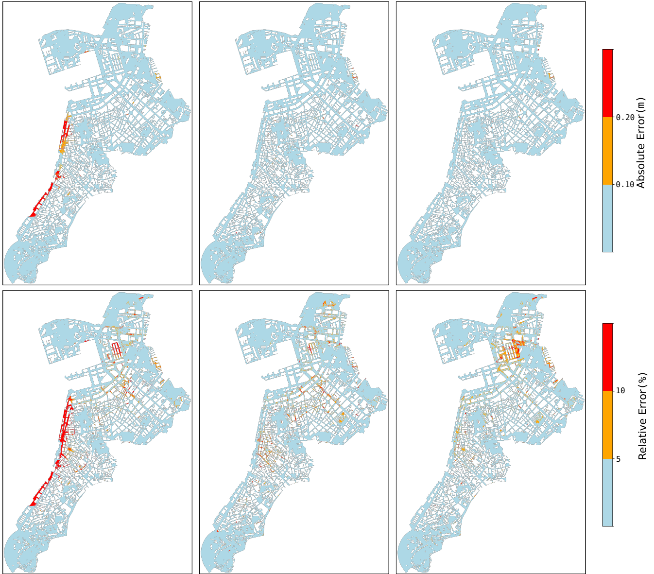
Figure 10. The absolute and relative error of maximum inundation depths.
