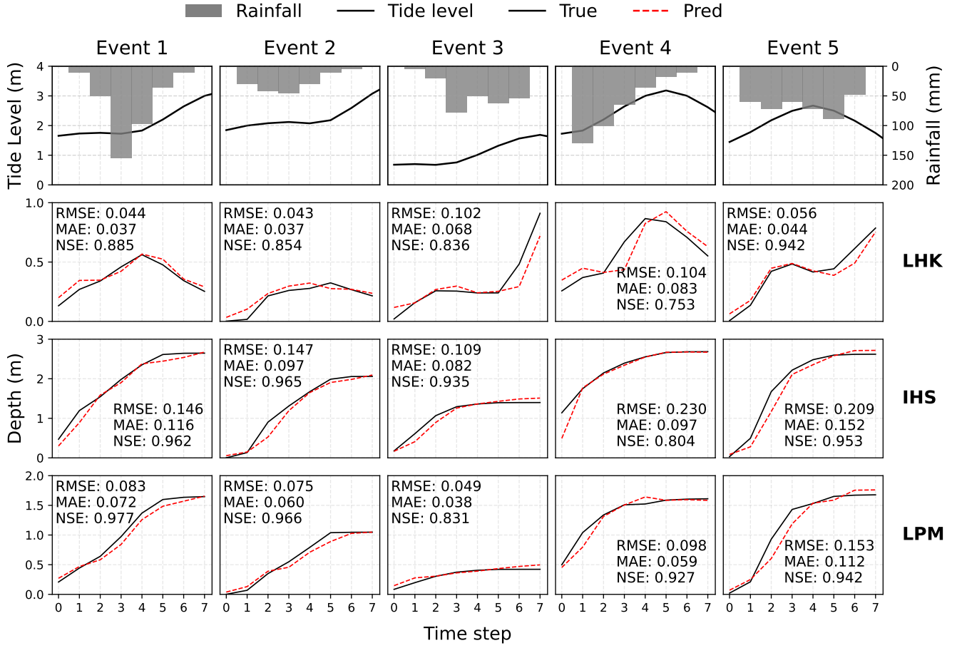
Figure 8. Comparison of water depth processes in three flood-prone locations.
