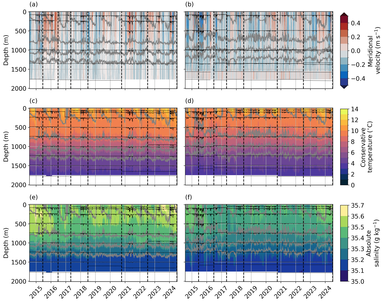
Figure 2. Gridded fields of moored meridional velocity (a-b), conservative temperature (c-d) and absolute salinity (e-f) of the concatenated mooring WB1 and WB2 (a,c,e) and EB1 (b,d,f). Black lines mark the depth derived from the pressure time series for the individual current meters (a-b) and CTD sensors (c-f). Grey contour lines show potential density values at 27.2, 27.4, 27.6 and 27.7 \text{kg m}^{-3} (top to bottom). Vertical dashed black lines indicate the individual servicing times for the moorings.
