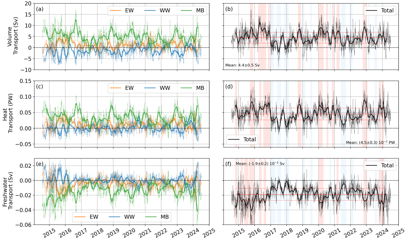
Figure 9. Rockall Trough (a,b) volume, (c,d) heat, and (e,f) freshwater transports. Panels (a,c,e) show transports for the eastern wedge (EW, orange), western wedge (WW, blue), and mid basin (MB, green); panels (b,d,f) show the total (black). Thin lines indicate unfiltered data, bold lines the 90-day low-pass-filtered data. In (b,d,f), red solid lines denote the mean total transport, and red dashed lines the \pm 1 standard deviation. In (b,d), red shading marks periods when the filtered time series exceeded the mean +1 standard deviation, and blue shading when they fall below the mean -1 standard deviation. In (f), the shading is reversed.
