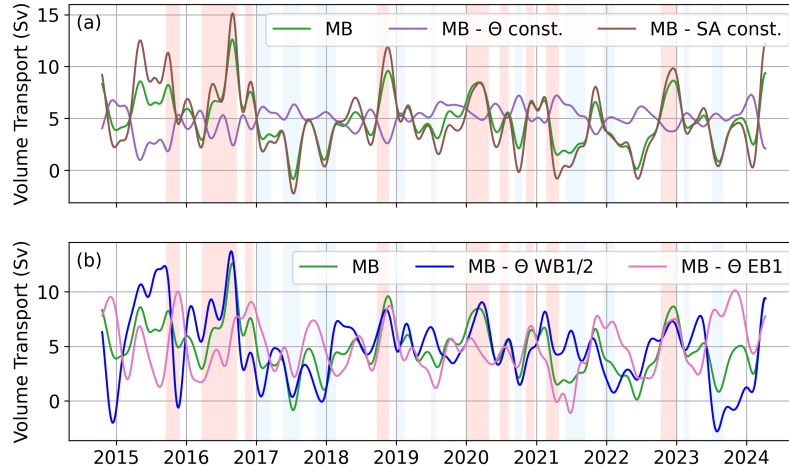
Figure 10. Time series of 90-day low-pass filtered volume transport through mid basin (MB) (a) isolating changes in salinity ( \Theta const., purple line) or temperature (SA const., brown line) and (b) isolating changes in temperature at WB1/2 (blue line) or EB1 (light pink line). The green line shows the mid basin volume transport as shown in Figure 9 for reference. Red (blue) shading mark period when the total Rockall Trough volume transport is higher (lower) than the temporal mean+1 standard deviation ( -1 standard deviation).
