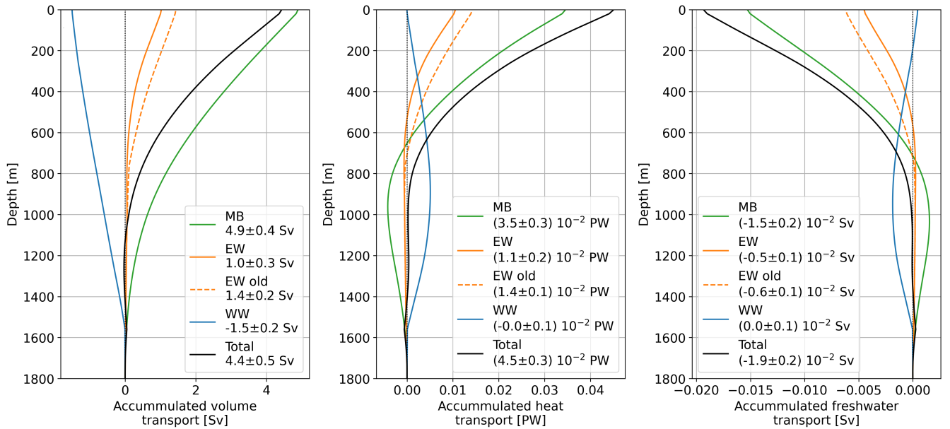
Figure 8. Depth-accumulated mean a) volume, b) heat and c) freshwater transports in the RT. Values are shown for the mid basin (MB) in green, the eastern wedge (EW) in orange (solid for the new, dashed for the old methodology), the western wedge (WW) in blue and the total transport in black.
