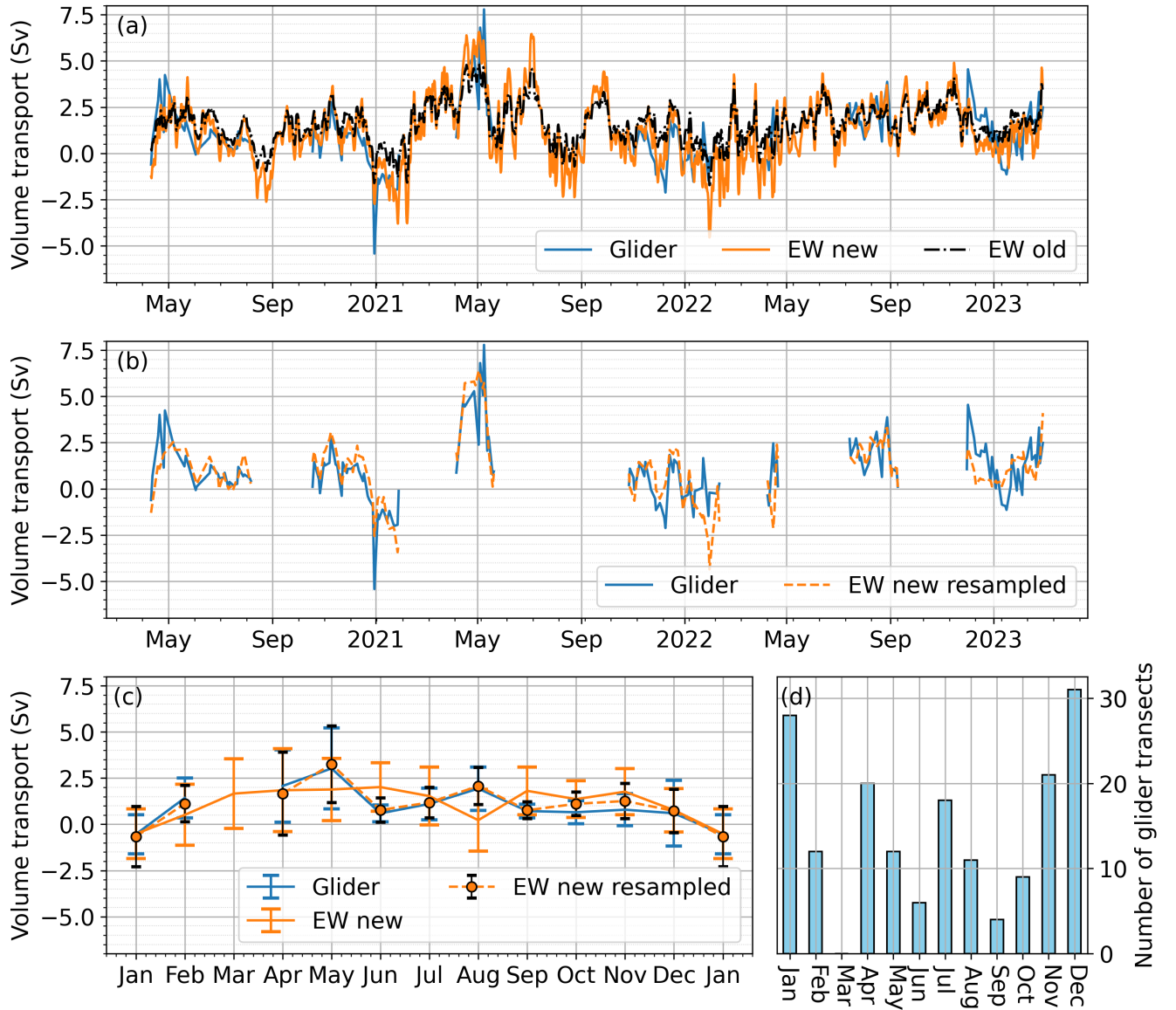
Figure 6. (a) Time series of volume transport for the upper 1000m derived from meridional velocity section based on glider transects (blue line), the new eastern wedge reconstruction (EW new, orange line), the old eastern wedge reconstruction (EW old, black dotted line). (b) Transport time series of the new approach averaged \pm 1 day on the time step of the glider observations (EW new resampled, orange dashed line). Glider transport are shown in blue again for reference. (c) Monthly mean seasonal cycle for glider (blue line), the new eastern wedge reconstruction (EW new, orange line) and the resampled new eastern wedge reconstruction (EW new resampled, orange dashed line). The error bars mark \pm 1 standard deviation. (d) Number of glider transects per month of the year.
