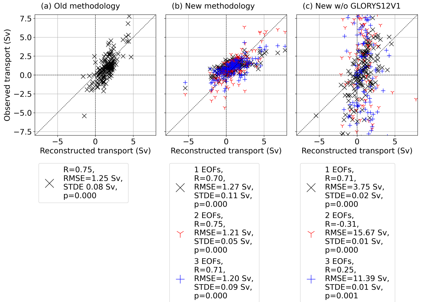
Figure 5. Linear regression of mooring-based reconstructions versus glider-derived transports. Panels show (a) the old methodology, (b) the new methodology using EB1 observations and GLORYS output at RTADCP, and (c) the new methodology using only EB1 observations. Statistics shown: R = Pearson correlation coefficient; RMSE = Root Mean Square Error; STDE = Standard Error; p = two-sided p-value for the null hypothesis that the slope equals zero.
