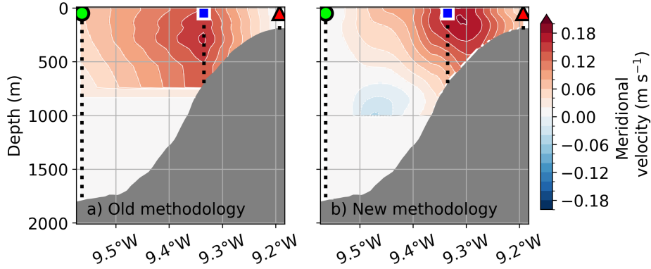
Figure 4. Averaged meridional velocity (2014-2024) for the eastern wedge using a) old methodology from Houpert et al. (2020) and Fraser et al. (2022) and b) the new methodology including glider observations. Black dotted line with green circle marks mooring EB1, black dotted line with blue square marks the position of the RTADCP, black dotted line with red triangle marks the eastern limit of the section. Please note that values below 1000m are near zero and therefore barely visible.
