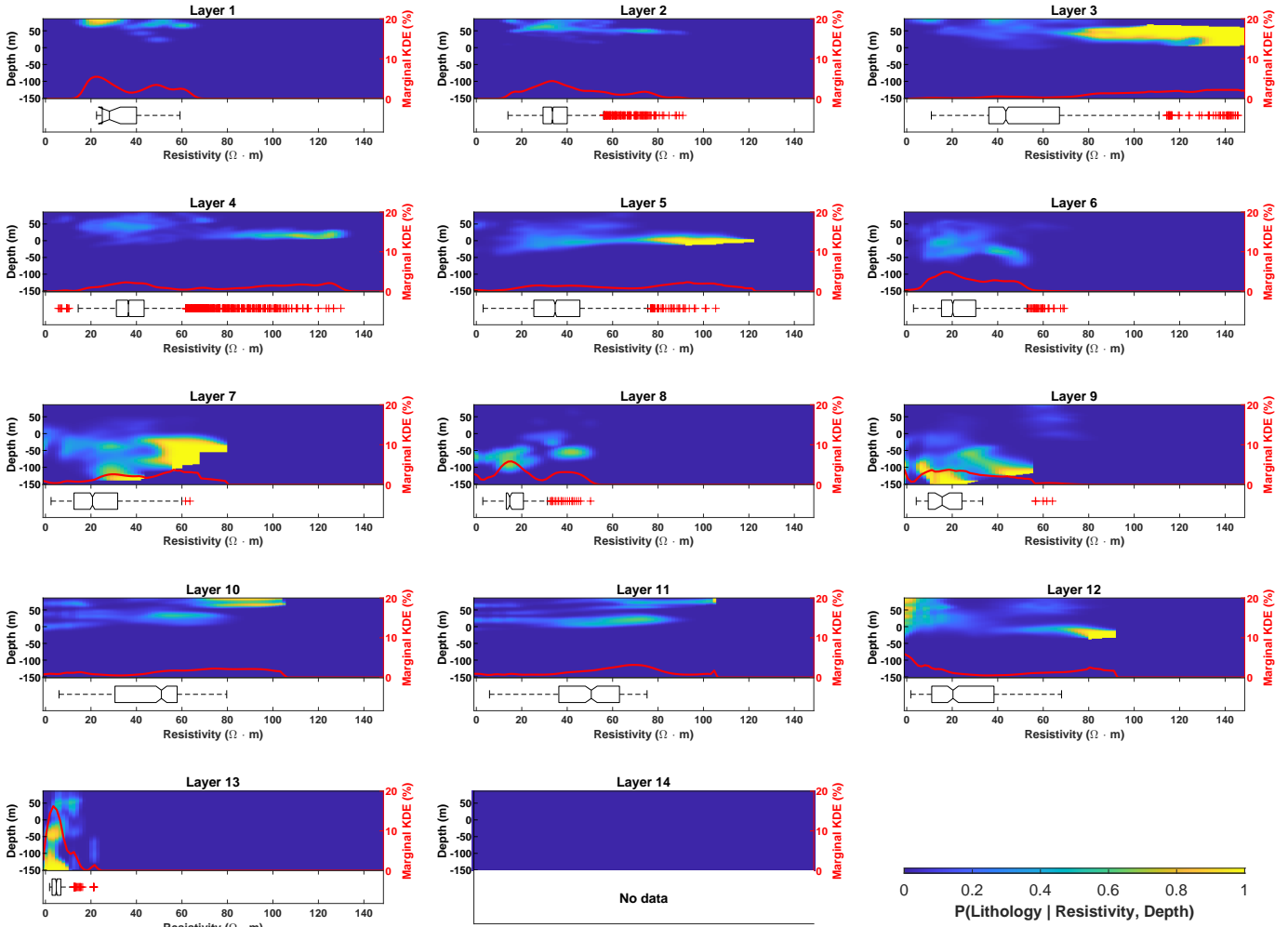
Figure 10. The heatmaps present the smoothed probabilistic distributions of each lithological layer estimated via KDE, conditioned on resistivity and depth. The red lineplot in each subplot represents the global normalized marginal probability of lithology conditioned solely on resistivity, derived from the KDE results. The boxplots below each heatmap display the distribution of resistivity values at each layer based on inverted geophysical data at borehole locations.
