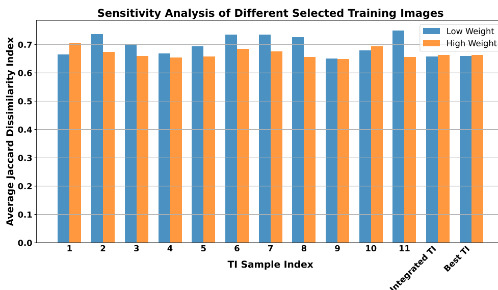
Figure 19. Sensitivity analysis of Training Image (TI) selection on lithological predictions using the MCP framework with geophysical constraints. The bar plot presents the average Jaccard dissimilarity index computed over 100 realizations for each of the 13 TI scenarios. These include 11 randomly selected TIs, one “Integrated TI” constructed from all 8 transects, and one “Best TI” using the current transect as the TI. Blue bars represent results under a low weight of geophysical constraint, while orange bars represent results under a high weight of geophysical constraint.
