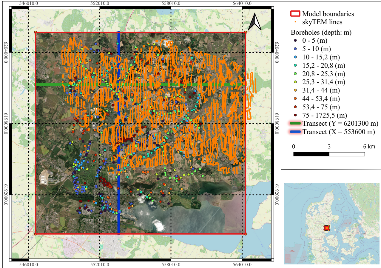
Figure 6. Distribution of boreholes and SkyTEM flight lines in the study area near Egebjerg, Denmark. The airborne electromagnetic data provide dense spatial coverage across the region in the central and northeastern parts. The red frame outlines the boundary of the previously established 3D model, which is used as a reference model for training image extraction. Borehole data are mostly shallow, with the majority of boreholes reaching depths of less than 50 meters. Two highlighted transects X = 553600 m and Y = 6201300 m were selected for detailed analysis. Both transects include segments with limited borehole data coverage.
