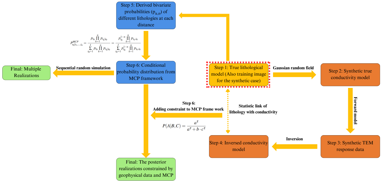
Figure 1. Workflow for the synthetic case
