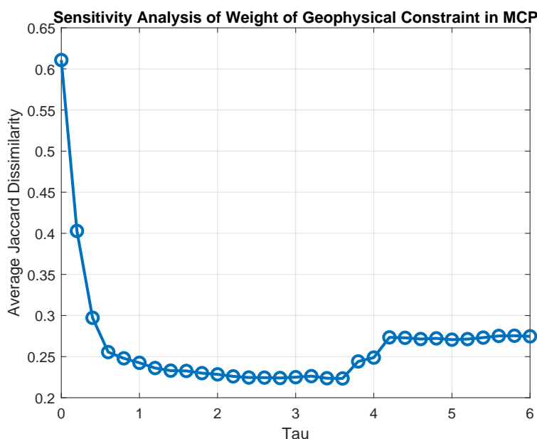
Figure 5. Sensitivity of weight of geophysical constraint in MCP via averaged Jaccard dissimilarity.
