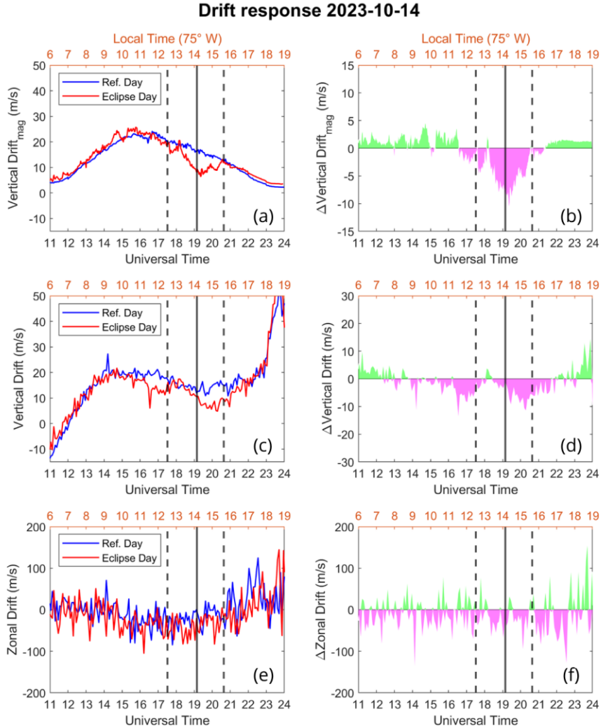
240 Figure 6: Vertical drift E \times B values (left) during the solar eclipse on 14 October 2023 and control day (12 October 2023). Differences between the eclipse day and the reference (right) are shown, where positive values are coloured green and negative values in magenta. Maximum obscuration (vertical black continuous line), eclipse onset and eclipse end (vertical black dashed line) are indicated.
