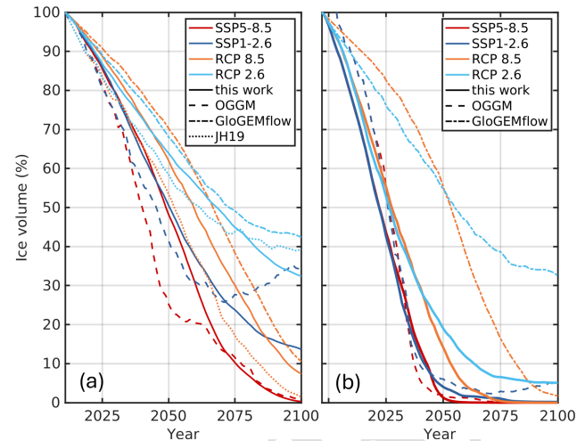
Figure 14. Comparison of glacier volume evolutions from previous studies for GAG (a) and HEF (b). Results of the large-scale models OGGM and GloGEMflow are from Schuster et al. (2023) and Zekollari et al. (2019), respectively. JH19 refers to the detailed full-Stokes study of GAG by Jouvet and Huss (2019). For each study, the ensemble medians are shown with the exception of GloGEMflow, for which the ensemble mean is presented. Note, that the projection start date of GloGEMflow is 2017 and we use a linear extrapolation to 1997.
