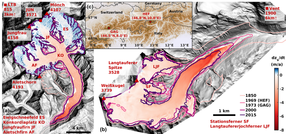
Figure 1. Map of Great Aletsch Glacier (GAG, a ) and Hintereisferner (HEF, b ) and their location in the European Alps ( c ). For GAG, mean annual elevation changes, \partial z_s/\partial t , are calculated from 2011 and 2019 digital elevation models (DEM, Leinss and Bernhard, 2021). For HEF, mean annual elevation changes are calculated from 2001 and 2013 DEMs (Sailer et al., 2017; Strasser et al., 2018). Prominent mountain summits are displayed with triangles and meteorological stations with squares. Note that the stations Lauterbrunnen (LTB) and Vent are outside the figure limits. Glacier outlines are taken from the Randolph Glacier Inventory (RGI v7.0) (RGI Consortium, 2023). The hillshade backgrounds are 2011 and 2001 DEMs for GAG and HEF, respectively.
