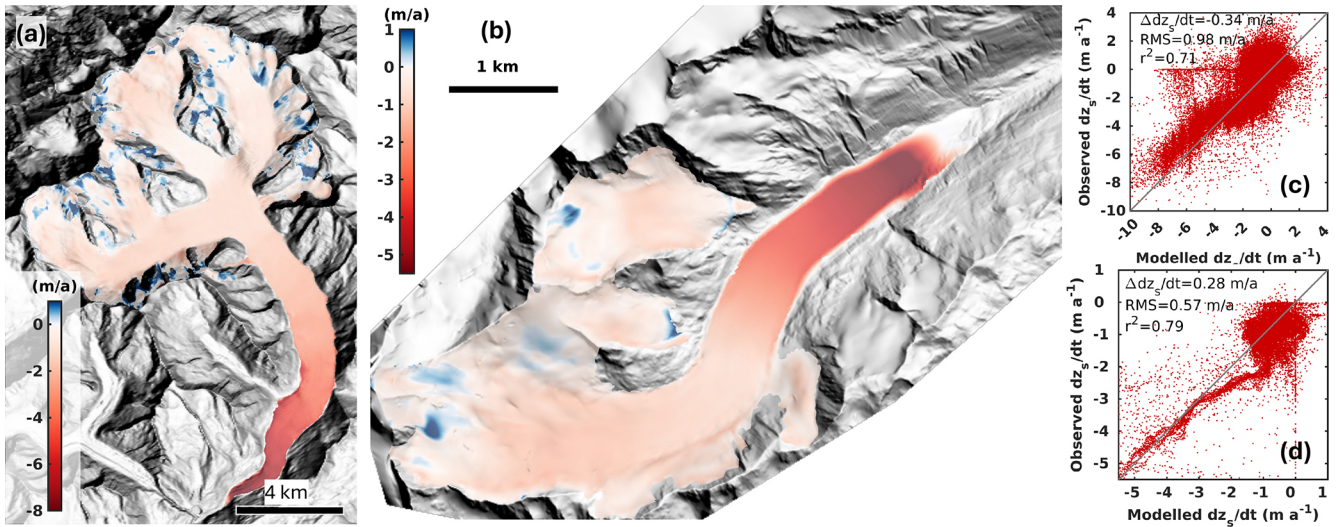
Figure 7. Modelled annual elevation change at GAG for the period 2011–2019 (a) and at HEF for the period 2001–2013 (b). The scatter plots show observed vs. modelled elevation change for GAG (c) and HEF (d).
