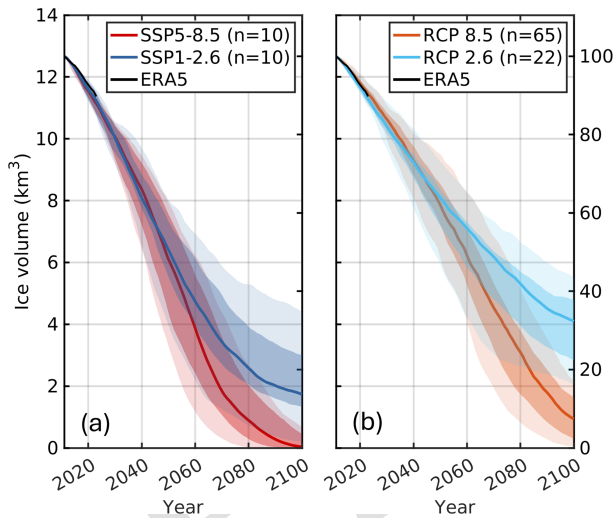
Figure 10. Glacier volume projections of GAG for CMIP6 scenarios SSP5-8.5 and SSP1-2.6 (a) and the CMIP5 scenarios RCP 8.5 and RCP 2.6 (b). Percentage values are relative to 2011. In addition an glacier volume projection based on the ERA5 reanalysis is shown to demonstrate the scenarios agreement over the past period (see Sect. 5.3). The ensemble median (thick lines), the 17th–83rd percentiles (dark shaded areas) and total range (light shaded areas) is shown.
