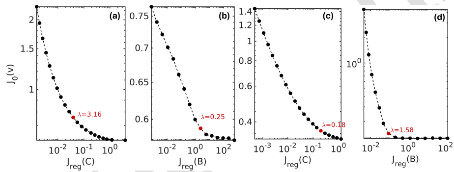
Figure A1. L-curves of the inversion for the basal friction coefficient ( a , c ) and the rheology B parameter ( b , d ) for HEF ( a , c ) and GAG ( b , d ). The selected regularization parameter \lambda of each inversion is highlighted in red.
