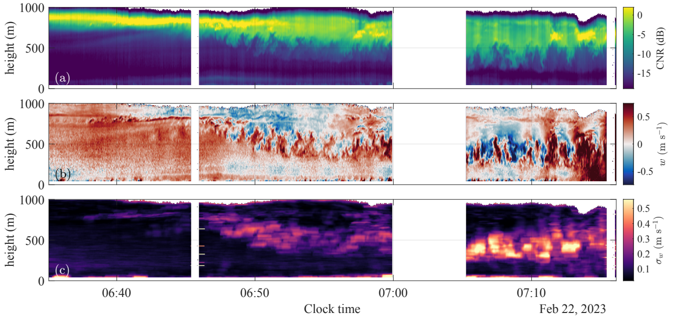
Figure 13. CNR (a), instantaneous vertical velocity component w (b), and estimated moving standard deviation, \sigma_w , of the component w (c) obtained using the WindCube100S on 22 February 2023 between 06:35 and 07:16 in the harbour.
