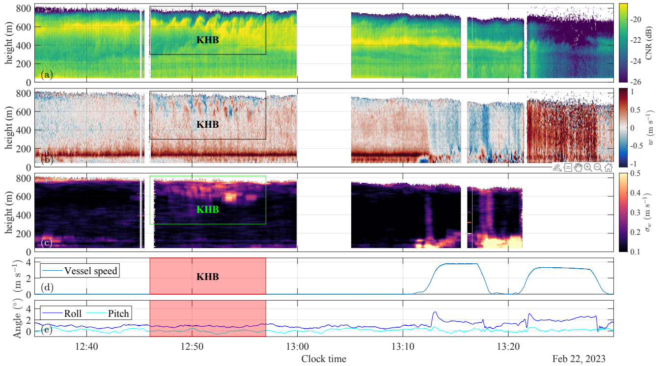
Figure 12. Time series of the Carrier-to-Noise ratio (CNR, a), instantaneous vertical velocity component w (b), and estimated moving standard deviation, \sigma_w , of the component w (c) obtained using the WindCube100S data in vertical stare mode from 12:35 to 13:30 on 2023-02-22. CTV absolute speed (d), roll and pitch angles (e) during the observational period.
