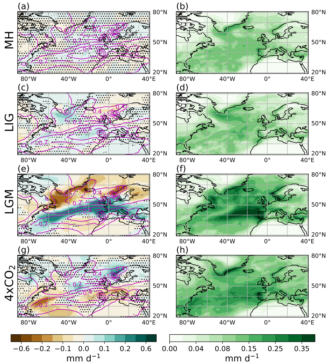
Figure 7. Same as Figure 6 but for multi-model mean change in DJF precipitation (mm d -1 ) associated with the NAO. Magenta contours show the pattern of the piControl . Stippling indicates where the ensemble is inconsistent in the direction of change.
