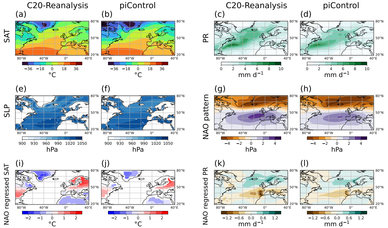
Figure 1. Comparison between observations taken from the 20th-Century Reanalysis (Compo et al., 2011) and the multi-model mean of the piControl simulations. Panels show DJF mean variables over the North Atlantic sector (see Section 2.3 for region definition). Panels present the (a, b) surface air temperatures in °C (SAT), (c, d) precipitation in mm d -1 (PR), (e, f) sea level pressure in hPa (SLP), (g, h) NAO pattern in hPa, and teleconnections between NAO and (i, j) SAT in °C and (k, l) PR in mm d -1 computed by regression against the NAO.
