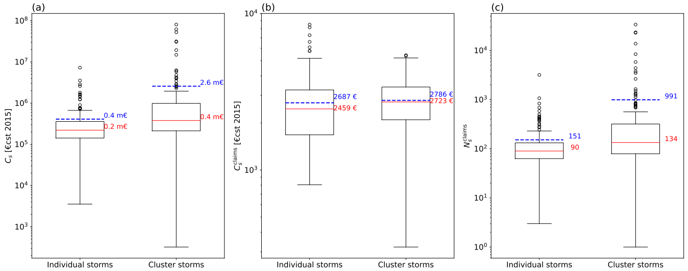
Figure 9. Distribution of the total cost per storm C_s in constant € 2015 (a), the mean cost per claim C_s^{claim} in constant € 2015 (b) and the number of claims per storm N_s^{claims} (c). Left bar plots show the statistics for the individual events and right ones for the storms being part of a cluster. Red solid lines indicate the median while blue dashed ones the mean.
