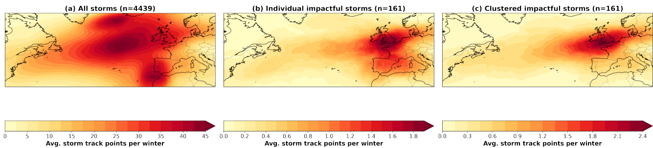
Figure C1. Distribution of storm tracks with an impact radius of 1300km for the set of all storms (a), isolated impactful storms resulting (b) and clustered impactful storms (c)
