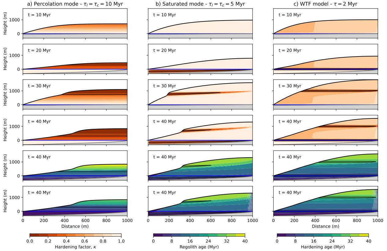
Figure 24. Comparison between three model experiments using a) the LAT model in the percolation mode, b) the LAT model in the saturated mode and c) the WTF model. In each column, the top 4 panels show the time evolution of the distribution of the hardening parameter, \kappa . The bottom two show the predicted regolith and hardening ages. The black line corresponds to the \kappa = \kappa_c contour. All model parameters are identical in the three experiments, including the uplift function made of two episodes of active uplift ( U = 100 m/Myr) of 10 Myr duration each followed by a period of tectonic quiescence. \tau_l = \tau_m = 5 Myr in the LAT experiments and \tau = 1 Myr in the WTF experiment.
