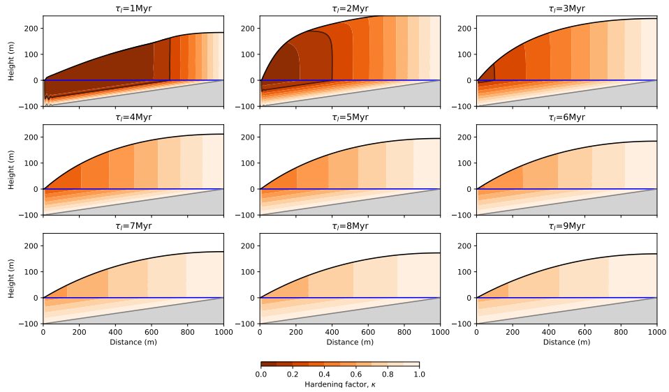
Figure S6. Model behavior with varying \tau , the laterisation time scale, in the saturated mode ( C = 0 ). Each panel corresponds to the model solution after 20 Myr of evolution with a different value of \tau increasing from top left to bottom right.
