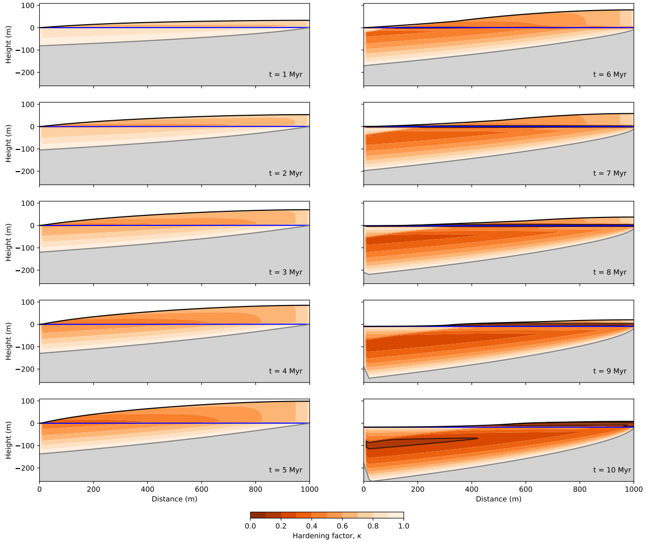
Figure S19. Evolution of a model experiment in which the LAT and WTF models have been combined. U = 30 m/Myr during the first half of the experiment and U = 0 m/Myr in the second half.
