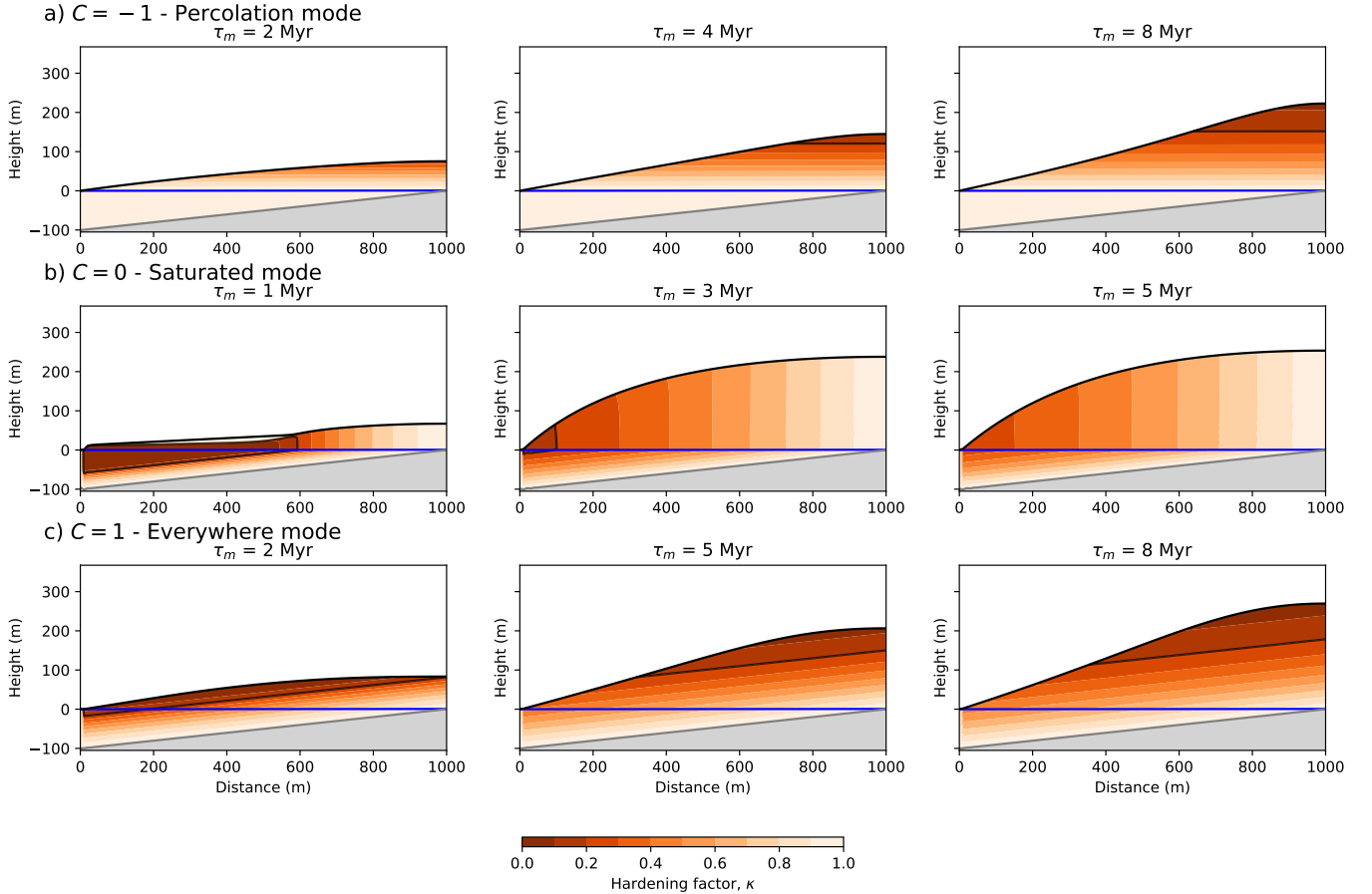
Figure 22. Model experiments in which we varied the mass loss time scale \tau_m while keeping all other parameter constant, including the laterisation time scale \tau_l at a value of 8 Myr. As indicated, each row of experiments corresponds to a different mode while each column to different values of \tau_m .
