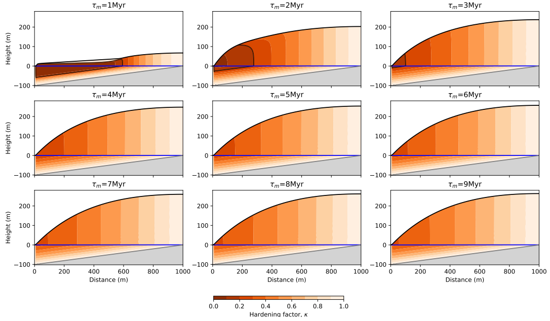
Figure S10. Model behavior with varying \tau_m , the mass loss time scale, in the saturated mode ( C = 0 ). Each panel corresponds to the model solution after 20 Myr of evolution.
