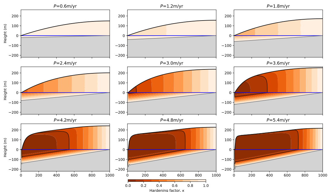
Figure S9. Model behavior with varying P , the precipitation or surface infiltration rate, in the saturated mode ( C = 0 ). Each panel corresponds to the model solution after 20 Myr of evolution.
