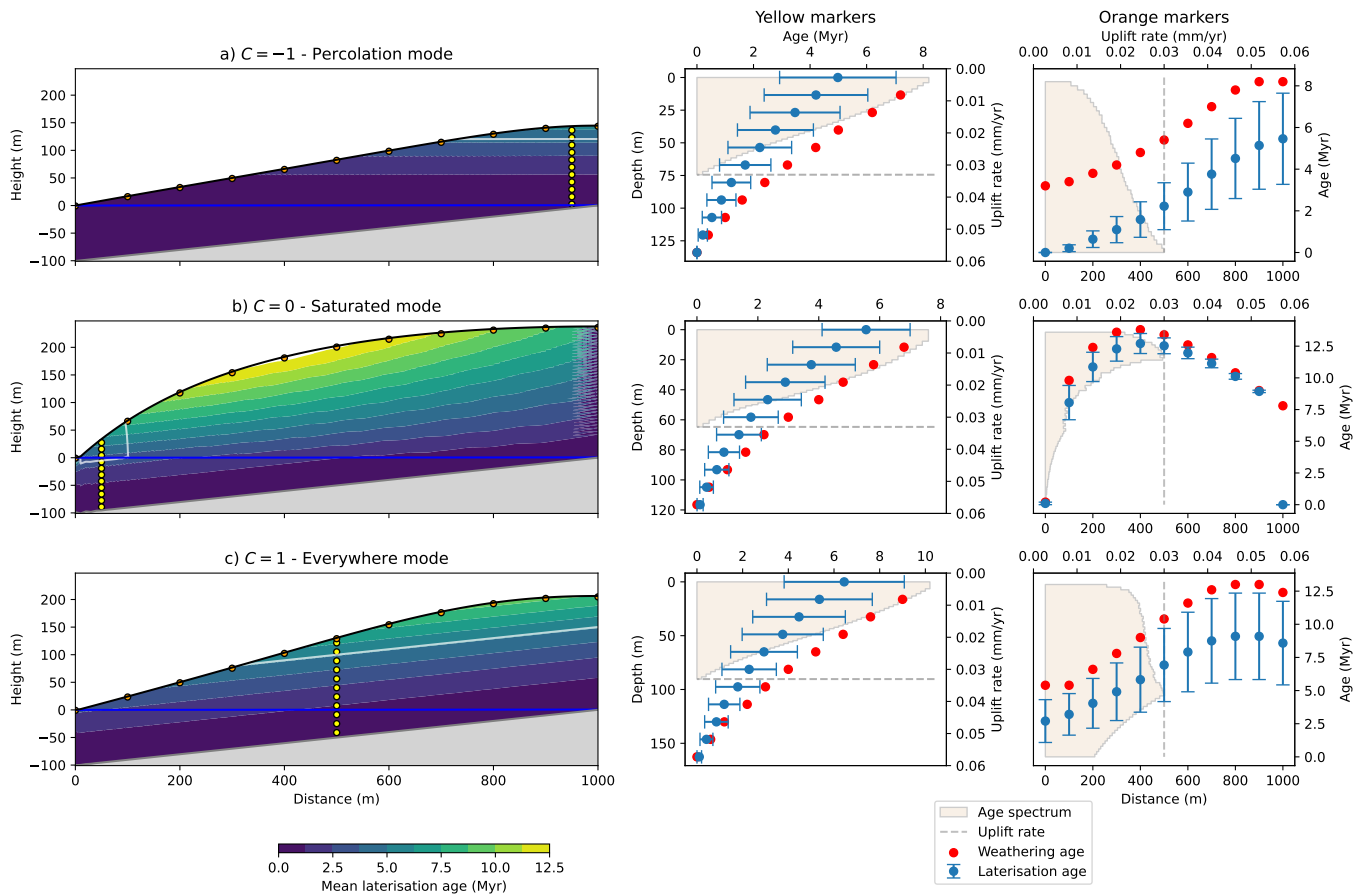
Figure 16. Contours of secondary weathering ages (left panels) for experiments in a) the percolation, b) the saturated and c) the everywhere modes. The white lines outline duricrusts. Central panels show distribution of mean and standard deviation in secondary weathering ages (blue circles) and primary weathering ages (red circles) along a vertical profile shown in the left panel. Beige shaded area is the computed distribution of ages for the entire profile. Right panel is similar to central panel but for points located along the surface of the model.
