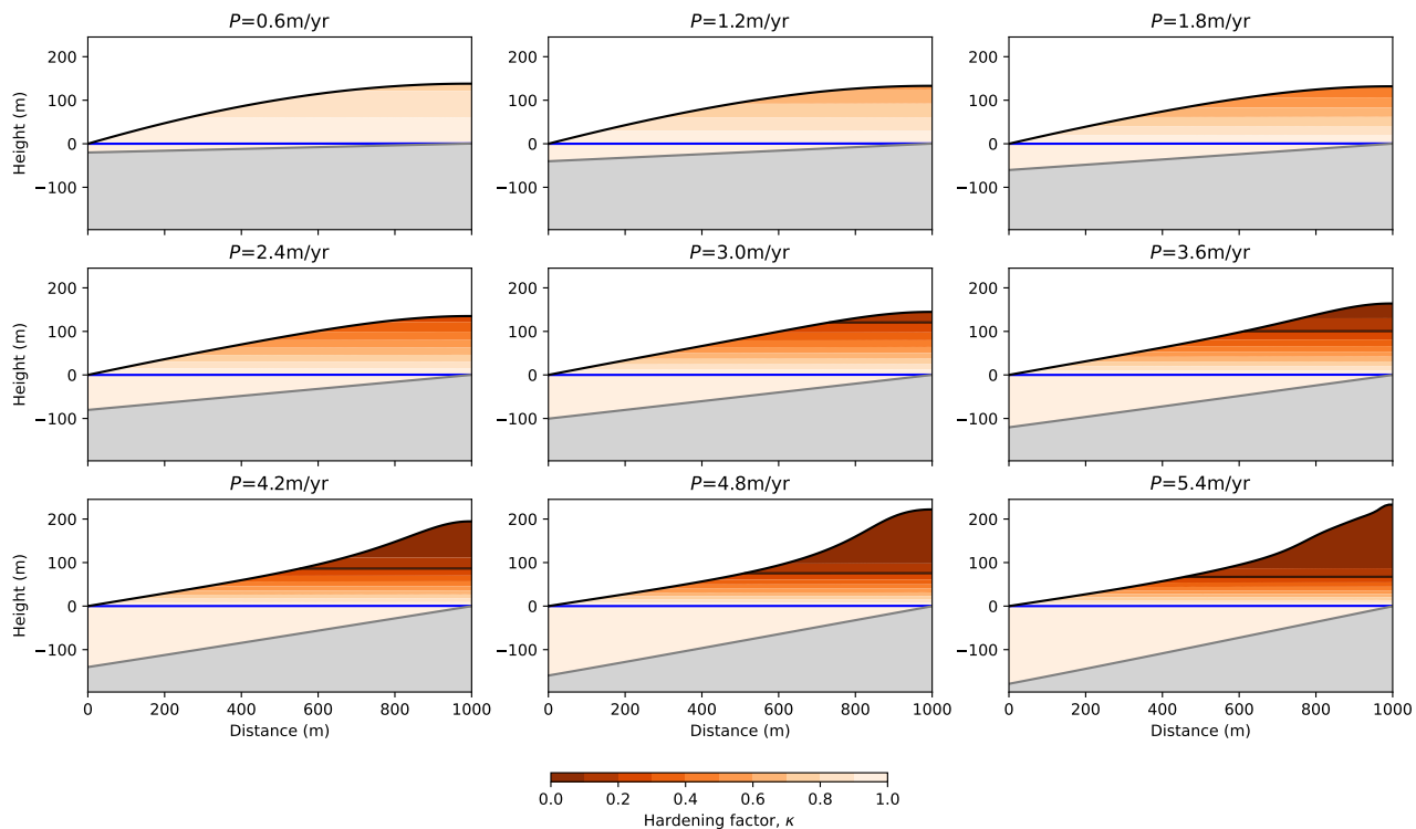
Figure S4. Model behavior with varying P , the precipitation or surface infiltration rate, in the percolation mode ( C = -1 ). Each panel corresponds to the model solution after 20 Myr of evolution.
