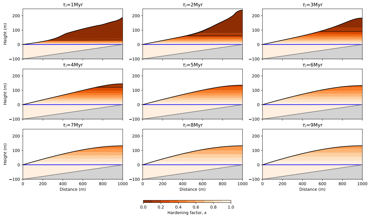
Figure S1. Model behavior with varying \tau , the laterisation time scale, in the percolation mode ( C = -1 ). Each panel corresponds to the model solution after 20 Myr of evolution with a different value of \tau increasing from top left to bottom right.
