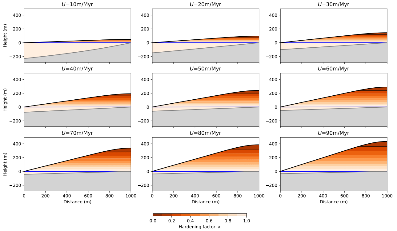
Figure S2. Model behavior with varying U , the uplift rate, in the percolation mode ( C = -1 ). Each panel corresponds to the model solution after 20 Myr of evolution with a different value of U increasing from top left to bottom right.
