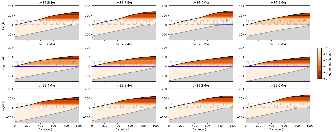
Figure 14. Varying the precipitation rate by introducing dry ( P = 0.5 m/yr) and wet periods ( P = 9.5 m/yr) of equal duration, 4 Myr. All model parameters are identical to those of the reference model in the percolation mode. The circle on the thin grey line shows the position of the corresponding panel with respect to the uplift cycles.
