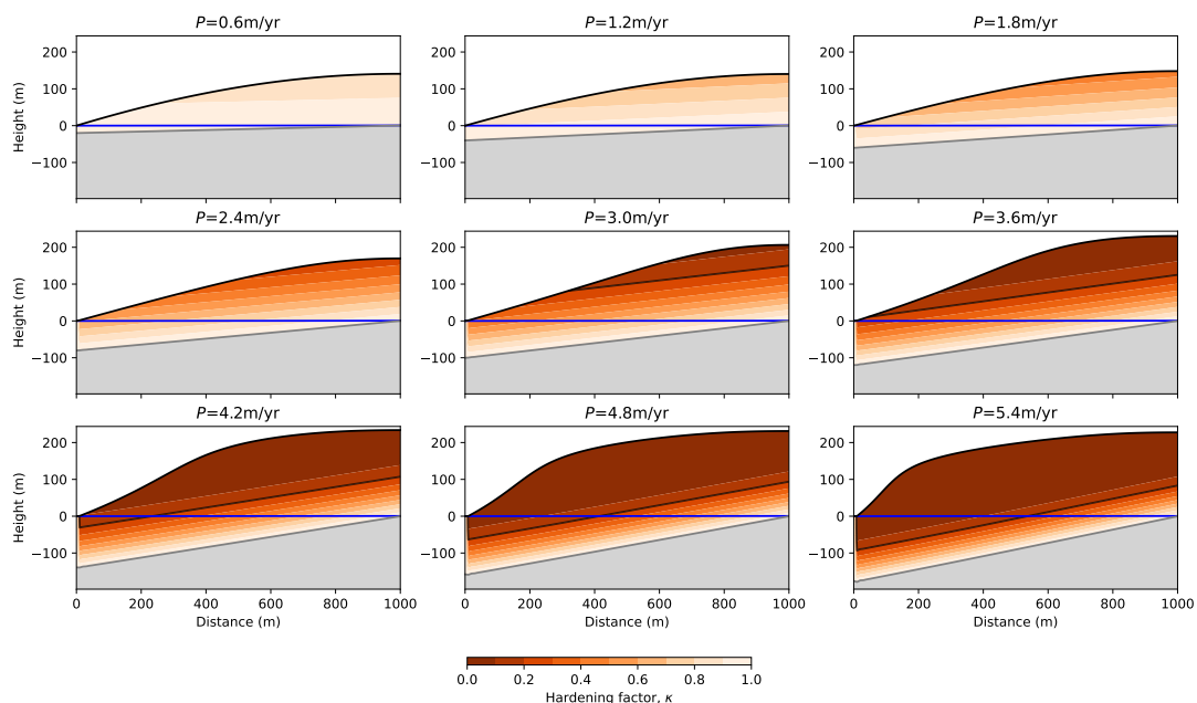
Figure S14. Model behavior with varying P , the precipitation or surface infiltration rate, in the everywhere mode ( C = 1 ). Each panel corresponds to the model solution after 20 Myr of evolution.
