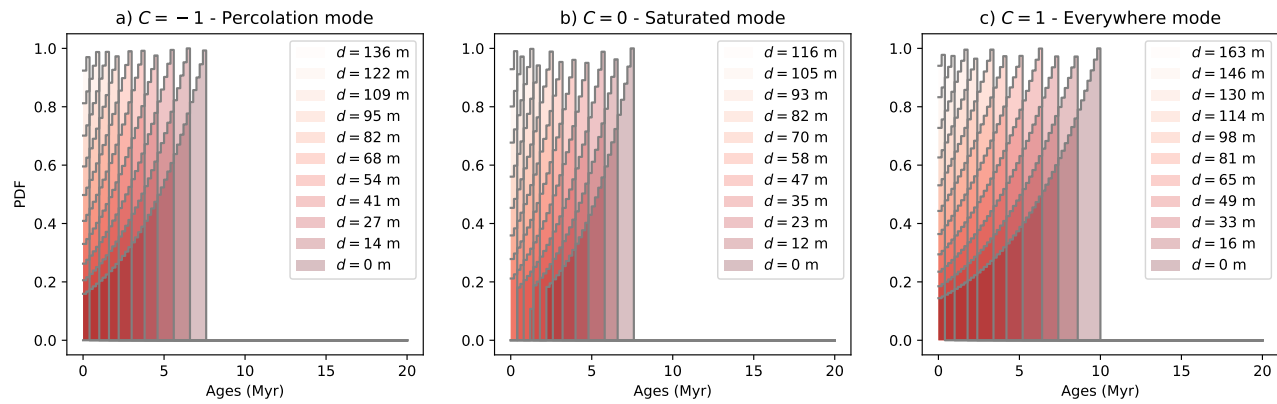
Figure S18. Computed age spectra along vertical profiles shown in Figure 16.
