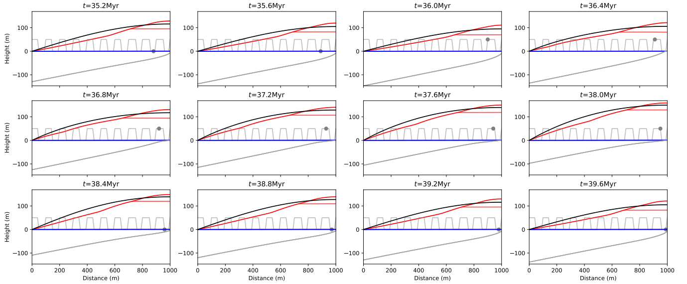
Figure 12. Comparison of contours for the percolation mode (in red) and a scenario without duricrust formation (in black). The water table (in blue) and weathering front (in gray) are the same for both scenarios. The variation uplift rate is the same as for the previous scenario. All model parameters are identical to those of the reference model in the percolation mode, apart for \tau in the scenario without duricrust formation, with \tau = 1.2e8 . The circle on the thin grey line shows the position of the corresponding panel with respect to the uplift cycles.
