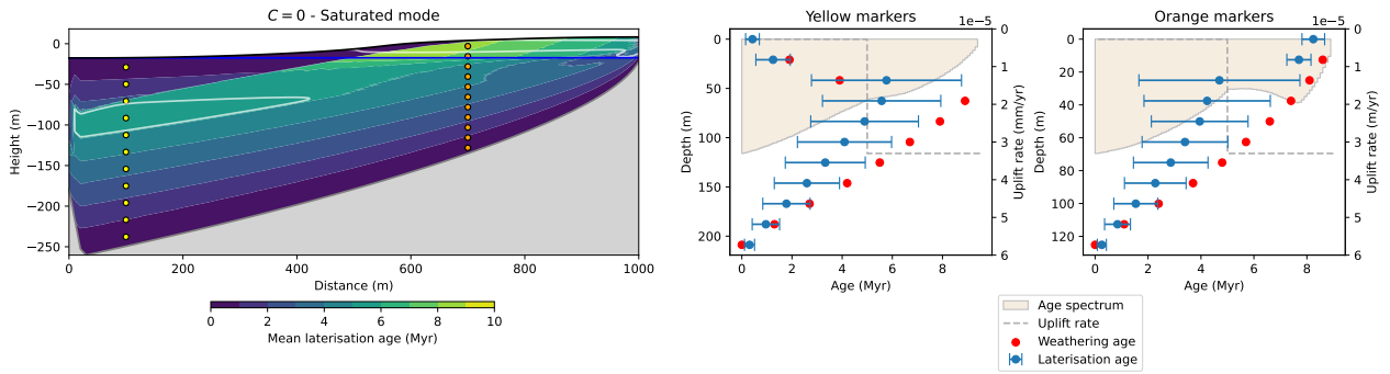
Figure 25. Predicted ages in a model experiment combining the LAT and WTF models. Areas within the white contours correspond to duricrusts ( \kappa < \kappa_c ).
