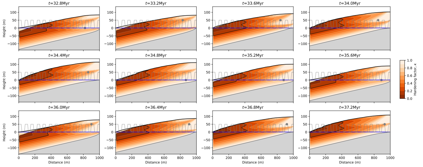
Figure 13. Varying the uplift rate by introducing periods of quiescence ( U = 0 ) and active uplift ( U = 60 m/Myr) of equal duration, 5 Myr. All model parameters are identical to those of the reference model in the saturated mode. The circle on the thin grey line shows the position of the corresponding panel with respect to the uplift cycles.
