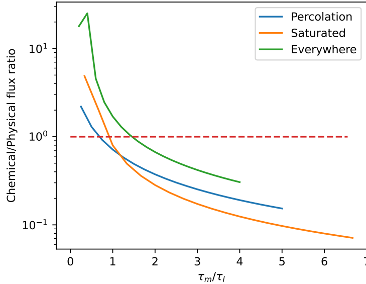
Figure 19. Computed ratio of chemical vs. physical fluxes (or erosion rate) as a function of the ratio of the mass loss time scale and the laterisation time scale. Values estimated at the end of a model run in which the time scale for laterisation, \tau_l , was chosen to lead to the formation of a thin duricrust (i.e. \tau_l = 4, 5 and 7 Myr in the percolation, saturated and everywhere modes, respectively).
