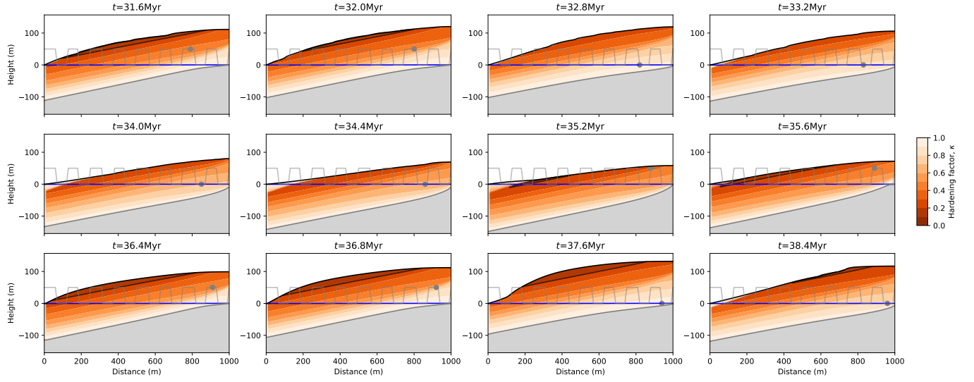
Figure S16. Varying the uplift rate by introducing periods of quiescence ( U = 0 ) and active uplift ( U = 50 m/Myr) of equal duration as in Figure 11 but with C = 1 , i.e., in everywhere mode.
