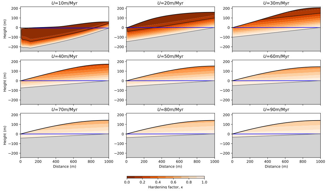
Figure S13. Model behavior with varying U , the uplift rate, and K_d , the surface transport coefficient in a constant ratio, in the everywhere mode ( C = -1 ). Each panel corresponds to the model solution after 20 Myr of evolution.
