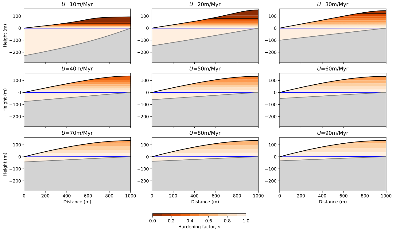
Figure S3. Model behavior with varying U , the uplift rate, and K_d , the surface transport coefficient in a constant ratio, in the percolation mode ( C = -1 ). Each panel corresponds to the model solution after 20 Myr of evolution.
