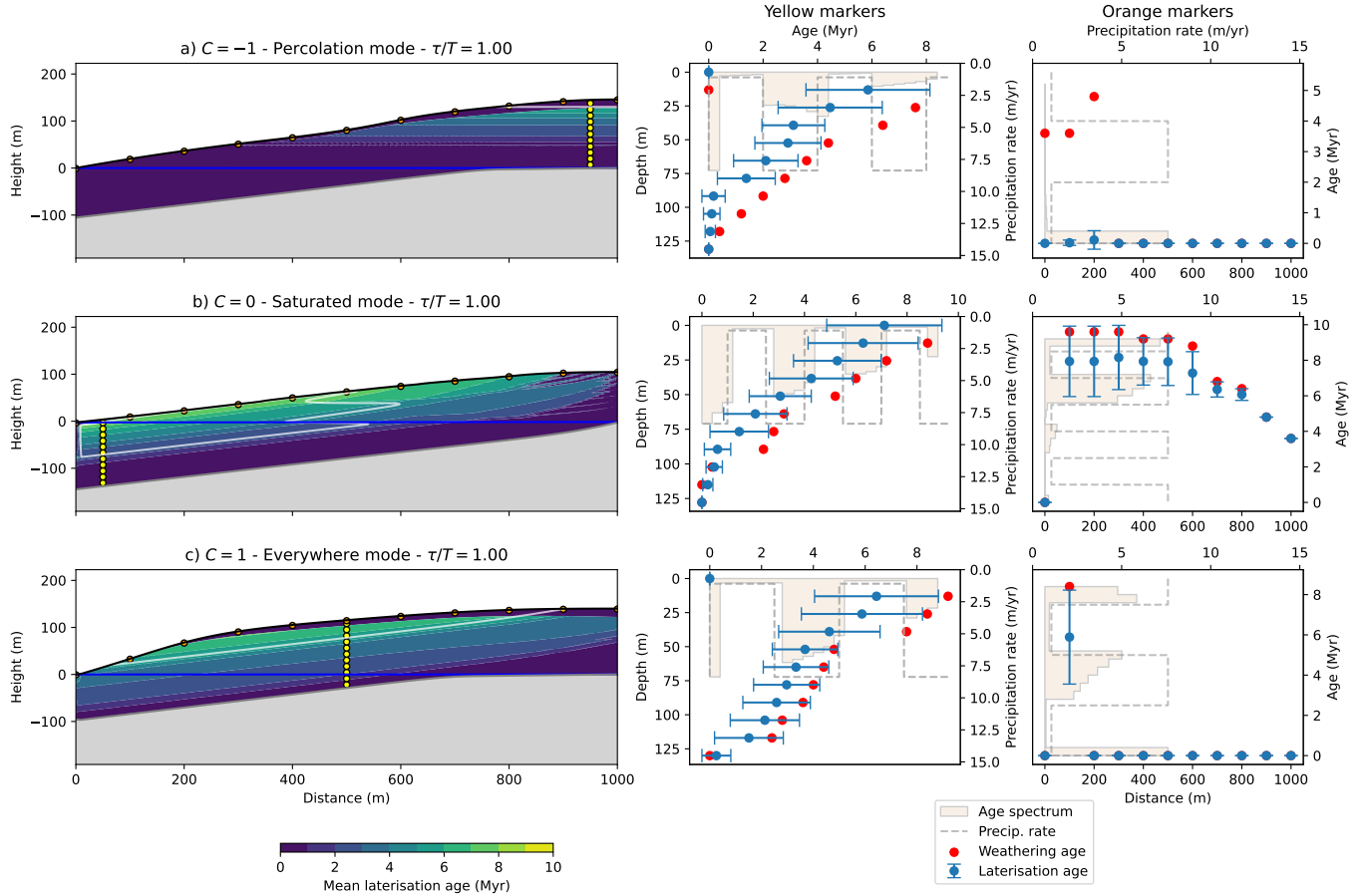
Figure 18. Age predictions for three model experiments with periodic variations in precipitation rate. See Figure 16 for detailed description of figure. The dashed lines in the central and right panels indicate the periods of enhanced precipitation rate. T is the period of the precipitation function.
