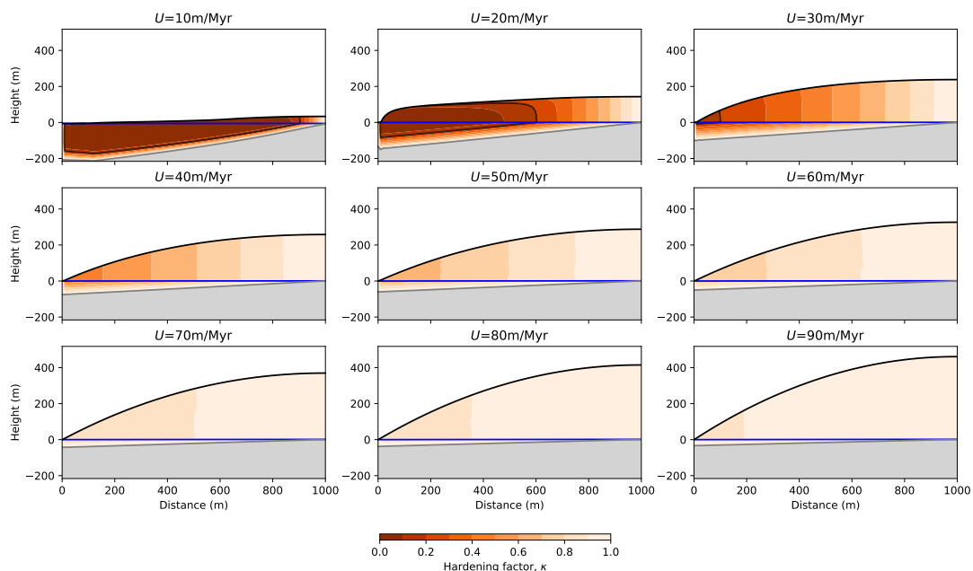
Figure S7. Model behavior with varying U , the uplift rate, in the saturated mode ( C = 0 ). Each panel corresponds to the model solution after 20 Myr of evolution with a different value of U increasing from top left to bottom right.
