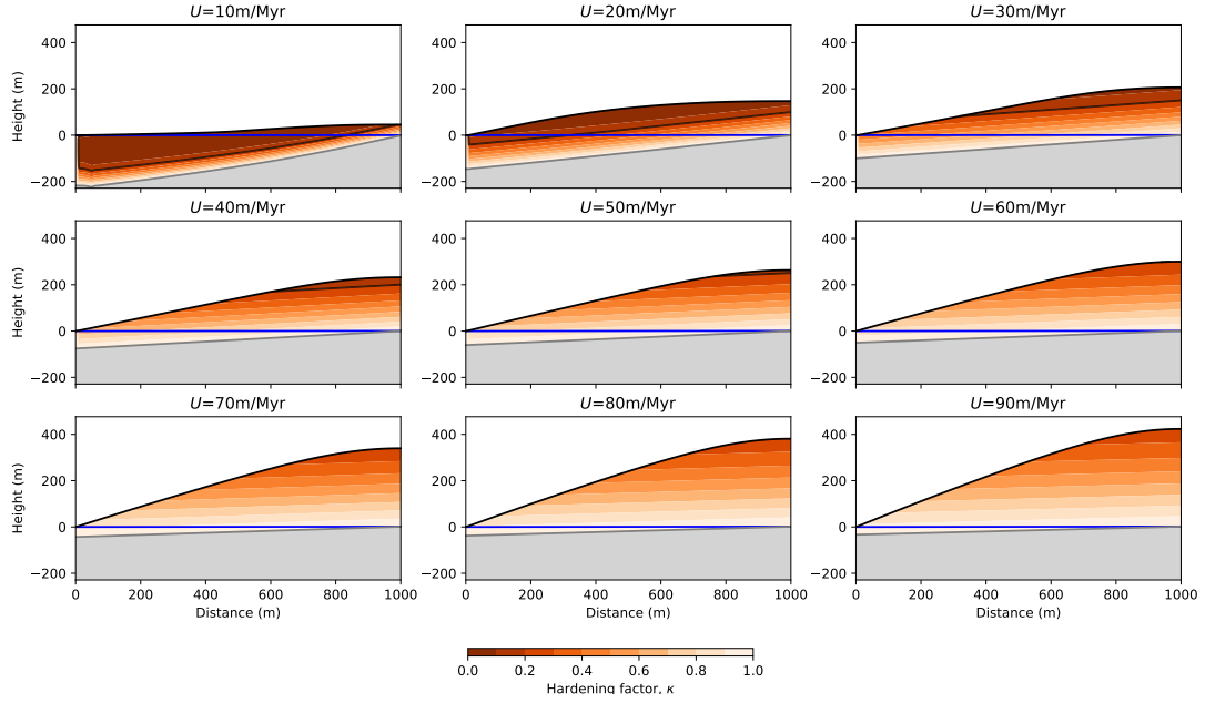
Figure S12. Model behavior with varying U , the uplift rate, in the everywhere mode ( C = 1 ). Each panel corresponds to the model solution after 20 Myr of evolution with a different value of U increasing from top left to bottom right.
