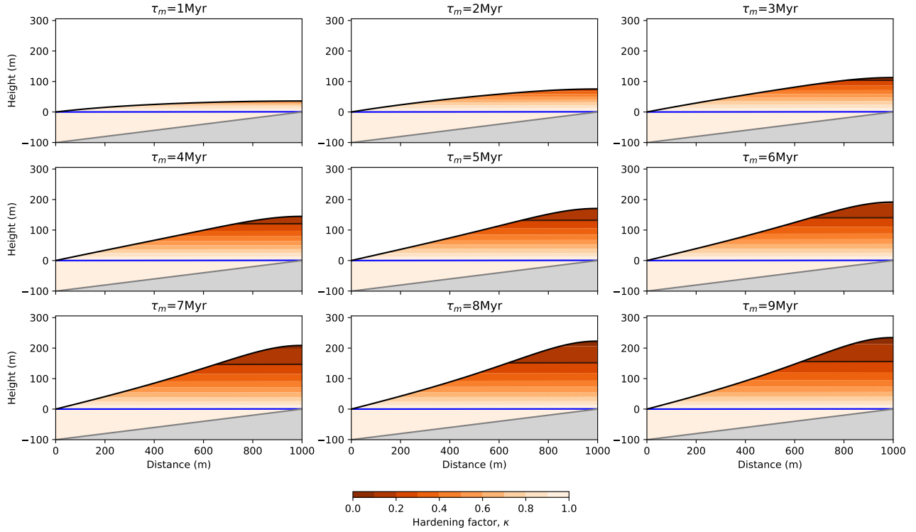
Figure S5. Model behavior with varying \tau_m , the mass loss time scale, in the percolation mode ( C = -1 ). Each panel corresponds to the model solution after 20 Myr of evolution.
