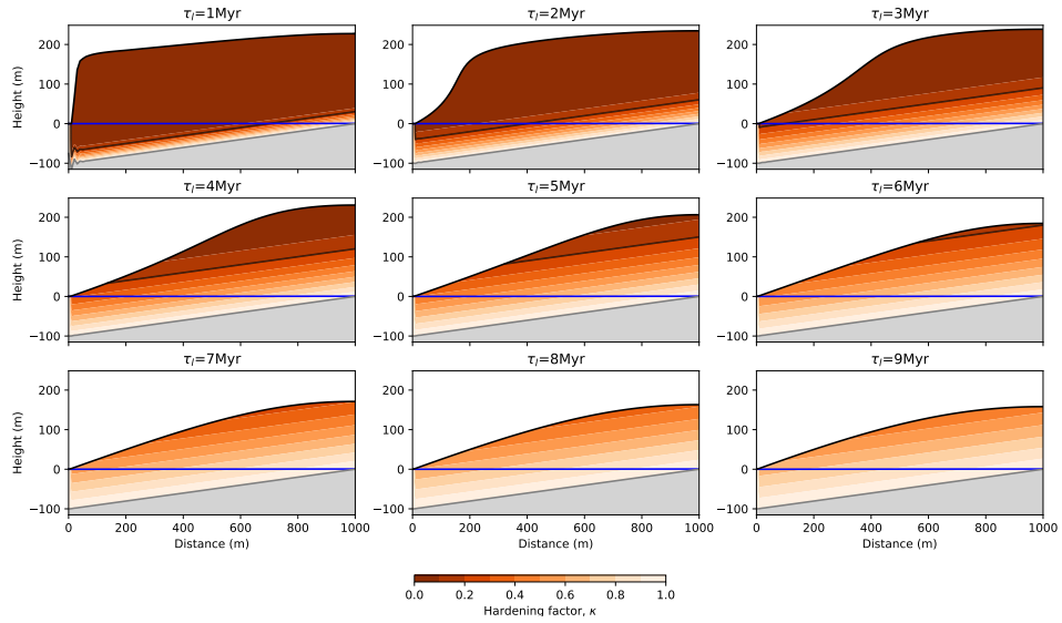
Figure S11. Model behavior with varying \tau , the laterisation time scale, in the everywhere mode ( C = 1 ). Each panel corresponds to the model solution after 20 Myr of evolution with a different value of \tau increasing from top left to bottom right.
