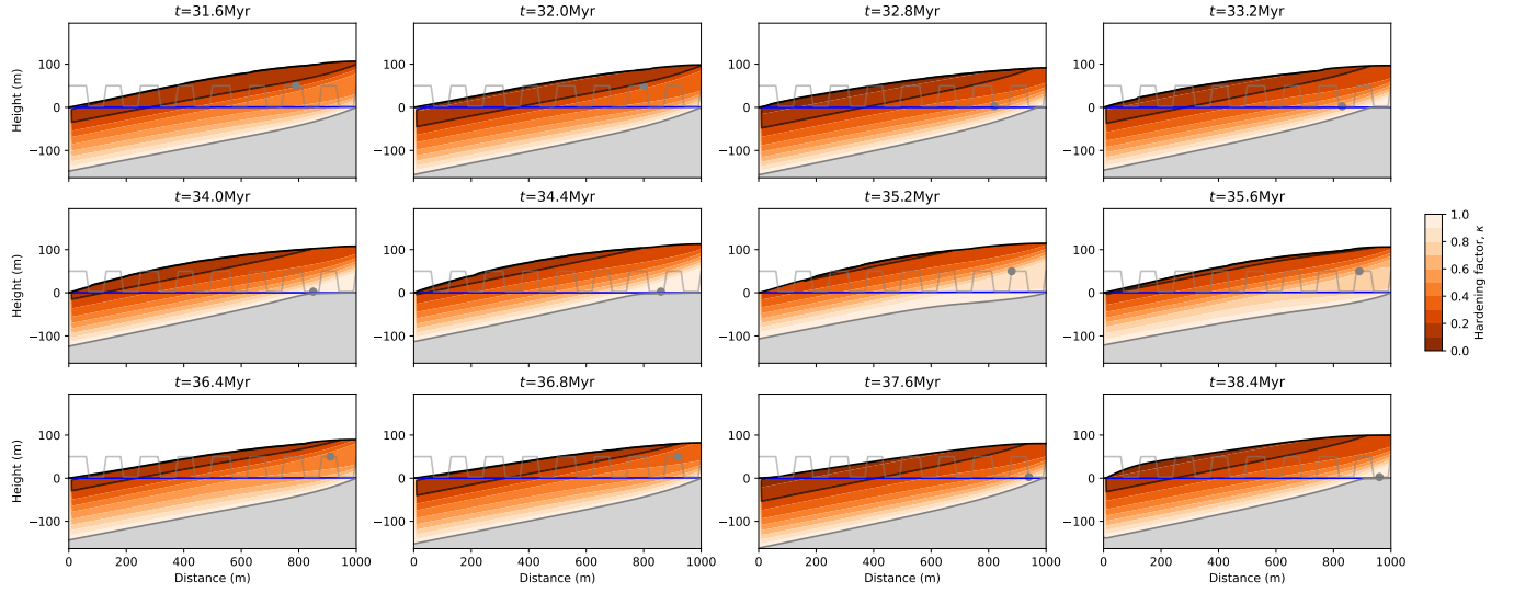
Figure S17. Varying the precipitation rate by introducing dry ( P = 0.5 m/yr) and wet ( P = 7.5 m/yr) periods of equal duration as in Figure 14 but with C = 1 , i.e., in everywhere mode.
