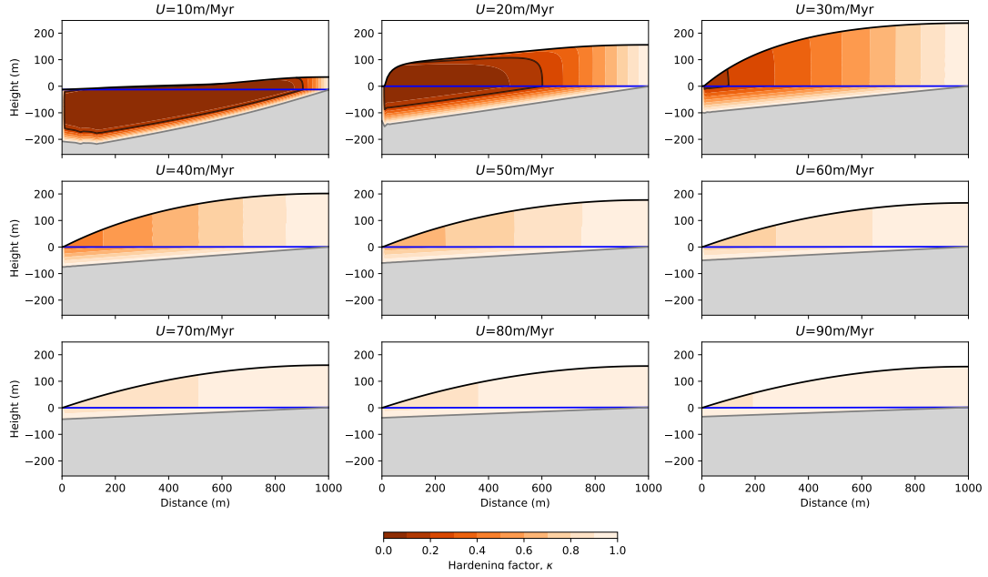
Figure S8. Model behavior with varying U , the uplift rate, and K_d , the surface transport coefficient in a constant ratio, in the saturated mode ( C = 0 ). Each panel corresponds to the model solution after 20 Myr of evolution.
