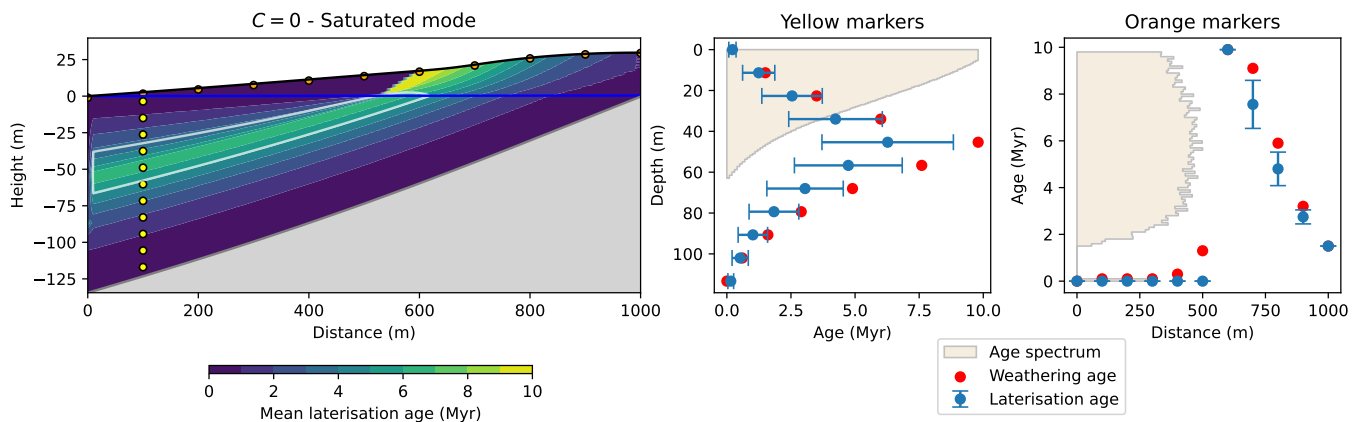
Figure 23. Contours of secondary weathering ages (left panels) for an experiment in the saturated mode and a mass loss time scale ( \tau_m = 2 Myr) smaller than the laterisation time scale ( \tau_l = 5 Myr). Uplift rate is set to 20 m/Myr to enhance the effect of duricrust burial by sedimentation. Age distributions along a vertical profile and the surface of the model are shown in the central and right panels.
