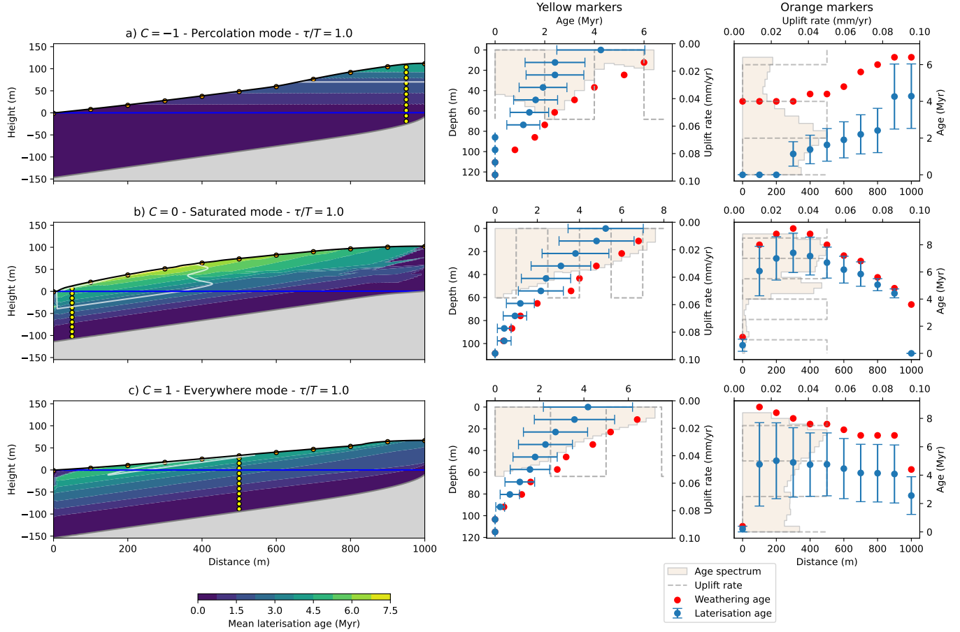
Figure 17. Age predictions for three model experiments with periodic variations in uplift rate. See Figure 16 for detailed description of figure. The dashed lines in the central and right panels indicate the periods of active uplift. T is the period of the uplift function.
