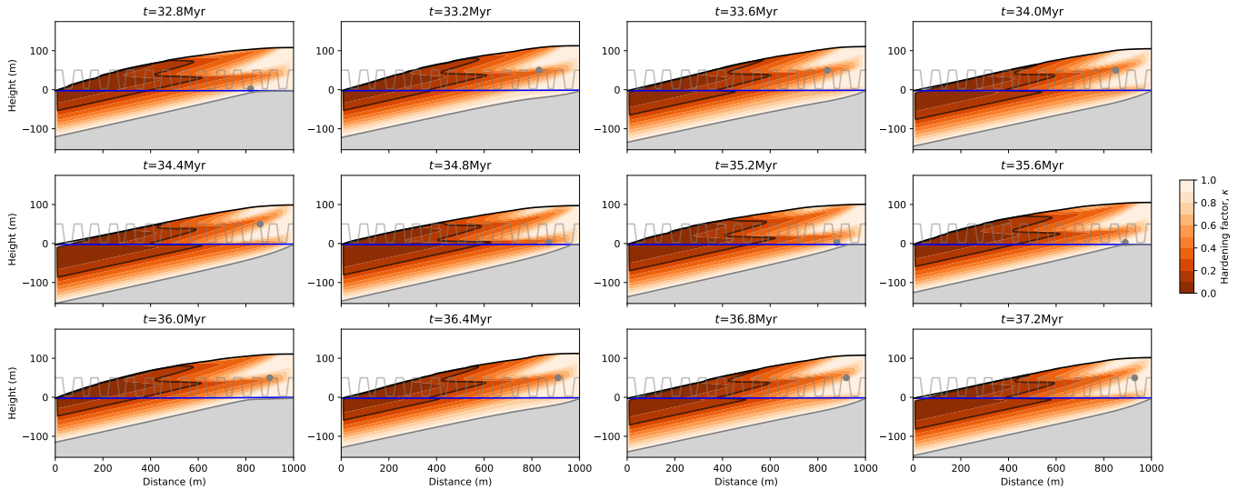
Figure 15. Varying the precipitation rate by introducing dry ( P = 0.5 m/yr) and wet periods ( P = 9.5 m/yr) of equal duration, 5 Myr. All model parameters are identical to those of the reference model in the saturated mode. The circle on the thin grey line shows the position of the corresponding panel with respect to the uplift cycles.
