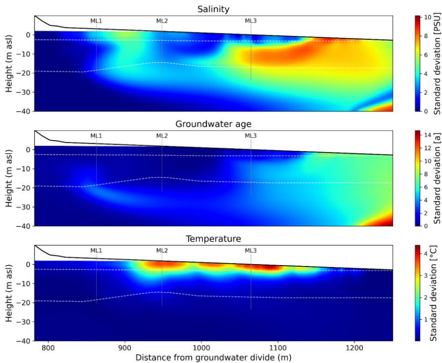
470 Figure 6: Standard deviation of simulated salinity, groundwater age and temperature time series along the modelled cross-section between July 2016 and February 2024.
