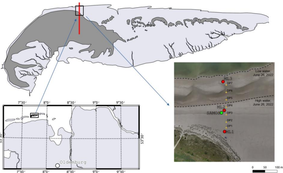
125 Figure 1: Location of the instrumented field site on Spiekeroog Island. The red line indicates the model transect. Dark grey area on the island highlight dune areas. The red circles indicate the positions of the multi-level groundwater monitoring wells ML1, ML2 and ML3. The green circle represents the geophysical saltwater monitoring system SAMOS. The yellow circles indicate the positions of the Direct-Push (DP) sampling points. The aerial picture is from a drone-survey on June 26, 2022. The maps were adapted from Massmann et al. (2023) under the open access Creative Commons Attribution License (CC BY).
