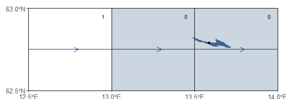
Figure 3. Catchment-lake scheme for lake 12247 ( A_{lake} = 22.46 \text{ km}^2 , A_{catchment} = 1662 \text{ km}^2 , A_{grid} = 1415 \text{ km}^2 and N = 1 ). The dot denotes the lake centroid, respectively. The arrows indicate the flow direction, and the numbers indicate the grid cell levels. The blue-shaded grid cells represent those selected for the streamflow estimation, according to the workflow (Figure 2).
