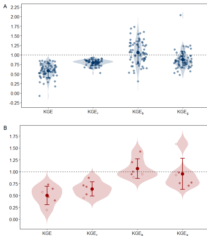
Figure 6. Kling-Gupta efficiency ( KGE ) and its components, timing ( KGE_r ), bias ( KGE_b ) and variability ( KGE_g ), when comparing monthly simulations of scaled streamflow with reference data from the HYPE model (A) and observed data (B) of streamflow. Filled dots correspond to study sites where A_{lake} \leq A_{grid} (approach I) and unfilled dots corresponds to study sites where A_{lake} > A_{grid} (approach II). The horizontal dashed line marks where KGE and its components equal 1, representing a perfect match
