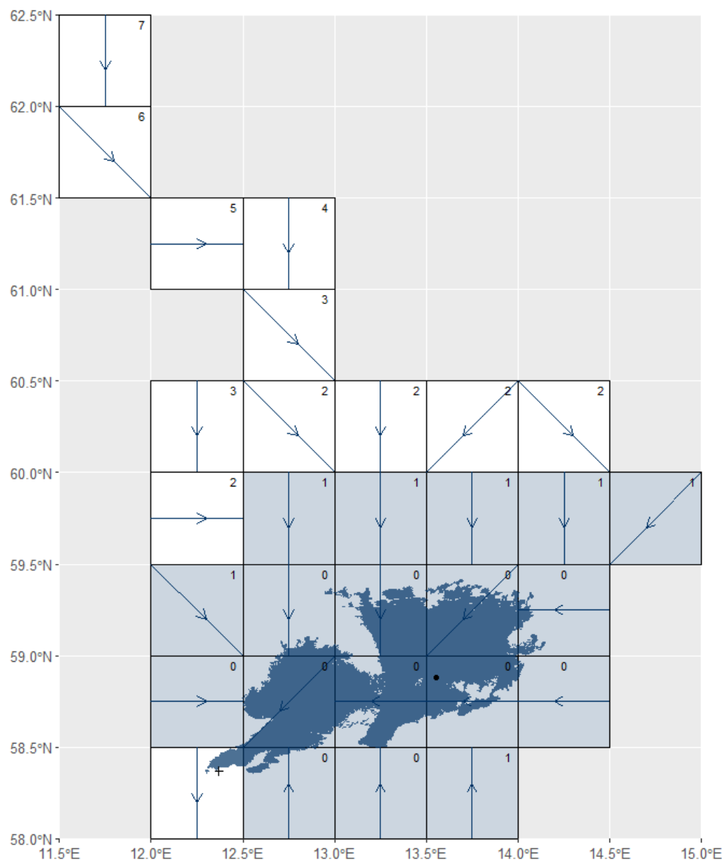
Figure 5. Catchment-lake scheme for lake Vänern – 105 ( A_{lake} = 5486 \text{ km}^2 , A_{catchment} = 48421 \text{ km}^2 and A_{grid} = 1604 \text{ km}^2 ). The dot and cross denote the lake centroid and the pour point, respectively. The arrows indicate the flow direction, and the numbers indicate the grid cell levels. The blue-shaded grid cells represent those selected for the streamflow estimation, according to the workflow (Figure 2).
