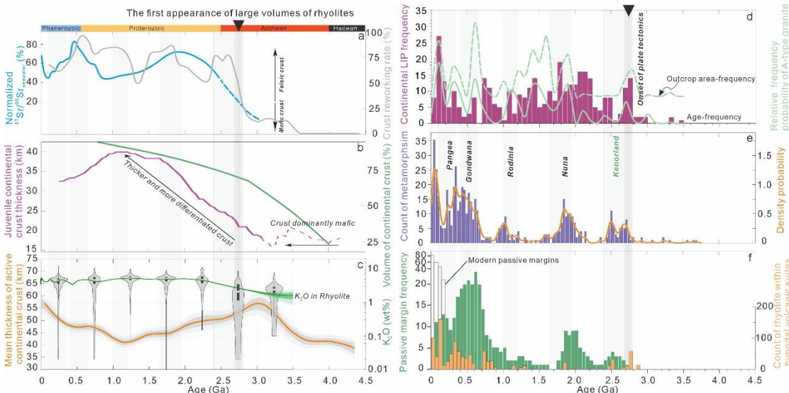
Figure 45: Secular changes of (a) Normalized seawater ^{87}Sr/^{86}Sr curve (Shields, 2007) and the degree of reworking of the continental crust (Dhuime et al., 2012); (b) Continental growth curve (Dhuime et al., 2012) and thickness of juvenile continental crust (Dhuime et al., 2015); (c) K_2O in global rhyolites and mean thickness of active continental crust (Tang et al., 2021); (d) the numbers of continental large igneous provinces (LIPs) (Ernst et al., 2021), and the relative age/outcrop area-frequency probability of A-type granites (Condie et al., 2023) through Earth's history; (e) Ages and probability density function for global metamorphism (Brown and Johnson, 2019b); and (f) the distributions of passive margins and the count of rhyolites within bimodal volcanics (Bradley, 2008). Note the convergence of multiple proxies (rhyolite K_2O , crustal reworking, metamorphic peaks, etc.) within the 2.7 Ga transition window.
