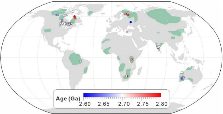
135 Figure 3: The distributions of ~2.7±0.1 Ga rhyolites on Earth. The filled circles represent the location of rhyolite samples. The light green filled areas cover the scope of global cratons. We should note that the significant amount of rhyolite around 2700 million years ago, is not confined to any particular region but instead scattered across ancient cratons.
