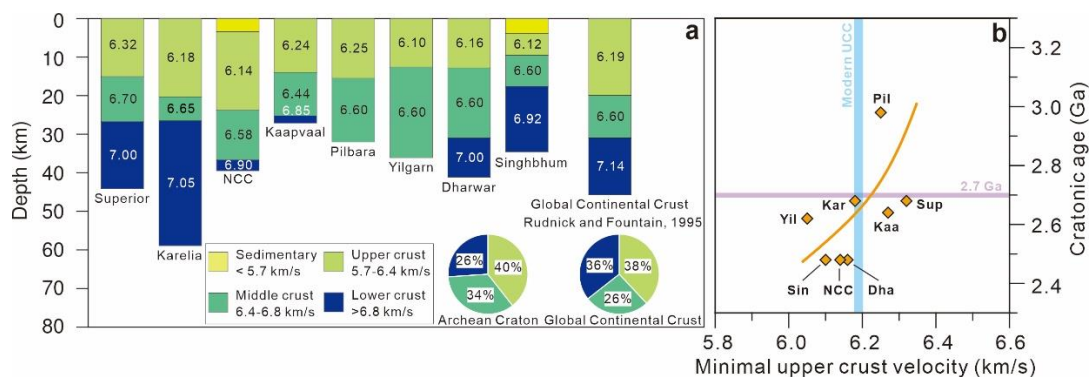
Figure 4: The velocity structure of Archean cratons and global continental crust. (a) Representative cratons' velocity structure (Musacchio et al., 2004; Kuusisto et al., 2006; Xia et al., 2017; Durrheim and Green, 1992; Drummond and Collins, 1986; Drummond, 1988; Vijaya Rao et al., 2015; Kaila and Sain, 1997) and global continental crust velocity structure (Rudnick and Fountain, 1995). (b) Minimal upper crust velocity versus cratonic age, with the fitting curve marked by orange solid line. The light blue line shows the average velocity of modern upper crust (UCC). Abbreviation: Sup: Superior, Kar: Karelia, NCC: North China Craton, Kaa: Kaapvaal, Pil: Pilbara, Yil: Yilgarn, Dha: Dharwar, Sin: Singhbhum.
