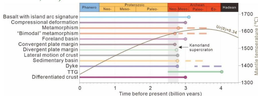
Figure 1: The beginning ages (circles) and age ranges (solid and dashed lines) of proposed major geological archives for plate tectonics. The solid lines correspond to the widespread and continual presence of these geological archives, whereas the dashed lines indicate sporadic occurrences of such geological events. Three ingredients are crucial to understanding the onset of plate subduction: (1) a rigid and more differentiated continental crust; (2) mutual movements of plates; (3) geological evidence for plate margin interaction. The beginning ages and age ranges for a possible rigid continental lithosphere are represented by differentiated crust (Dhuime et al., 2015), tonalite-trondhjemite-granodiorite series (TTGs) (Bowring and Williams, 1999; Moya and Martin, 2012), giant vertical dyke (Ernst et al., 2021) and sedimentary basins (Siahi et al., 2016; Srinivasan and Ojakngas, 1986; Wingate, 1999). The initiation of lithospheric mobility of continents is constrained by paleomagnetic evidence (Cawood et al., 2018). The geological evidence for plate margin interaction can be indicated by the occurrence of divergent (Bradley, 2008; Cawood et al., 2018) and convergent plate margins (Condie, 2021), foreland basin (Burke et al., 1986; Catuneanu, 2001; Corcoran and Mueller, 2007), paired
