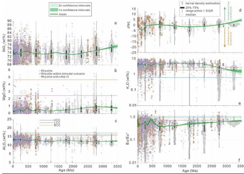
Figure 2: The features of (a)SiO 2 ; (b) MgO; (c) Al 2 O 3 , (d) initial neodymium isotopes (εNd), (e) K 2 O and (f) Eu/Eu* of rhyolites through time. The compositions of present-day continental crust are adapted from (Rudnick and Gao, 2003). 350-Myr-bin moving average of rhyolite compositions together with the 1σ and 2σ confidence intervals acquired by bootstrap resampling (numbers=1000) are shown. The kernel density estimations, medians, inter-quartile range (IQR, 25%–75%) and range within 1.5IQR of each 500-Myr-bin are also shown for all data without rejection. UCC=upper continental crust; LCC=lower continental crust; BCC=bulk continental crust.
