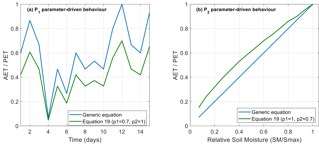
430 Figure 9. Comparison of equation evap_19 with a typical evapotranspiration formulation (here the generic equation is represented as evap_19 where p_1 and p_2 equal 1). (a) p_1 parameter-driven behaviour: Time series of AET/PET over 15 days, illustrating how evap_19 constrains AET to remain below PET. (b) p_2 parameter-driven behaviour: Relationship between relative soil moisture ( SM/S_{max} ) and AET/PET, showing the stronger non-linear response of AET equation evap_19 to changes in soil moisture availability.
