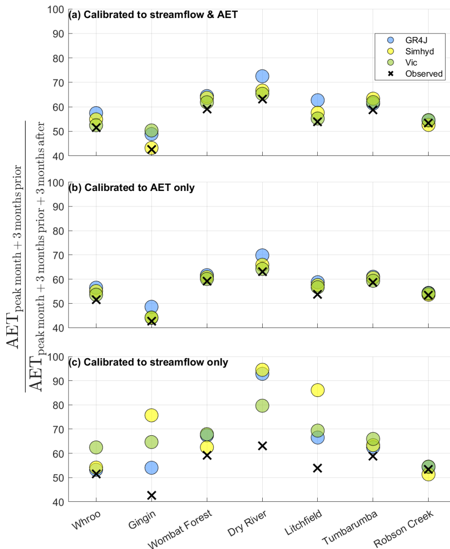
Figure 8. Percentage of AET which occurs in the first half of the observed seasonal peak, for each catchment and model combination, utilising evapotranspiration equation evap_19 . The models are calibrated to (a) streamflow and AET, (b) AET only, and (c) streamflow only. Note: The 7-month period is determined by identifying the peak month of observed AET (the most common peak month across the flux data time period—one of the AET signatures). The values shown represent the total AET accumulated in the first four months (including the peak month) as a percentage of the total AET over the full 7-month period. Catchments are ordered by increasing total AET over the 7-month period.
