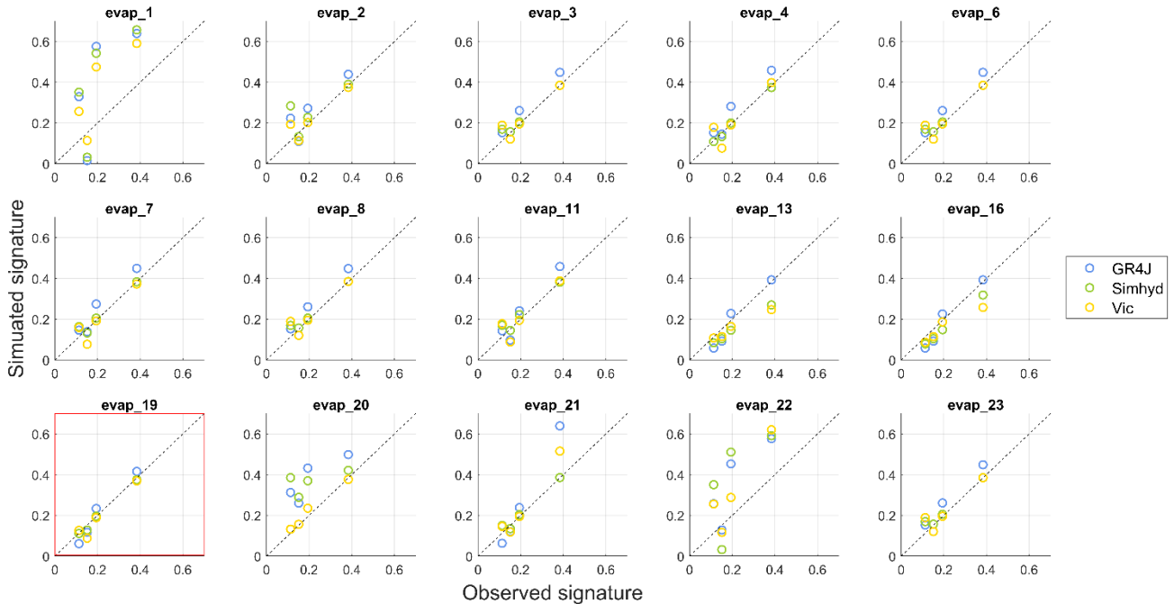
Figure 6. Monthly asynchronicity of AET: observed vs. simulated, across all equations and models. AET equation evap_19 is highlighted with a red box. Remaining signature plots are in supplementary materials S6. This signature is purely based on the
