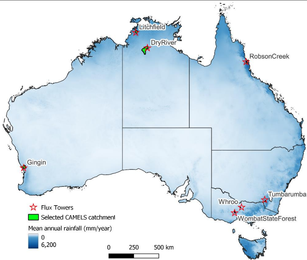
140 Figure 2: Map of Australia showing the seven flux tower sites and their associated catchments.
