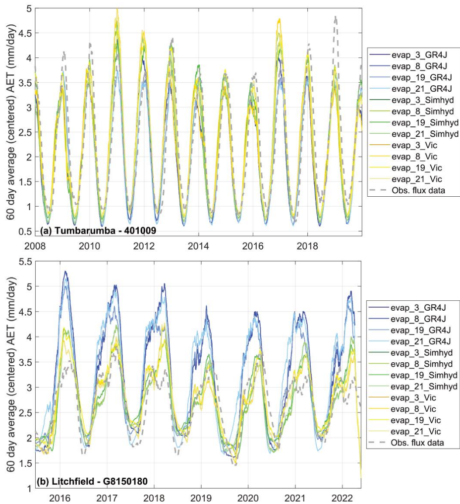
315 Figure 5. Modelled AET vs. observed flux tower data, showing the four best performing AET equations across the three models at Tumbarumba (a) and Litchfield (b).
