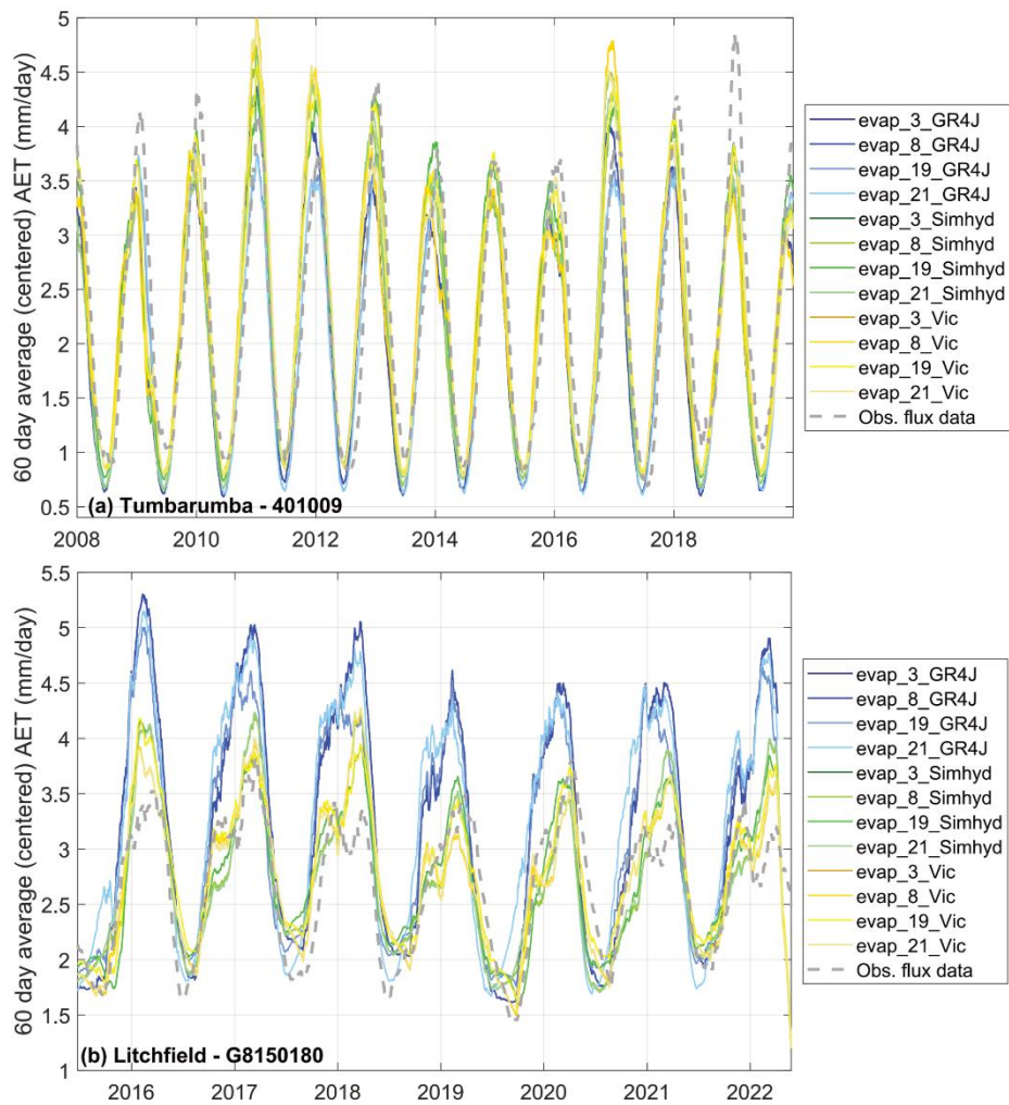
Figure 5. Modelled AET vs. observed flux tower data, showing the four best performing AET equations across the three models at Tumbarumba (a) and Litchfield (b).
