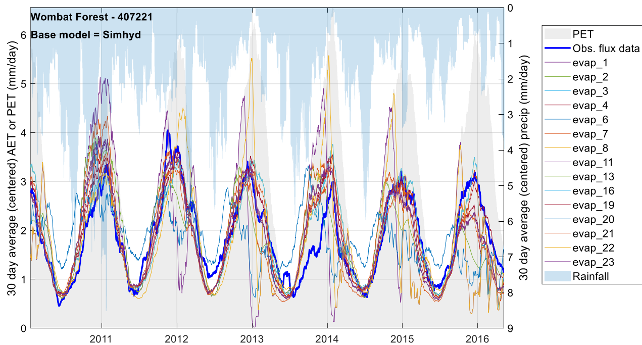
285 Figure 3. Observed flux tower data, precipitation, and PET for Wombat Forest, Victoria, Australia. 15 calibrations showing simulated AET at the site (evap_1, evap_2, etc.) for the base model (Simhyd).
