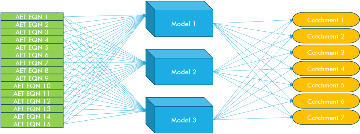
Figure 1: General methodology visualisation. By holding the model structure constant and only varying the AET equation, this approach isolates the influence of different AET equations on model performance.
