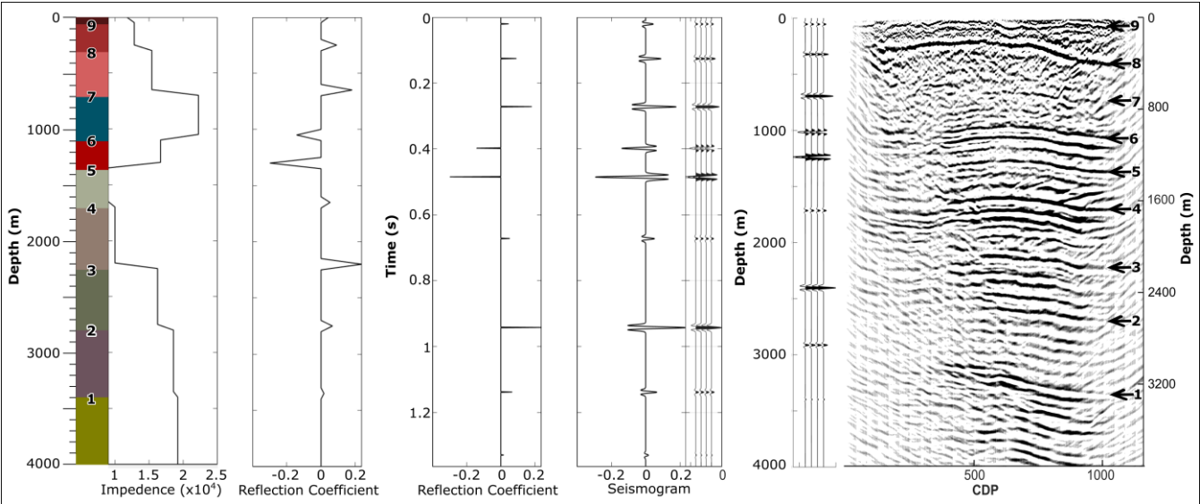
Figure 9: One-dimensional (1D) synthetic seismogram generated using average physical properties derived from interpreted geological contacts on the seismic profiles, as well as profile 1 showing key reflection contacts numbered 1 to 9 from bottom to top and correspond to: (1) the Ventersdorp Supergroup – Campbellrand and Schmidtsdrif Subgroup contact; (2) Campbellrand and Schmidtsdrif – Asbestos Hills and Koegas Subgroup contact; (3) the boundary between the Ghaap and Postmasburg Groups; (4) the Makganyene–Ongeluk Formation contact; (5) the Ongeluk–Hotazel Formation contact; (6) the Hotazel–Moodraai Formation contact; (7) the pre-Gamagara unconformity between the Transvaal and Keis Supergroups; (8) the Keis–Karoo Supergroup contact; and (9) the surface unconformity between the Karoo Supergroup and the overlying Kalahari Group.
