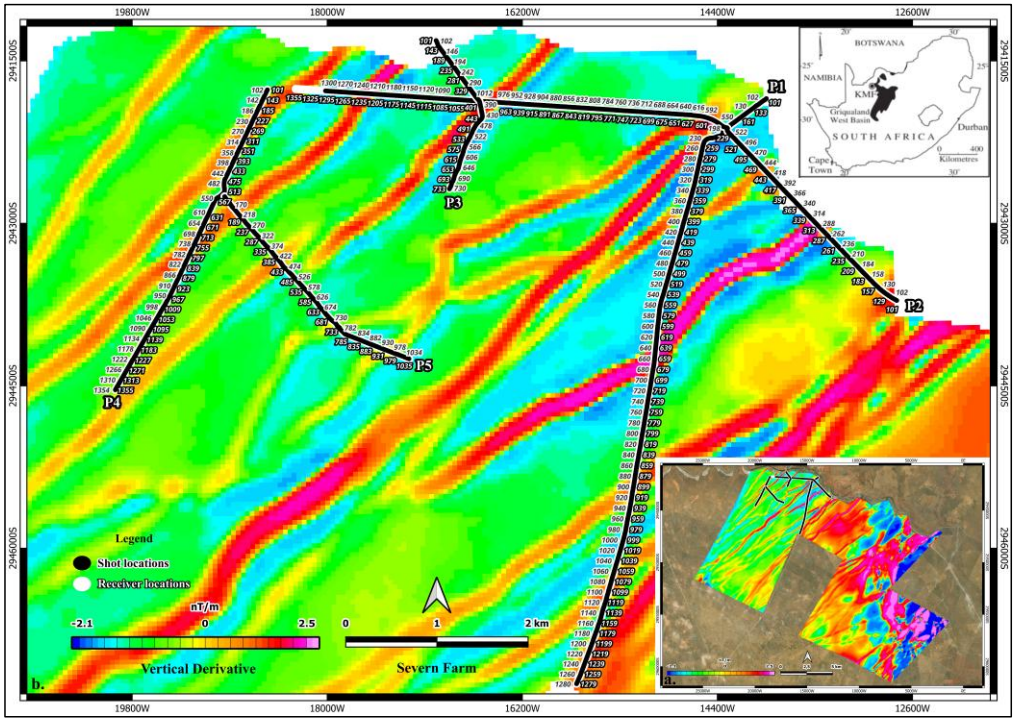
90 Figure 2: Seismic acquisition layout in relation to magnetic anomalies across the Kalahari Manganese Field (KMF). (a) First vertical derivative (1VD) of the Total Magnetic Intensity (TMI) map with 2D reflection seismic profiles overlain, illustrating the correlation between subsurface magnetic structures and the seismic survey lines. (b) Zoomed-in view of the Severn farm area showing the detailed layout of the 2D seismic profiles with shot and receiver positions superimposed on the magnetic map. The map highlights localized magnetic anomalies associated with subsurface lithological contrasts relevant to manganese exploration. 95 A detailed geological interpretation of these seismic lines has been presented by Jogee et al. (2025). In the present study, we extend this work by focusing focus on the near-surface characterization using both reflected and refracted wavefield energy to provide an integrated understanding of the shallow subsurface architecture. We further demonstrate how numerical seismic simulations can be effectively utilized to design and optimize data acquisition parameters, assess processing workflows, and guide geological interpretation in complex terranes such as the Griqualand West Basin. In addition, we present and compare results from pre-stack time and depth Kirchhoff migration approaches to evaluate their relative performance in enhancing the imaging of manganese-bearing stratigraphic horizons and associated geological contacts. Finally, we compute the seismic attribute (e.g., cosine of phase) on the seismic sections to enhance the detection of the manganese mineralised zones and compare the results with the traditional seismic amplitude displays. 100
