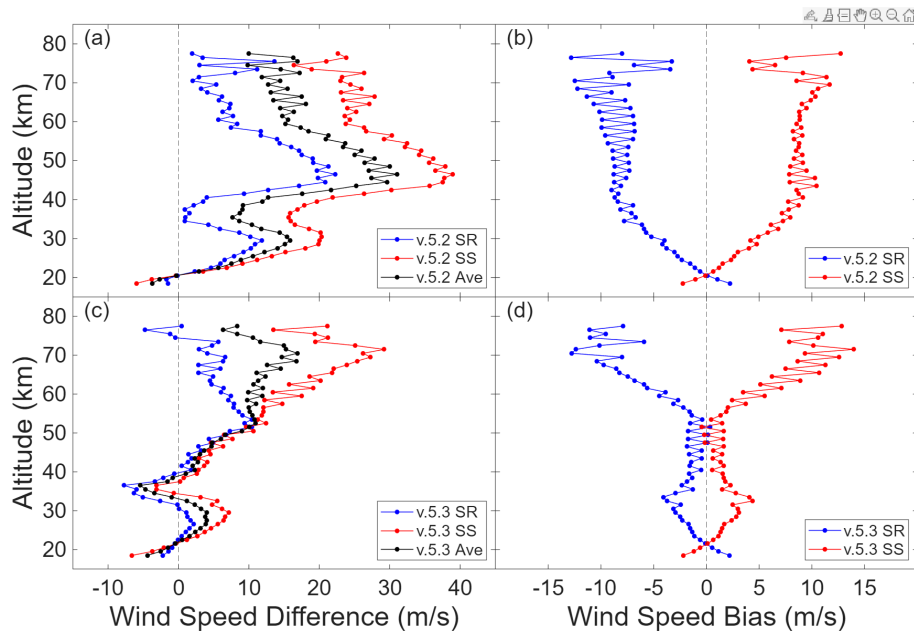
Figure 11. (a) Average difference between ACE v.5.2 (sunrise (blue), sunset (red), and both (black)) and MERRA-2 winds for each ACE wind speed measurement in 2019. (b) ACE sunrise-sunset bias, shown as the difference between sunrise and sunset averages and the total average in (a). Plots (c) and (d) are the same as (a) and (b), respectively, but for ACE v.5.3 processing.
