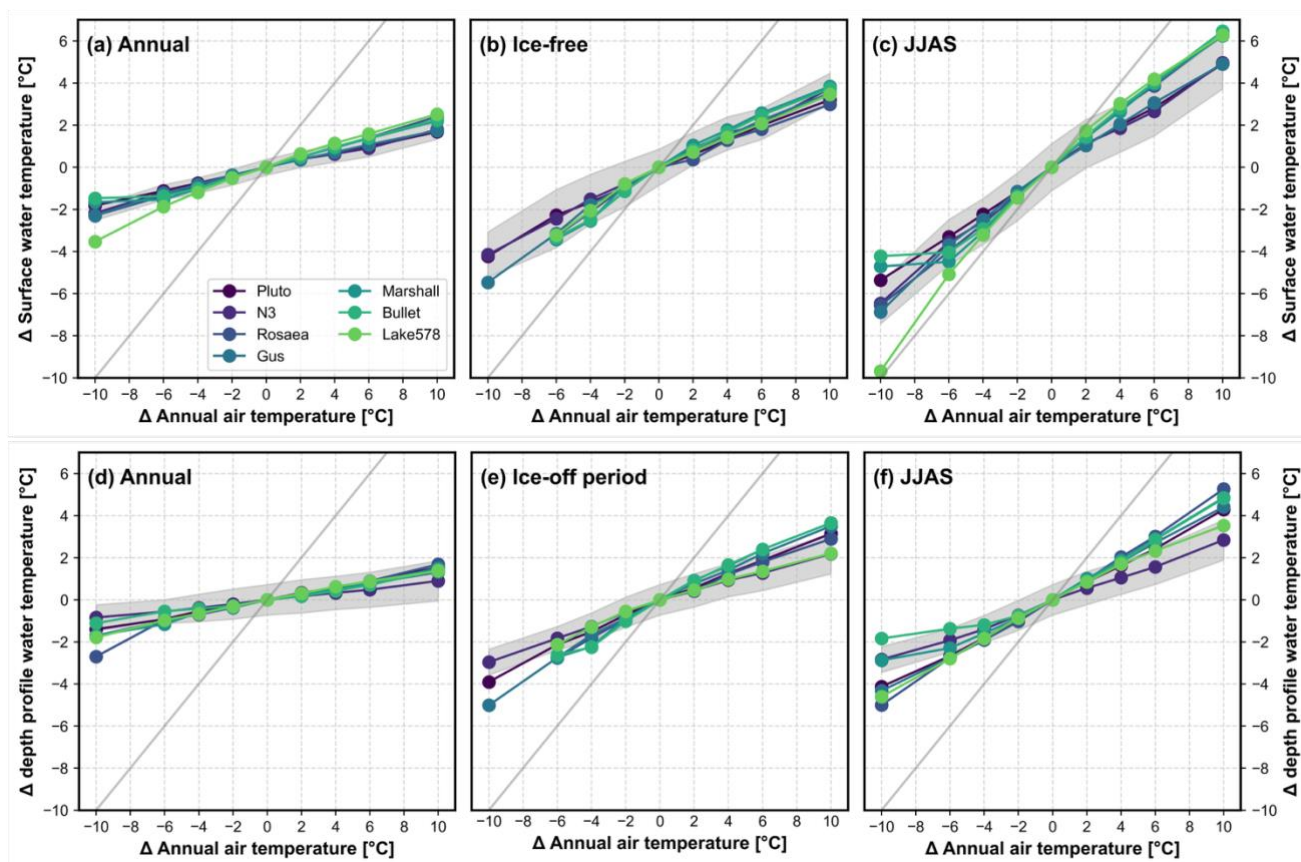
345 Figure 4: Sensitivity of surface water (a–c) and average depth profile temperatures (d–f) to changes in annual air temperature. (a) and (d) annual, (b) and (e) IFS, (c) and (f) JJAS water temperature [°C]. Each point denotes the median value of the 30-year simulation. The grey line is the 1:1 line. Grey shading represents the standard deviation for the 30 years simulated for Lake N3. Standard deviation is on the same order as for other lakes. For some lakes, simulations under 10 °C lower magnitude of temperature change than modern resulted in year-round ice cover; therefore, these simulations were not plotted.
