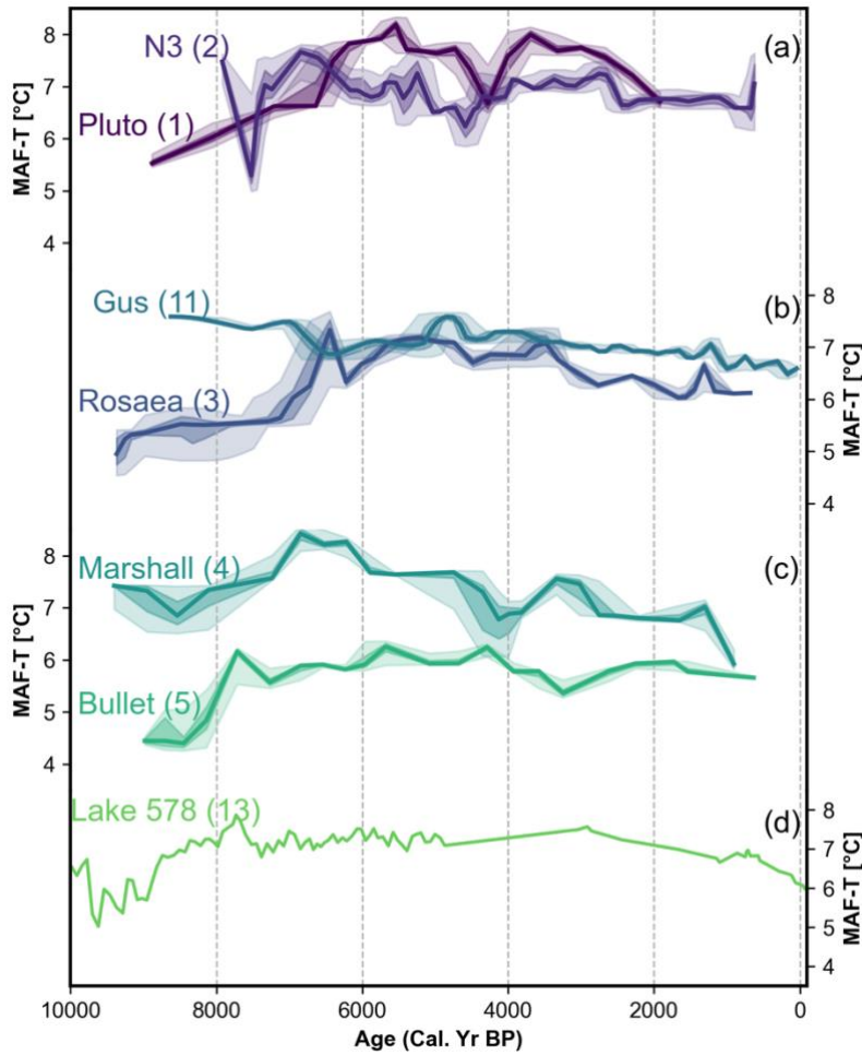
Figure 2: Reconstructed mean air temperatures of the months above freezing (MAF-T) in (a) Lakes N3 and Pluto at 69 °N, (b) Lakes Gus (Cluett et al., 2023) and Rosaea at 67 °N, (c) Lakes Marshall and Bullet at 64 °N, and (d) Lake 578 at 61 °N (Schneider et al., 2024). For timeseries in a–c, the bold line indicates the median modelled age, and the light and dark shading represent the 95 th percentile and interquartile age uncertainty, respectively. Numbers in parentheses next to site names refer to site IDs shown in Fig. 1.
