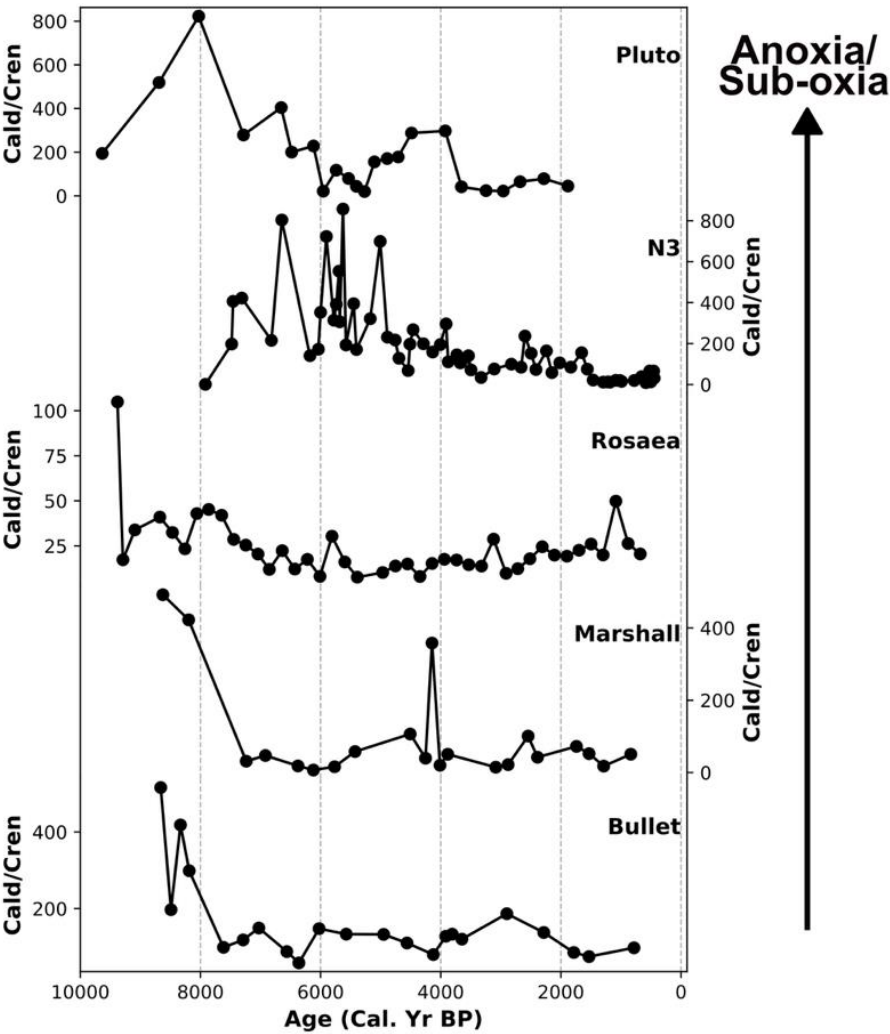
Figure 5: Variations of the ratio of caldarchaeol to crenarchaeol (Cald/Cren) in the study lakes.
