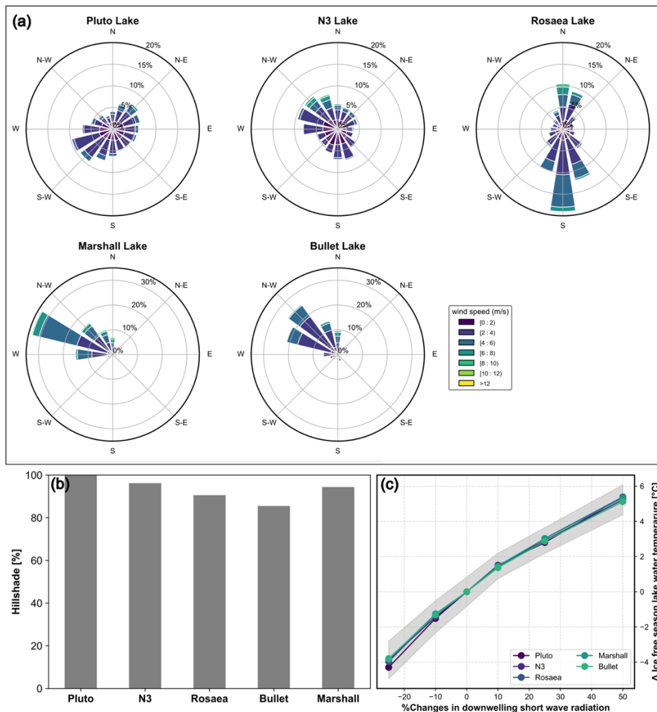
Figure 6: (a) Wind strength and direction in the study lakes from April to September, based on six-hourly ERA5 data from 1994 to 2024. (b) Percentage change in average summer (April to September) direct radiation on study lakes relative to Pluto Lake, which is the least shaded of the five. (c) Sensitivity of average surface water temperature to changes in incoming shortwave radiation. Each point denotes the median value of the 30-year simulation. Grey shading represents the standard deviation for the 30 years simulated for Lake N3. Standard deviation is on the same order as for other lakes.
