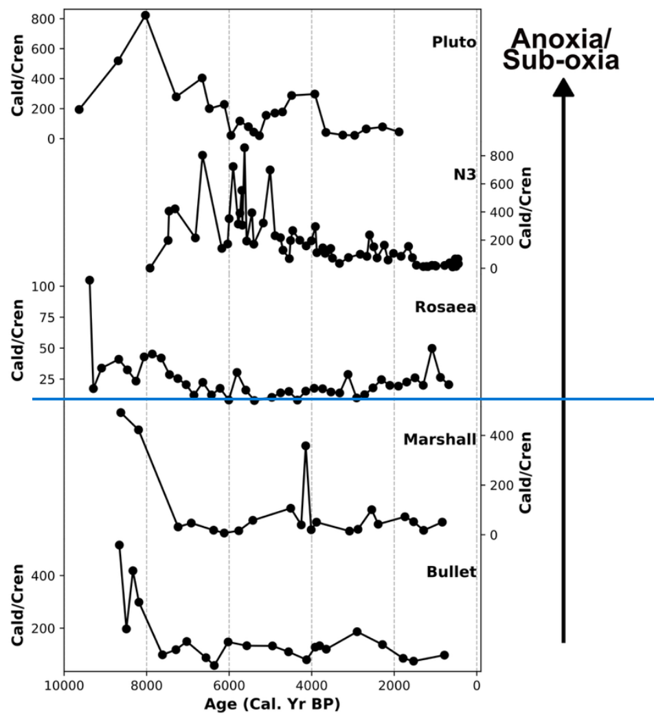
Figure 5: Variations of the ratio of caldarchaeol to crenarchaeol (Cald/Cren) in the study lakes.
