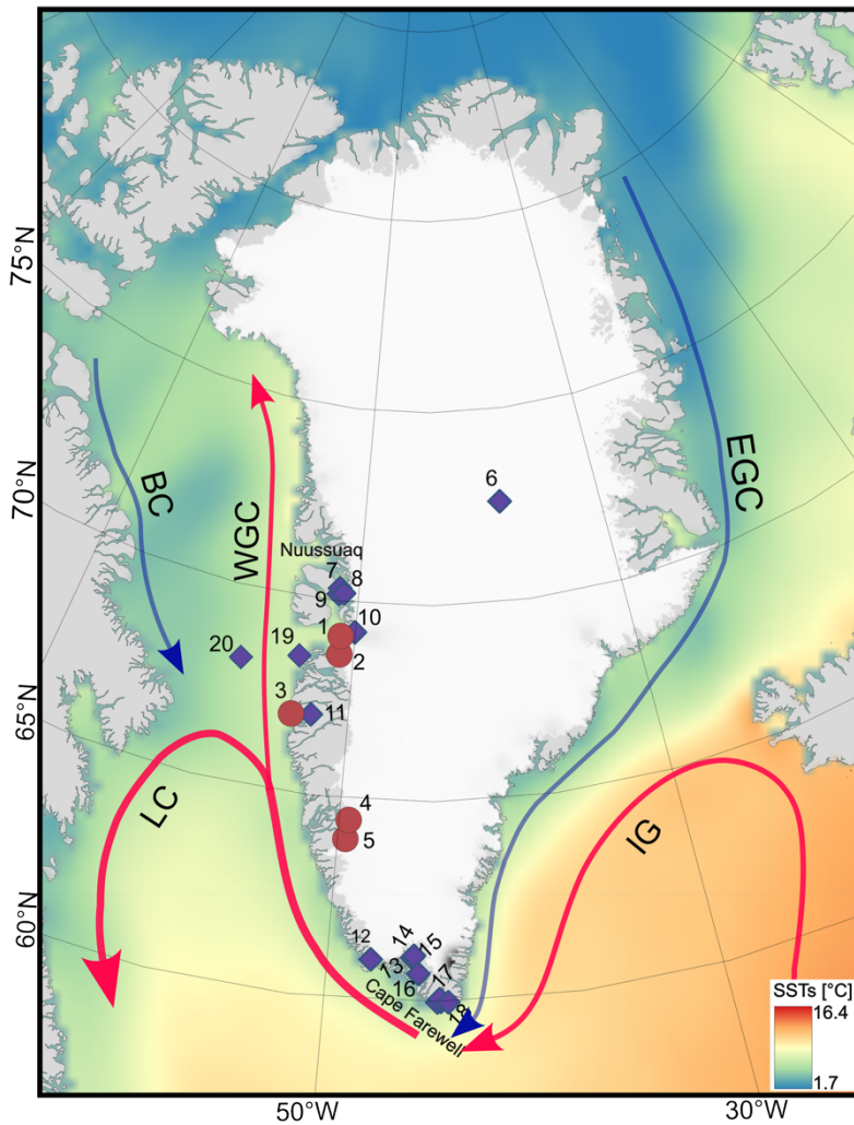
Figure 1: Map of Greenland and surrounding area showing study lakes in brown circles (1–5), sites mentioned in the text in blue diamonds (6–20) and ocean currents; WGC: West Greenland, EGC: East Greenland, IRIG : Irminger, BC: Baffin, and LC: Labrador currents . Site numbered as follows: (1) Pluto, (2) N3, (3) Rosaea, (4) Marshall (5) Bullet (6) GISP2 (Kobashi et al., 2017), (7) Sermikassak, (8) Qangattaq ice cap (9) Saqqap Tasersua (Schweinsberg et al., 2017, 2019) (10) North Lake (Axford et al., 2013) (11) Lake Gus ( Cluett et al., 2023 )( Cluett et al., 2023 ) (12) Qipisarqo (Frechette and de Vernal, 2009; Kaplan et al., 2002) (13) Lake 578 (Schneider et al., 2024) (14) Spongilla Sø (Fredskild, 1973; Gajewski, 2015) (15) Alakariqssq glaciers (Larocca et al., 2020) (16) Comarum Sø (Fredskild, 1973; Gajewski, 2015) (17) N14 (Andresen et al., 2004), (18) Quvnerit glaciers (Larocca et al., 2020), and marine sediment cores (19) MSM343300 (Ouellet-Bernier et al., 2014) and (20) CC70 (Gibb et al., 2015). The fill colour represents modern summer sea surface temperatures (SSTs), data source: (*Fisher et al., 2023; Moon et al., 2023) ( Fisher et al., 2023; Moon et al., 2023 ).
