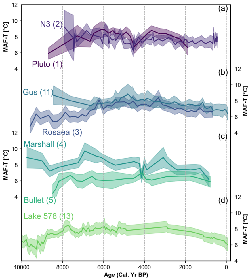
Figure 25: Reconstructed ice-free season lake water mean air temperatures ( HFS-LWT of the months above freezing (MAF-T) ) in (a) Lakes N3 and Pluto at 69 °N, (b) Lakes Gus (Cluett et al., 2023) and Rosaea at 67 °N, (c) Lakes Marshall and Bullet at 64 °N, and (d) Lake 578 at 61 °N (Schneider et al., 2024). For timeseries in (a – c), bold line Bold lines indicate median-modeled age-average MAF-T inferred from three high-latitude lacustrine brGDGTs calibrations (Otiniano et al., 2023, 2024; Raberg et al., 2021), and light and dark shading represents 95 th percentile and interquartile age uncertainty, respectively represents standard deviation of these calibrations . Numbers in parentheses next to site names names refer to site IDs shown in Fig. 1.
