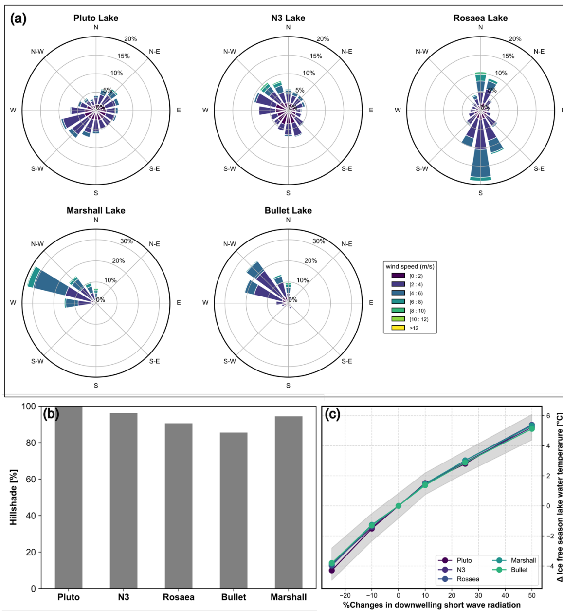
Figure 67: (a) Wind strength and direction in the study lakes from April to September, based on six-hourly ERA5 data from 1994 to 2024. (b) Percentage change in average summer (April to September) direct radiation on study lakes relative to Pluto Lake, which is the least shaded of the five. (c) Sensitivity of average surface water temperature to changes in incoming shortwave radiation. Each point denotes the median value of the 30-year simulation. Gray shading represents the standard deviation for the 30 years of model run simulated for Lake N3. Standard derivation deviation is on the same order for other lakes.
