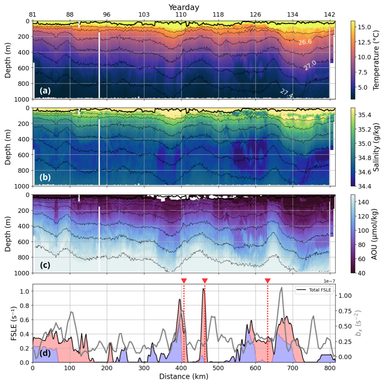
Figure 2. Glider sections showing (a) conservative temperature, (b) absolute salinity and (c) AOU. Isopycnals are overlaid using thin black contours and the MLD is depicted with the thick black line. (d) Averaged FSLE over a 0.125-degree radius around the gliders position, composed of diverging FSLE (red) stacked onto the converging FSLE (blue). The horizontal buoyancy gradient ( b_x ) is averaged between 300 – 700 m depth and shown in the gray line. The red dashed lines and arrows indicate yeardays corresponding to the satellite images of FSLE in Fig. 3.
