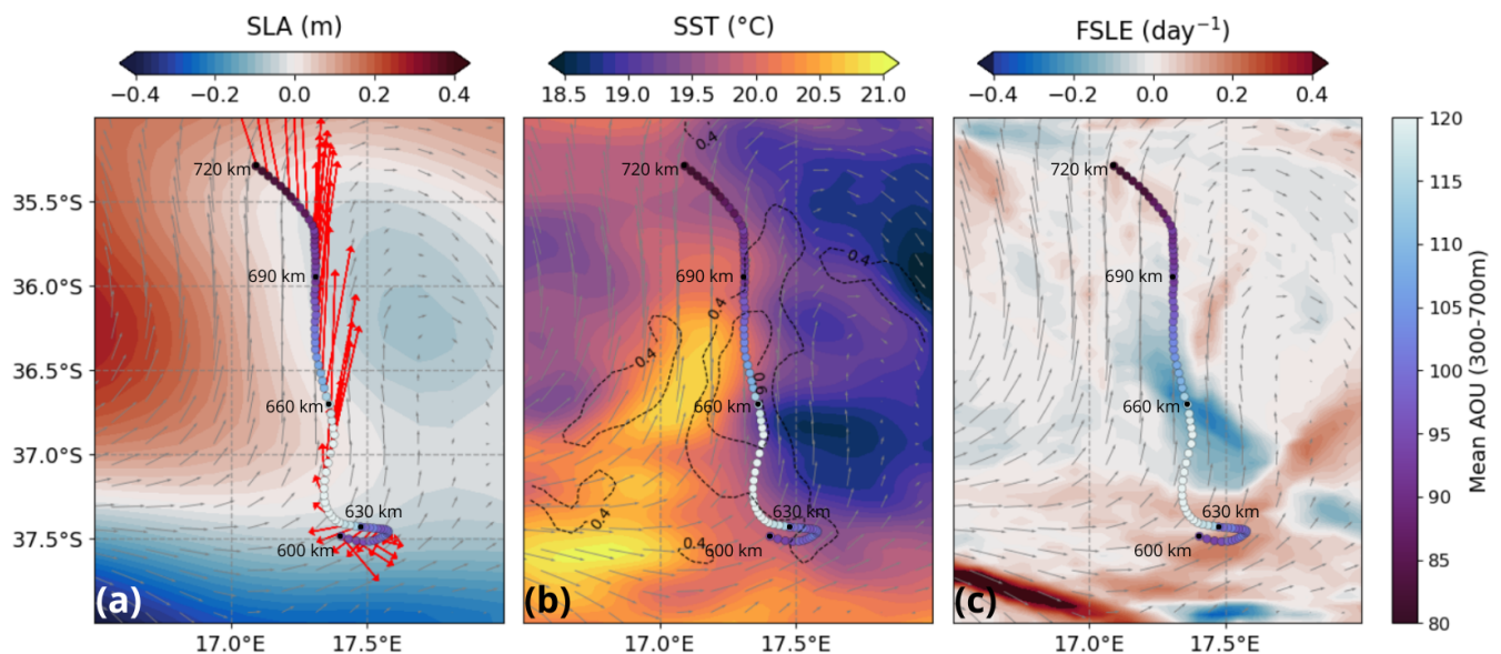
Figure 7. Daily average over 2023-05-06 to 2023-05-16 of (a) SLA, with red arrows representing the Depth-Average Current, (b) SST, where the dashed contour lines indicate the temperature gradient and (c) FSLE. Geostrophic velocities are represented with the grey vector field. Scattered dots represent the glider trajectory between 600 and 720 km. The color indicates the mean AOU between 300 and 700 m depth.
