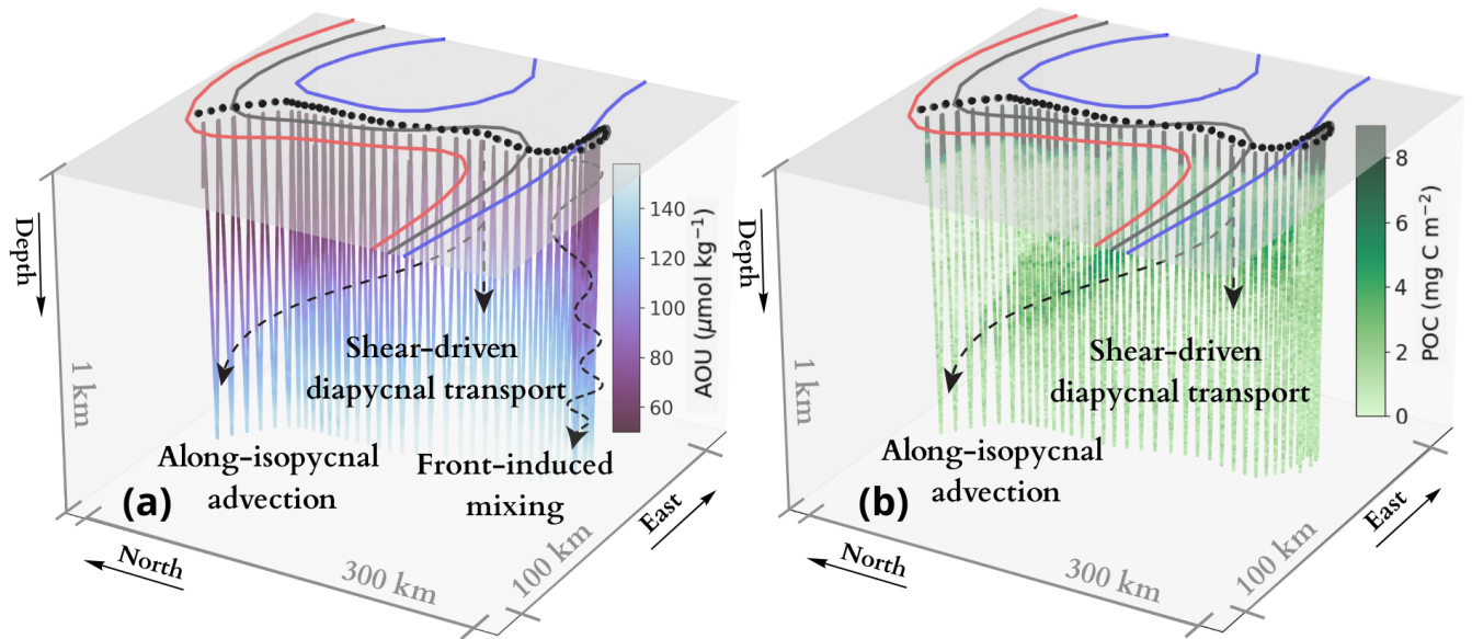
Figure 8. 3D glider transect of (a) AOU and (b) POC. The blue, grey, and red lines represent the Sea Level Anomaly (SLA) respectively (-0.5, 0, 0.5) m.
