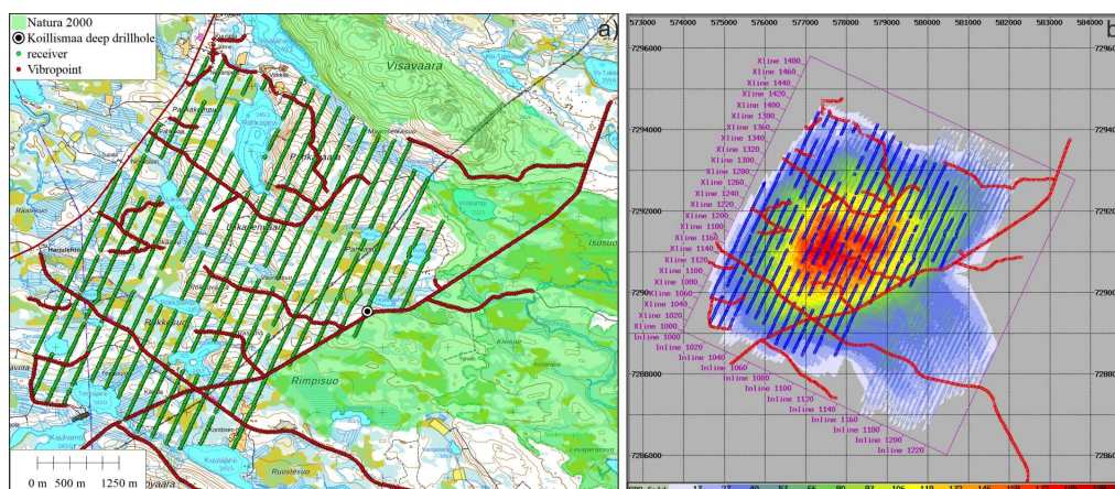
175 Figure 4: Layout of the SEEMS DEEP 3D seismic survey (a) and the corresponding CDP fold (b).
