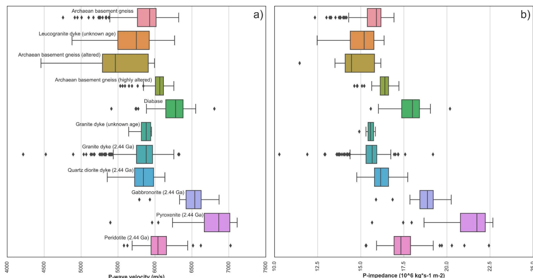
Figure 2: a) Box-and-whisker plot of the measured P-wave velocity using core samples from the Koillismaa deep drillhole grouped by the rocktype and ordered approximately by depth. The 2.44 Ga is related to the intrusion. b) Corresponding acoustic impedance plot based on the co-located velocity and density measurements.
