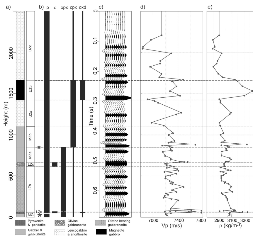
Figure 3: a) Representative stratigraphic section of KLIC based on the profile across the Porttivaara block (Karinen, 2010); b) In the sequence thick vertical lines indicate cumulus minerals and thin vertical lines indicate intercumulus minerals (p-plagioclase, o – olivine, opx – orthopyroxene, cpx – clinopyroxene, oxd – Fe-Ti oxides); stars denote occurrence of sulphide mineralisation (up to 3%); c) corresponding filtered (up to 62.5 Hz) zero-offset reflection coefficient series based on the velocity and density calculated from modal mineralogy; d) calculated velocity log; e) calculated density log. Points represent samples and the lines are the interpolated values.
