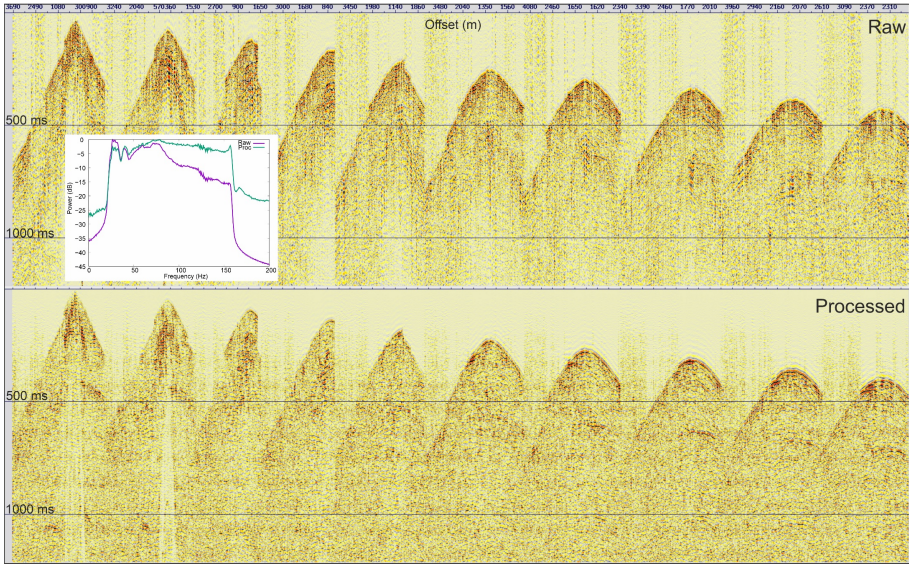
Figure 5: Example of raw (a) and processed (b) shot gather. Inset figure on the top shows the amplitude spectra of raw shot gather (in purple), and after full preprocessing for the same (in green).
