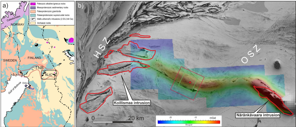
Figure 1: a) Simplified geological map of the Fennoscandian Shield (modified from Karinen 2010); KLIC = Koillismaa– Näränkävåara Layered Intrusion Complex, TNB = Tornio–Näränkävåara Belt; b) location of the study area with the composite image of the magnetic anomaly (Aeromagnetic anomaly map of Finland © Geological Survey of Finland 2016), Bouguer gravity anomaly (Salmirinne and Iljina, 2003) and simplified bedrock geology (Bedrock of Finland 1:1 000 000 © Geological Survey of Finland 2016) maps. Red dot marks the Koillismaa drillhole, rectangles mark the extend of the SEEMS DEEP 3D seismic survey (green) and the Common Earth Model area (red); HSZ = Hivaskoski Shear Zone, OSZ = Oulujärvi Shear Zone. Total Magnetic Intensity shading from low (white) to high values (black).
