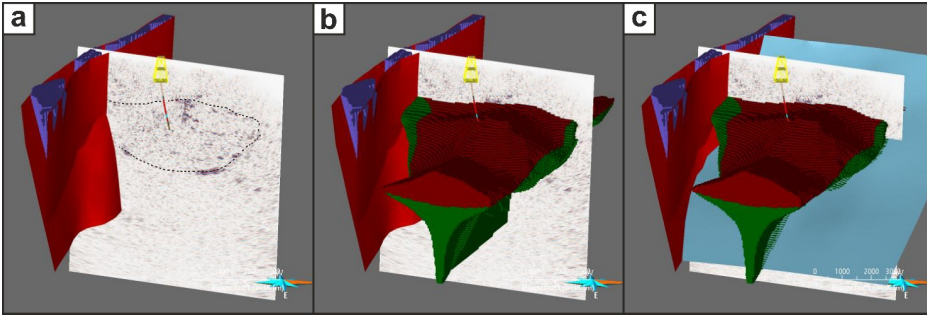
310 Figure 12: Snapshots of the CEM viewed roughly westward, showing the main lithological units (BIF and intrusion) and associated structures (red and pale blue surfaces). (a) BIF belt (purple) along a fault system (red), (b) voxel model of the intrusion, (c) geometry of the reverse fault (pale blue).
