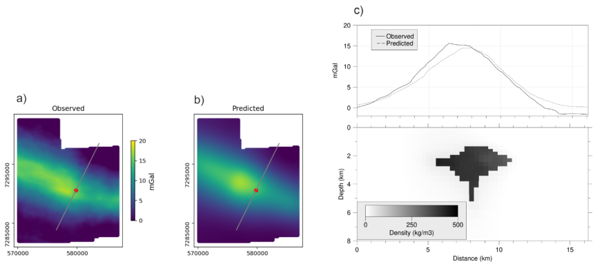
315 Figure 13: Gravity appraisal of the CEM. Gravity inversion was carried out by allowing density contrast to preferentially only exist within the modelled KDI. (a) Observed, and (b) predicted gravity anomaly. (c) Cross-section of the density model and the gravity response along the profile marked with the grey line in (a) and (b). 0 km on the profile represents the southern end of the line. Red dot marks the location of the Koillismaa drillhole.
