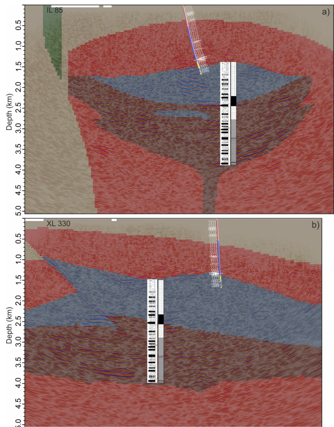
300 Figure 11: Inline 85 and crossline 330 from the final PreSTM volume (depth converted) with the CEM lithologies in the background. Synthetic seismogram and stratigraphic section from Fig. 3 is also shown for comparison.
