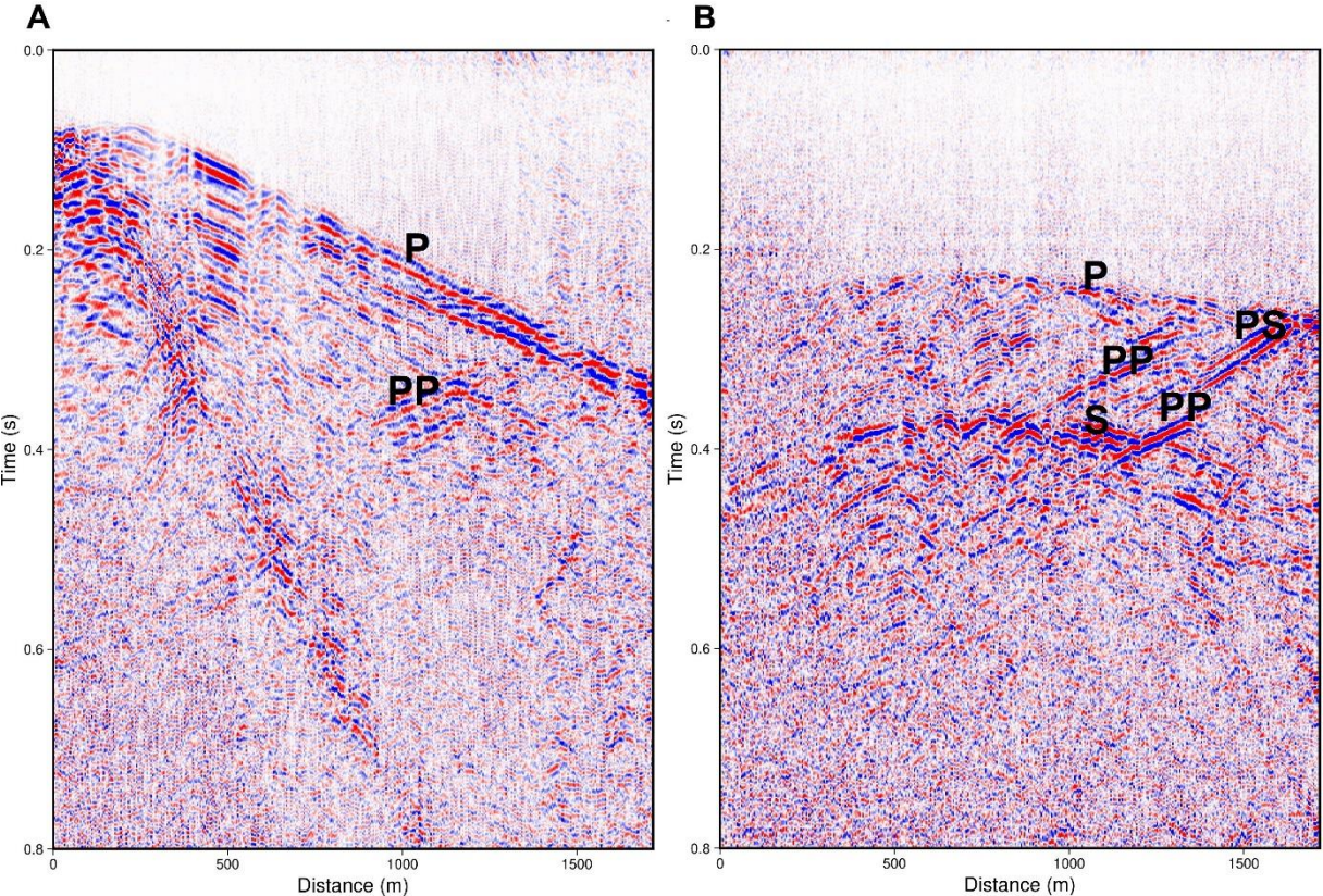
Figure 9: Seismic records from the walkaway VSP survey, with increasing depth towards right (the x-axis shows distance as measured along the drill hole). A) Record for a source point close to the drill hole. In this case the down going P-wave has a roughly linear appearance. B) Record for a source at some distance from the drill hole, in which the down going P-wave shows curvature. For clarity, the tube waves have been suppressed prior to display. Spectral balancing and AGC have also been applied. See text for description of the annotated seismic phases.
