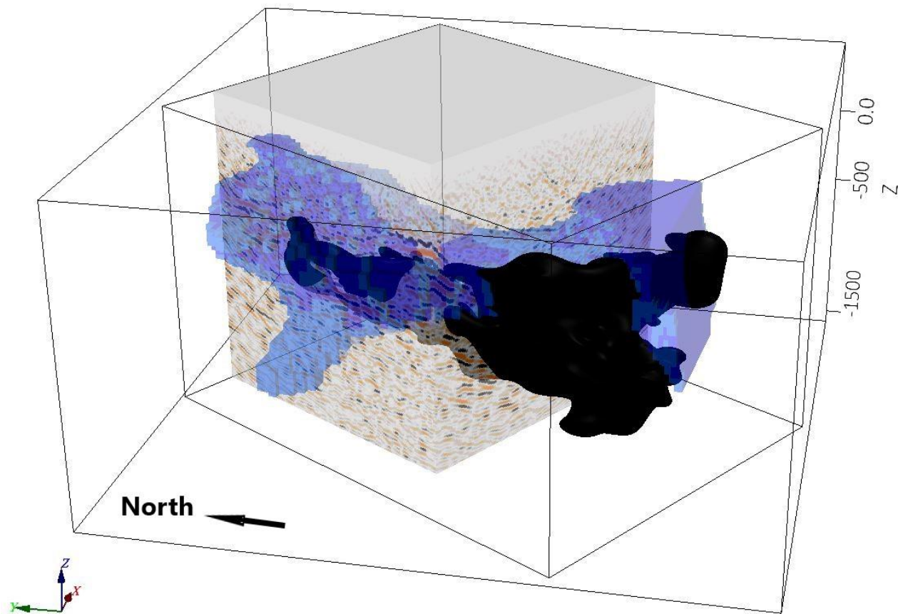
280 Figure 11: Pre-stack migrated depth volume from the 3D survey, in comparison with the geological model for the Per Geijer Deep mineralization, shown in black. Also shown in blue is the electrical conductivity model from a semi-airborne EM survey (Smirnova et al, 2020). All cells with conductivity >0.02 S/m are shown. The seismic volume and the conductivity model are semi-transparent.
