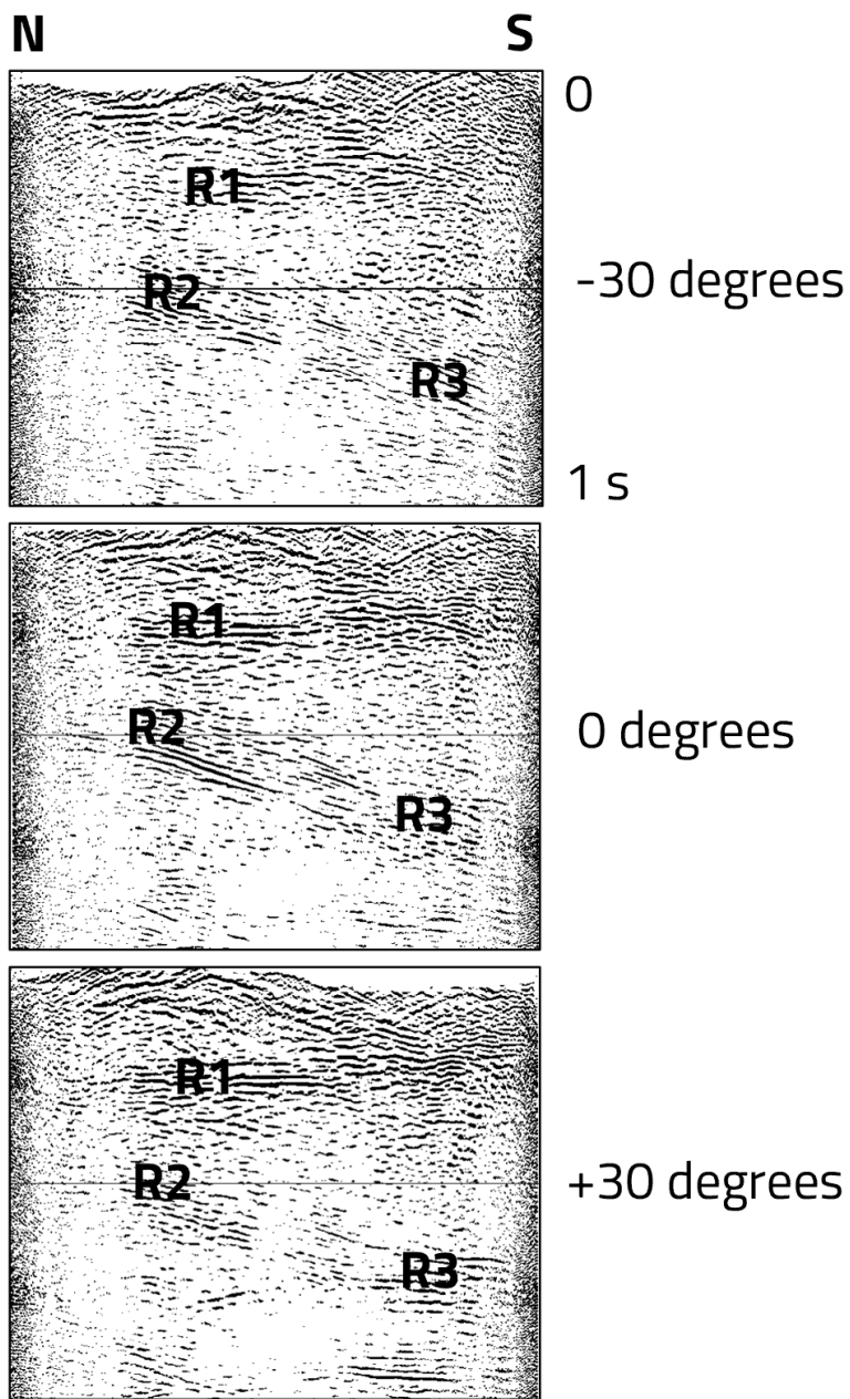
Figure 6: Cross-dip analysis for Profile 3. The data have been stacked assuming different cross-dip angles of the reflections, i.e. dip perpendicular to the profile direction, which is approximately north-south. The cross-dip is measured relative to horizontal and defined as positive for reflections dipping to the east. Reflection R2 has the highest amplitude for zero cross-dip, whereas R1 and R3 has highest amplitude for 30 degrees cross-dip towards east.
