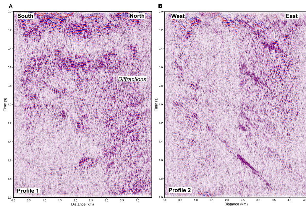
Figure 5: A) Stacked time section from Profile 1. B) Stacked time section from Profile 2. The change in reflection character at about 2.4 km along Profile 2 is caused by a change in the stacking fold.
