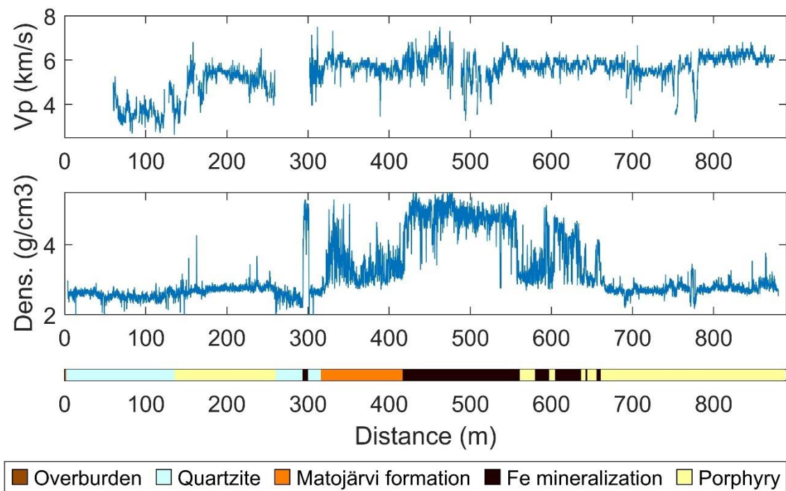
Figure 3: Wireline logs from one drill hole intersecting the Per Geijer Deep iron mineralization. The lithology description has been simplified.
