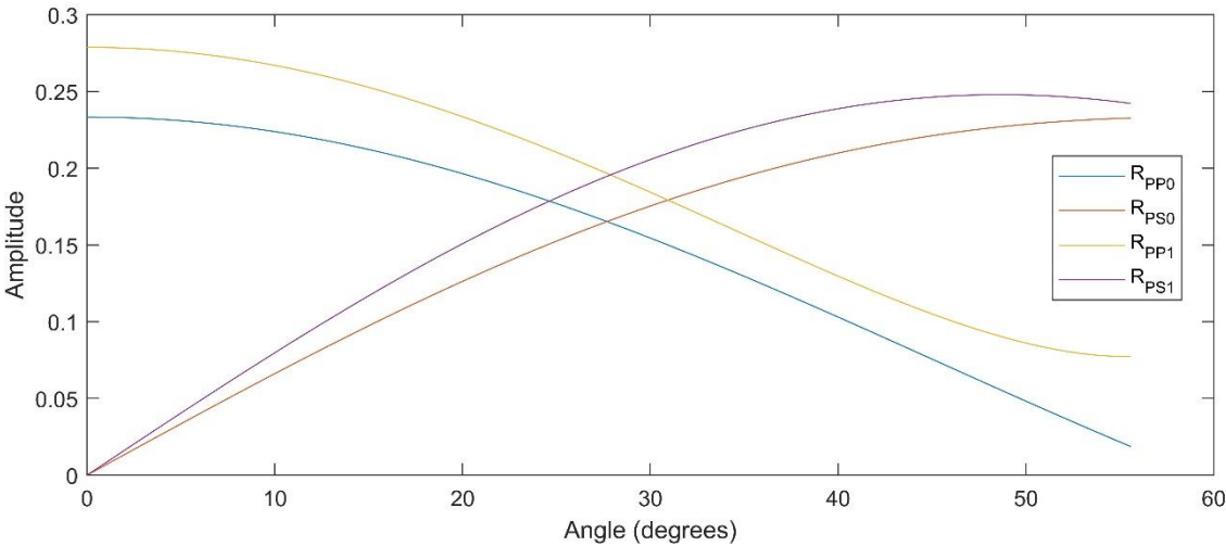
Figure 14: Calculated approximate reflection coefficients for the Per Geijer Deep mineralization. The angle is measured relative to vertical, with 0 degrees referring to normal incidence. R_{PP0} and R_{PS0} represent the case of no velocity contrast, whereas R_{PP1} and R_{PS1} represent a P-wave velocity increase from 5.5 to 6.0 km/s, and S-wave velocities defined through a V_P/V_S ratio of 1.72. For both cases, the density increases from 3.0 to 4.4 g/cm 3 at the contact.
