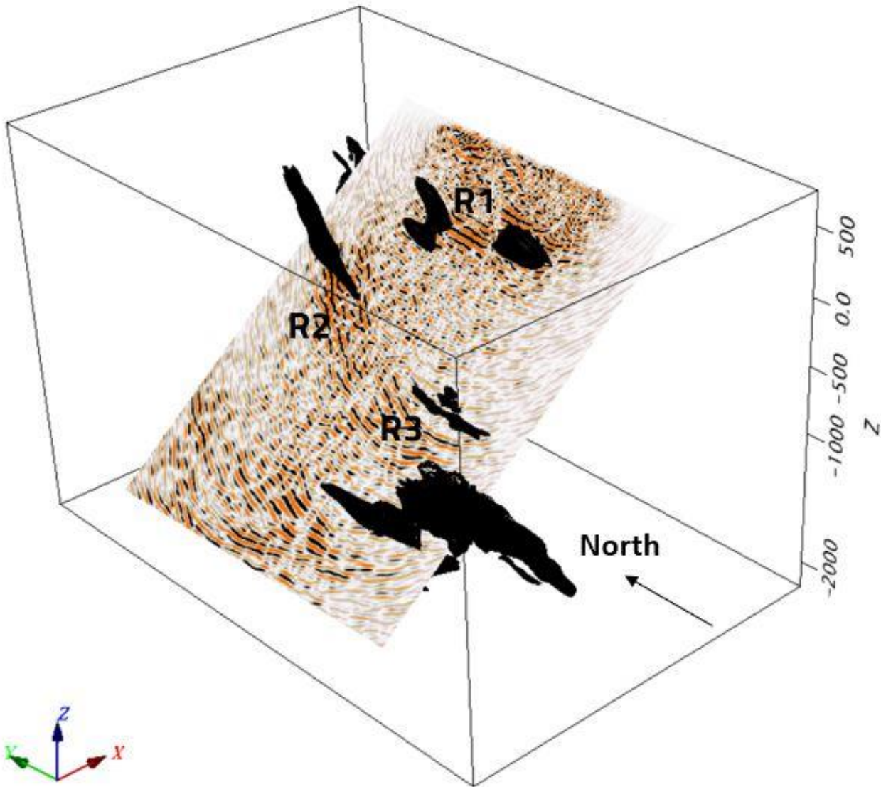
Figure 12: Depth section from Profile 3, plotted at an angle to account for the reflections mostly coming from the western side of the seismic line. The geological models for the iron-oxides are shown in black.
