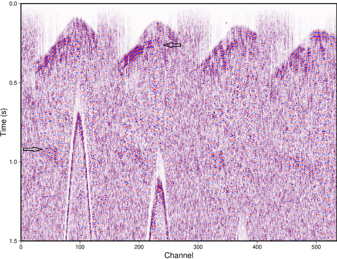
Figure 4: Example shot record data, from the 3D survey. The image only shows a subset of channels. Automatic gain control and frequency filtering has been applied prior to plotting. Arrows mark the reflections discussed in the text.
