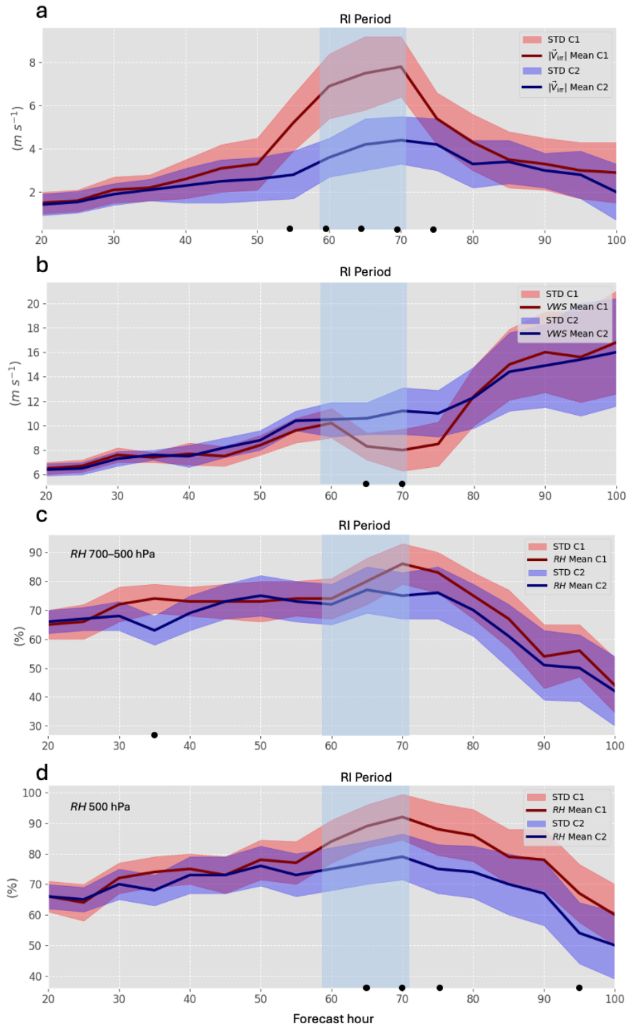
Figure 11. Time evolution of (a) ageostrophic wind at 250 hPa, (b) VWS (850–200 hPa), (c) RH (700–500 hPa) and (d) RH (500 hPa) within 500 km of Lidia. Red (blue) lines show the mean for the higher (lower) IRG; shaded areas indicate STD. Light blue band indicate the RI period. Black dots denote significant differences.
