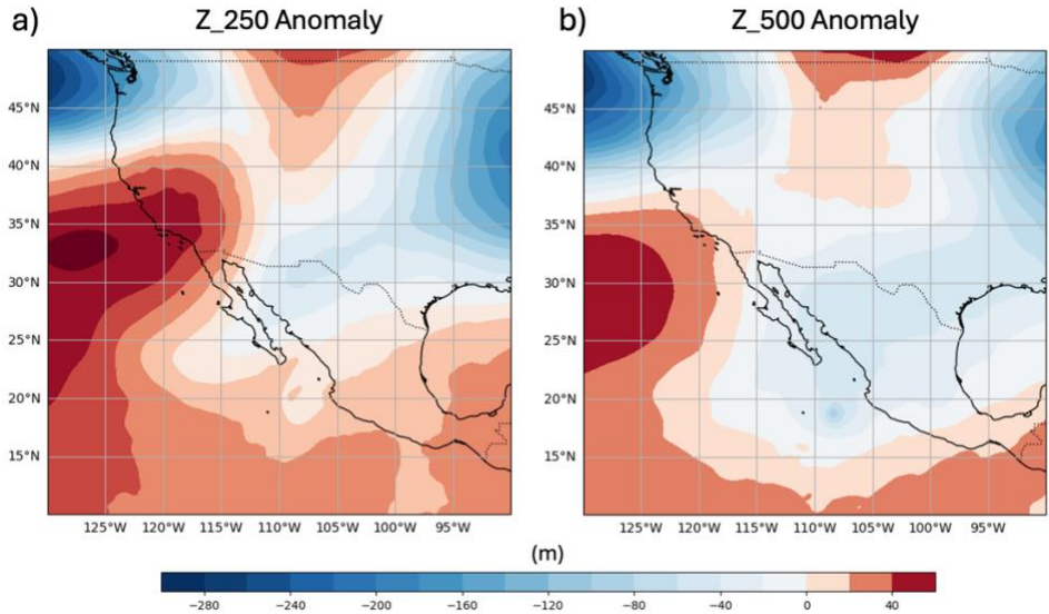
840 Figure A2. Z anomalies from ERA5 for (a) 250 and (b) 500 hPa during the period surrounding 841 Lidia's RI (12:00 UTC on 9 October, 2023). Warm (red) shading denotes positive height 842 anomalies, while cool (blue) shading indicates negative anomalies.
