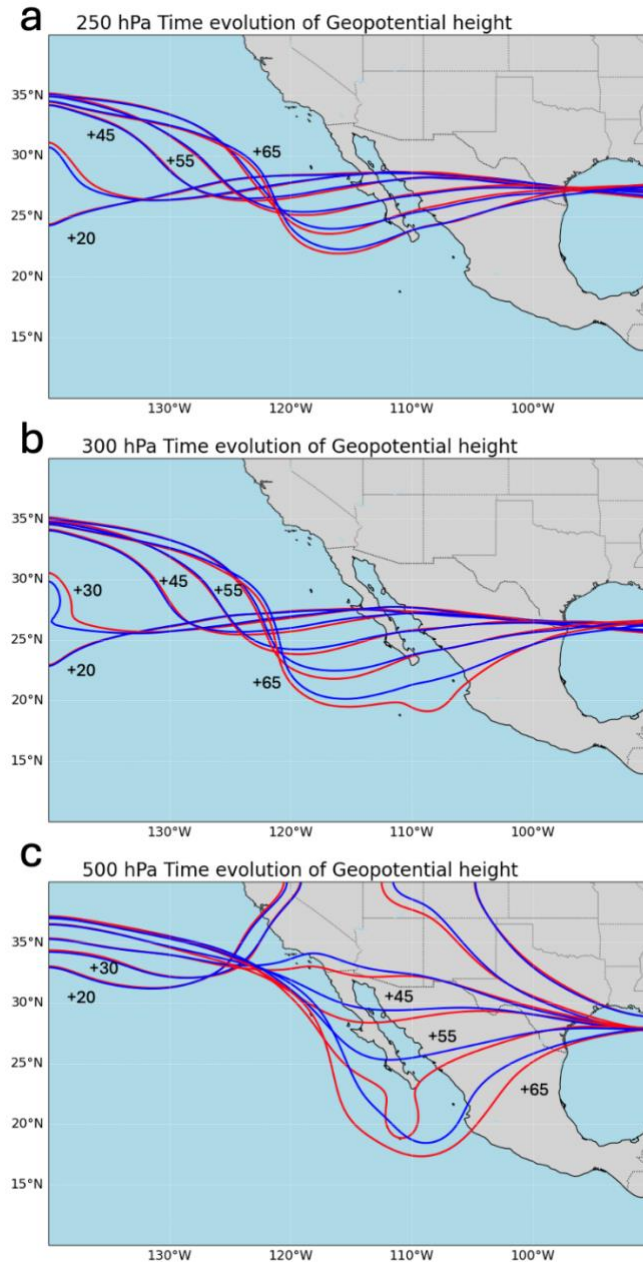
Figure 4. Z Composite corresponding to the highest (red contours) and lower (blue contours) IRG, at (a) 250 hPa, (b) 300 hPa and (c) 500 hPa, before and during the trough-TC interaction.
