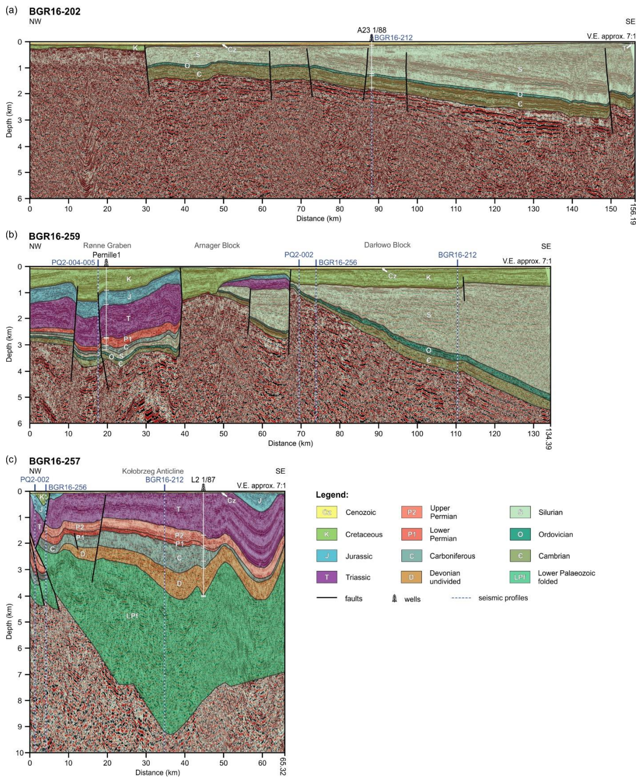
360 Figure 5. Seismic interpretation of the (a) BGR16-202, (b) BGR16-259, (c) BGR16-257 profiles Vertical exaggeration is 7:1.
