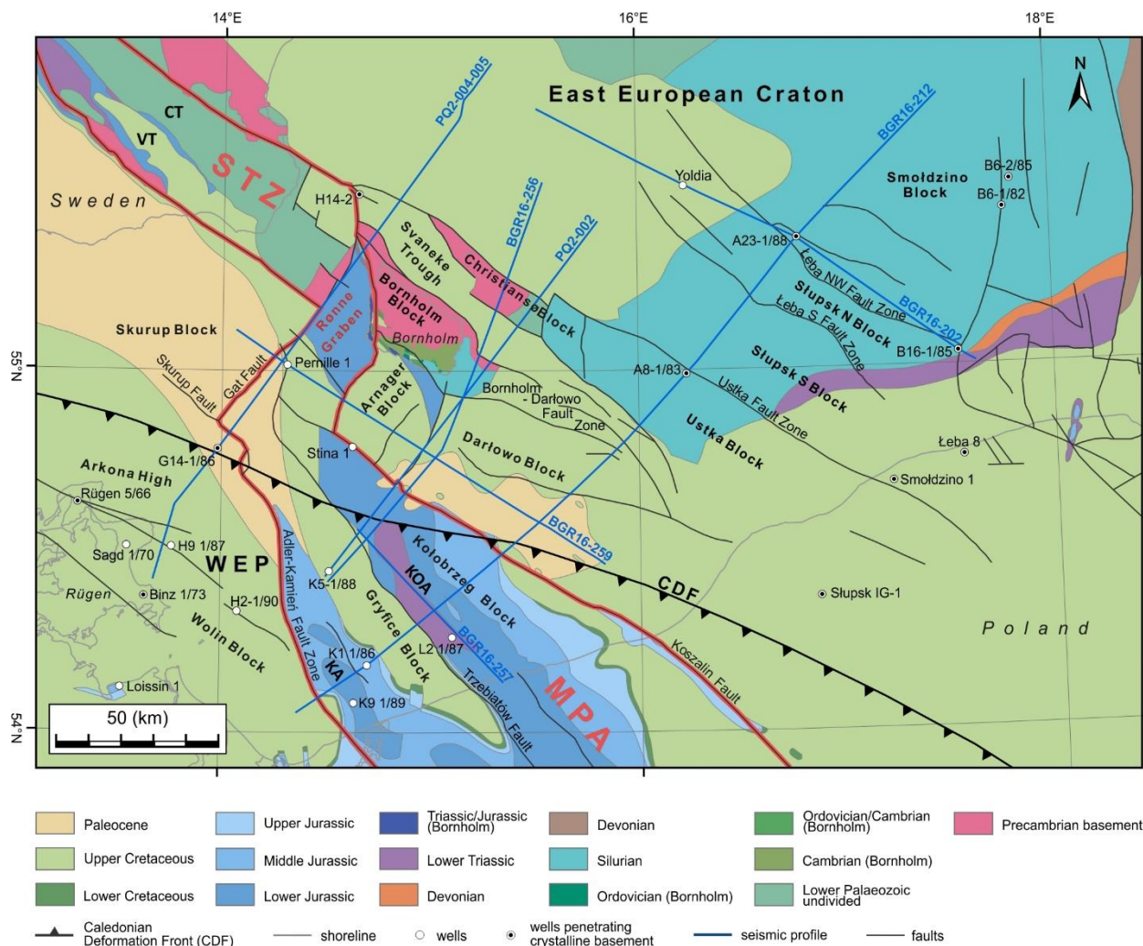
Figure 2. Geological map of the southern Baltic Sea without post-Paleocene sediments after Kramarska et al. (1999), Schlüter et al. (1998), and Sopher et al. (2016) and Pre-Quaternary map of Bornholm (Hansen and Poulsen, 1977). Position of main faults and tectonic blocks are modified from Kramarska et al. (1999), Krzywiec et al. (2003), Jaworowski et al. (2010), Pokorski (2010), Seidel et al. (2018) and Ponikowska et al. (2024). Permian-Triassic depocentres are outlined in red. Abbreviations: CDF, Caledonian Deformation Front; CT, Colonius Trough; KA, Kamień Anticline; KOA, Kolobrzeg Anticline; MPA, Mid-Polish Anticlinorium; STZ, Sorgenfrei-Tornquist Zone; VT, Vomb Trough; WEP, West European Platform.
