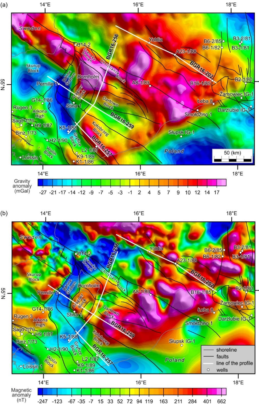
195 Figure 3. Gravity and magnetic anomaly maps. Location of main faults and tectonic blocks (modified from Kramarska et al. (1999), Krzywiec et al. (2003), Jaworowski et al. (2010), Pokorski (2010), Seidel et al. (2018) and Ponikowska et al. (2024)) overlaid
