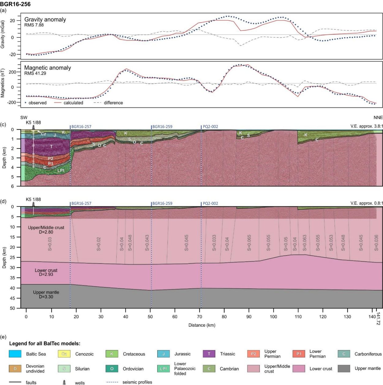
415 Figure 6. Two-dimensional gravity and magnetic model for the BGR16-256 profile. (a, b) Gravity and magnetic data, respectively. (c) Vertically exaggerated (3.8:1) upper part of the geological model. (d) Full geological model at the scale 0.8:1. Numbers indicate densities (D) in g/cm 3 and susceptibilities (S) in SI convention. Thin grey lines show the boundaries of blocks that differ in magnetic susceptibility.
