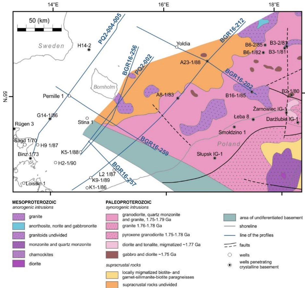
Figure 11. Geological map of the crystalline basement of the East European Craton in the area of interest (modified from Zemnińska et al., 2017 ).
