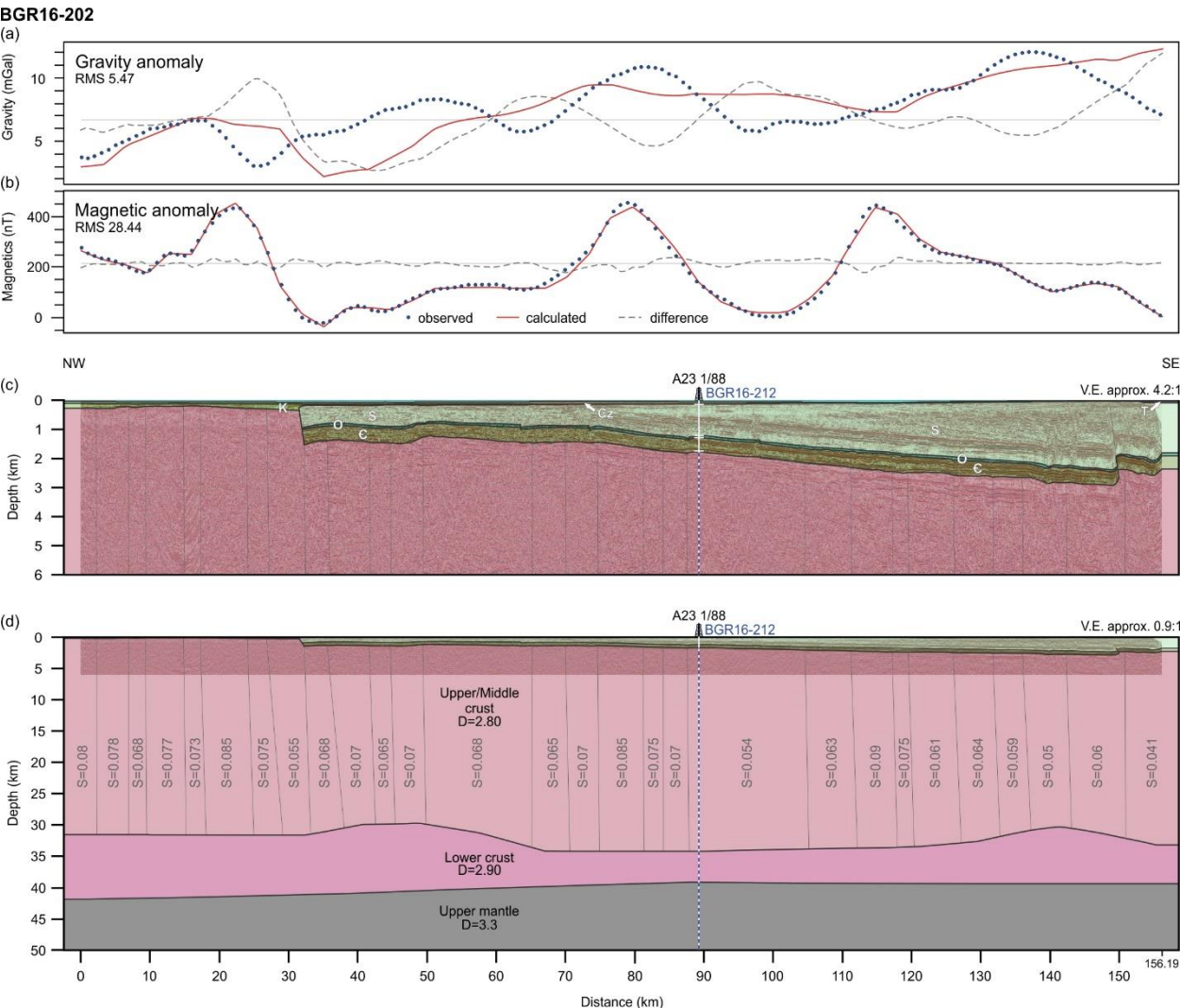
Figure 7. Two-dimensional gravity and magnetic model for the BGR16-202 profile. (a, b) Gravity and magnetic data, respectively. Blue, dotted lines – observed and red, solid lines – modelled. Grey, dashed line shows the magnitude of error. (c) Vertically exaggerated (4.2:1) upper part of the geological model. (d) Full geological model at the scale 0.9:1. Numbers indicate densities (D) in g/cm 3 and susceptibilities (S) in SI convention. Thin grey lines show the boundaries of blocks that differ only in magnetic susceptibility.
