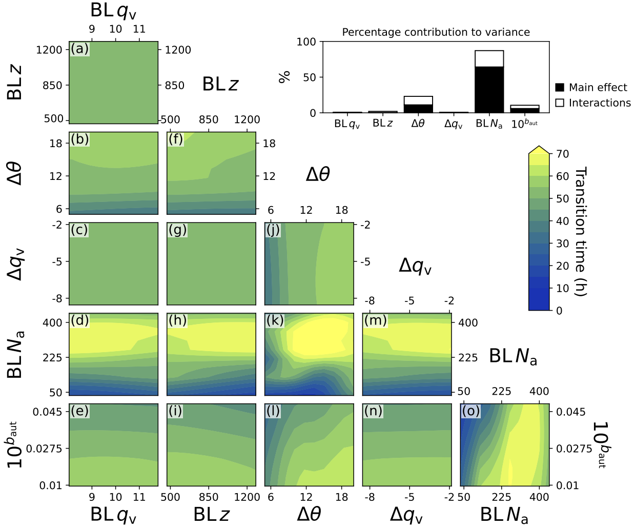
Figure 8. Averaged transition time response surface. The transition time emulator was sampled 1-million times using a 6-dimensional grid and a-o) shows each 2-dimensional combination of the six perturbed factors averaged through the remaining 4 dimensions not shown in that panel. The inset in the top right shows the contribution of each parameter’s variance to the variance in the transition time.
