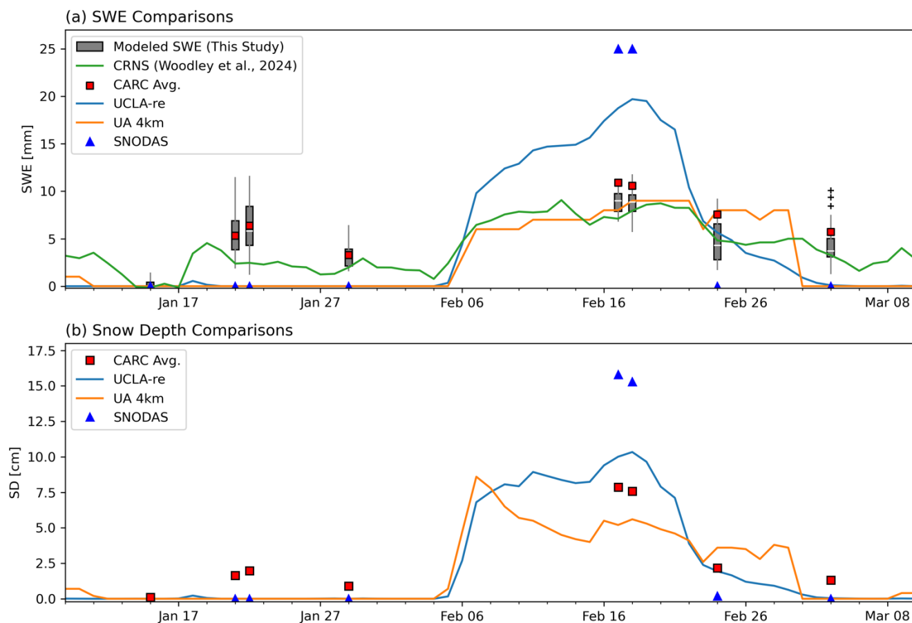
Figure 85 Comparisons of (a) SWE estimates and (b) snow depth estimates from gridded products and in situ measurements between 9 January to 10 March 2021. In (a), time series of the UCLA Snow Reanalysis (blue line), UA SWE (orange line), daily mean CRNS SWE (green line) from Woodley et al., (2024; blue line from Fig. 5a) are shown. Daily SNODAS SWE estimates for each of the dates corresponding to a lidar flight are shown as blue triangles, and an averaged CARC SWE for each digital snow model (DSM) for the 1 km 2 study region are plotted as red squares. URANOS modelled SWE estimates from this study for each date are plotted as grey boxplots to illustrate the variability of SWE within our study region. Snow depth from the same sources are shown in (b), except for CRNS and URANOS, which do not estimate snow depth.
