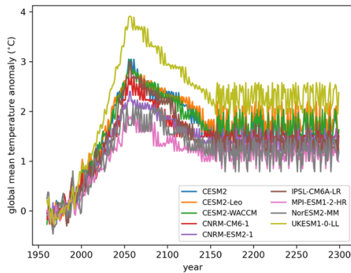
561 562 Figure C1. Illustration of the construction of schematic overshoot scenarios mimicking SSP5-3.4-OS. To construct the forcing, SMB and 563 retreat forcing are drawn from existing annual forcing files (not shown). Instead, the figure shows the sequence of global mean temperature 564 anomaly drawn from each individual original ESM temperature time series.
