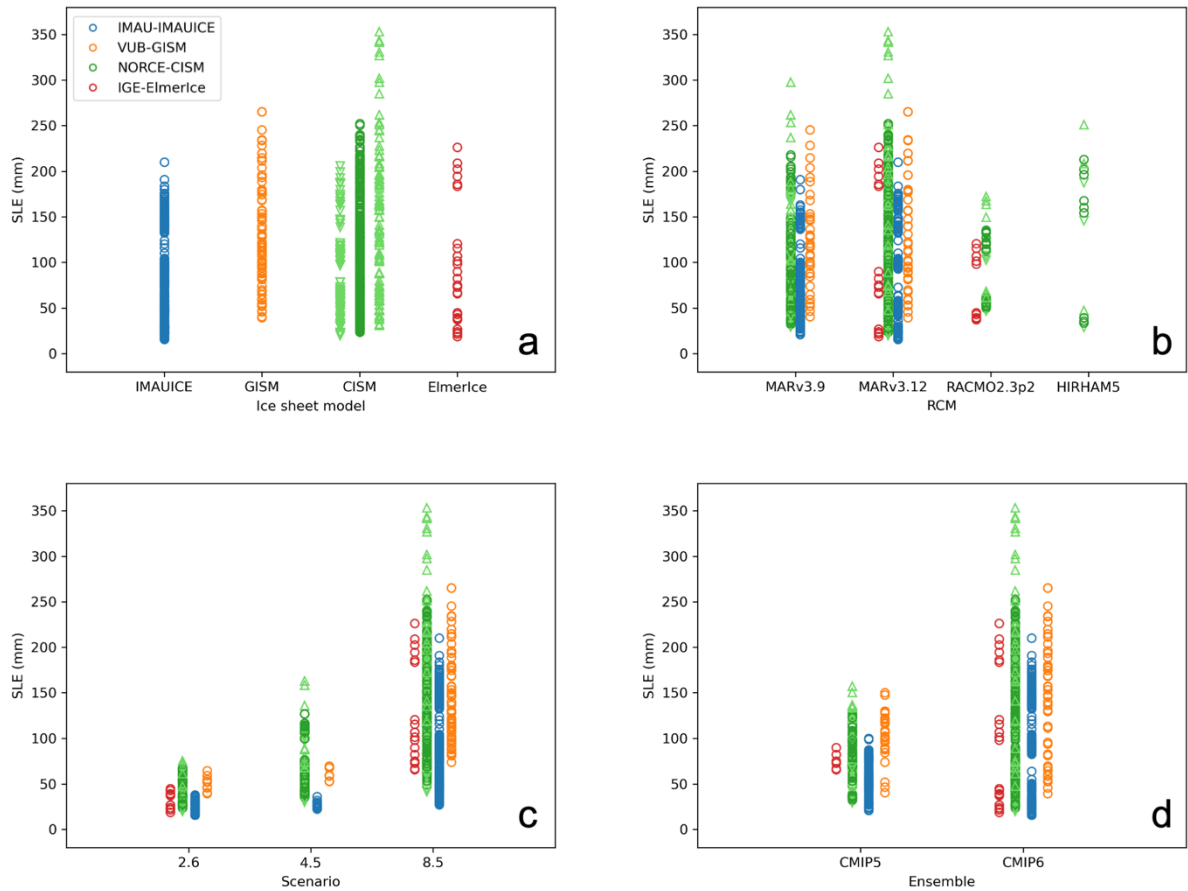
344 Figure 7. Sea-level contribution by year 2100 from the GrIS sorted by a) ice sheet model, b) regional climate model, c) scenario and d) 345 CMIP ensemble. The colour legend is the same for all panels. Scenarios labelled ‘2.6’ in c) include SSP1-2.6 and RCP2.6 and ‘8.5’ includes 346 SSP5-8.5 and RCP8.5. Triangular light green markers for NORCE-CISM indicate experiments with extreme values of the retreat parameter 347 \kappa in the 5 th percentile (upward-pointing) and 95 th percentile (downward-pointing). 348
