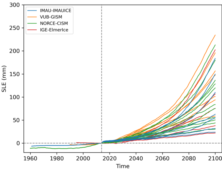
312 313 Figure 5. Projected sea-level contribution from the GrIS until 2100 from a subset of experiments with all four participating ice sheet models 314 (one model version per group), median retreat sensitivity and forcings produced specifically for PROTECT (MARv3.12, RACMO2.3p2, 315 HIRHAM5). The aim of this figure is to illustrate the range and distribution of the projections, not individual members.
