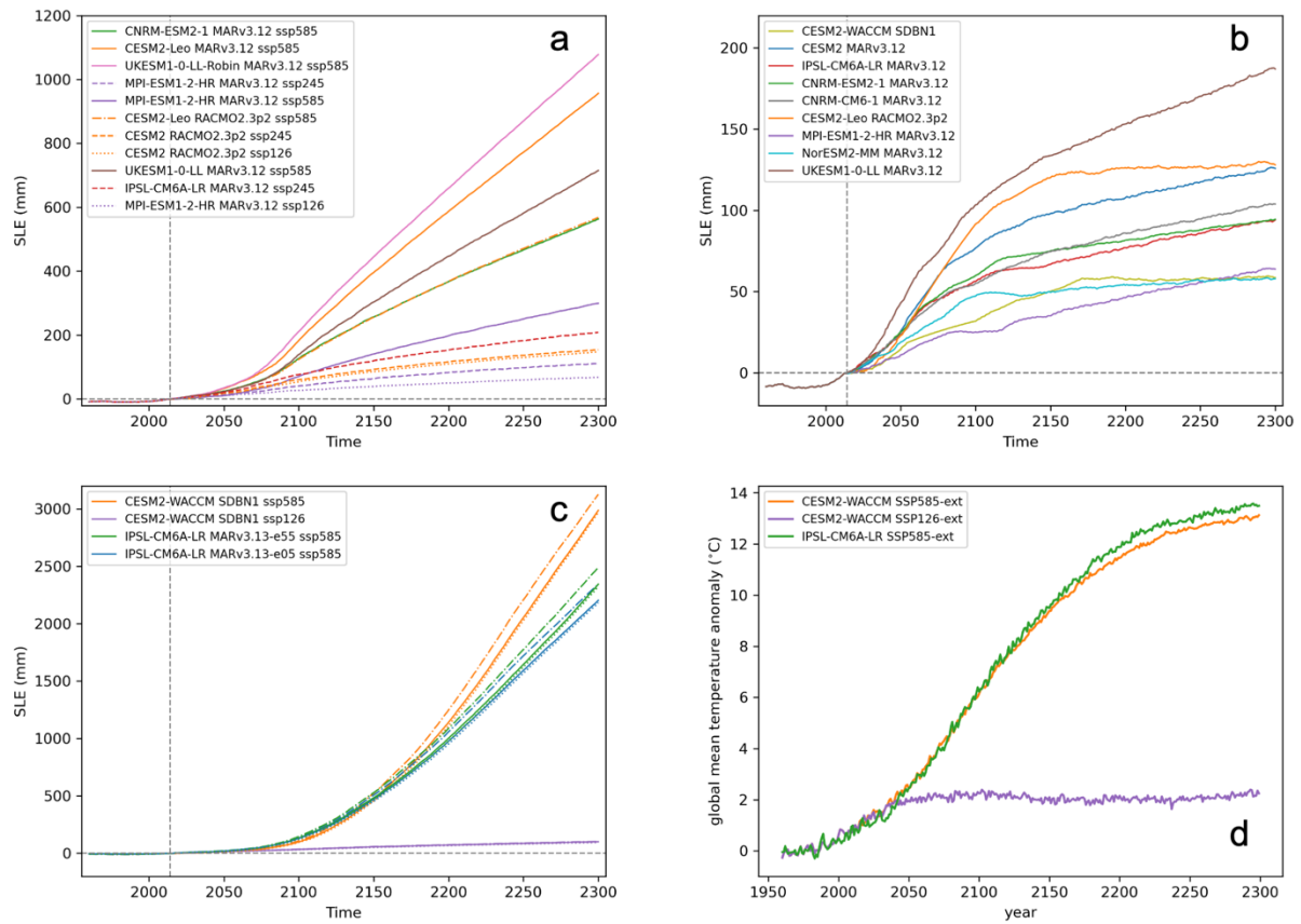
Figure 8. Extensions to 2300 with NORCE-CISM for various ESMs/RCMs with median values of retreat parameter \kappa for a) repeated forcing after 2100 and b) overshoot scenario mimicking SSP5-3.4-OS. c) Natural extensions with CMIP6 forcing until 2300 with median (solid), high(dot-dashed) and low (dotted) values of retreat parameter \kappa . For scenario SSP1-2.6, experiments with various values for \kappa are largely overlapping and difficult to distinguish. Extensions to 2200 are overlapping with the respective continuations to 2300 and are not shown. d) ESM global mean temperature anomaly relative to 1960-1989 for the experiments in c.
