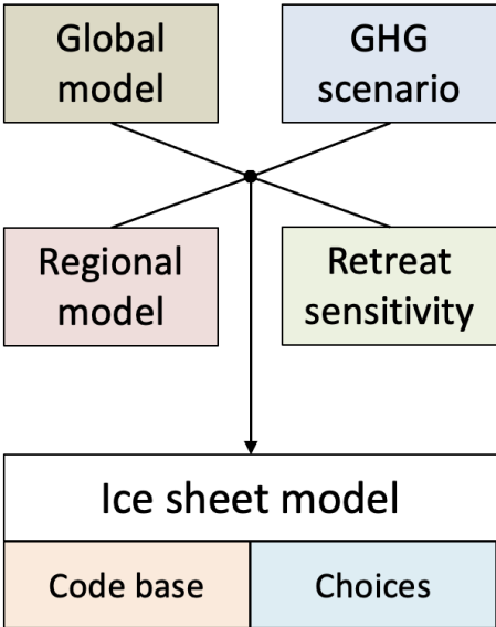
299 300 Figure 4. Forcing and model options relevant for the larger ensemble design.
