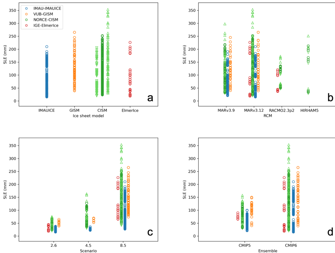
350 351 Figure 7. Sea-level contribution by year 2100 from the GrIS sorted by a) ice sheet model, b) regional climate model, c) scenario and d) 352 CMIP ensemble. The colour legend is the same for all panels. Scenarios labelled ‘2.6’ in c) include SSP1-2.6 and RCP2.6 and ‘8.5’ includes 353 SSP5-8.5 and RCP8.5. Triangular light green markers for NORCE-CISM indicate experiments with extreme values of the retreat parameter 354 kappa in the 5 th percentile (upward-pointing) and 95 th percentile (downward-pointing).
