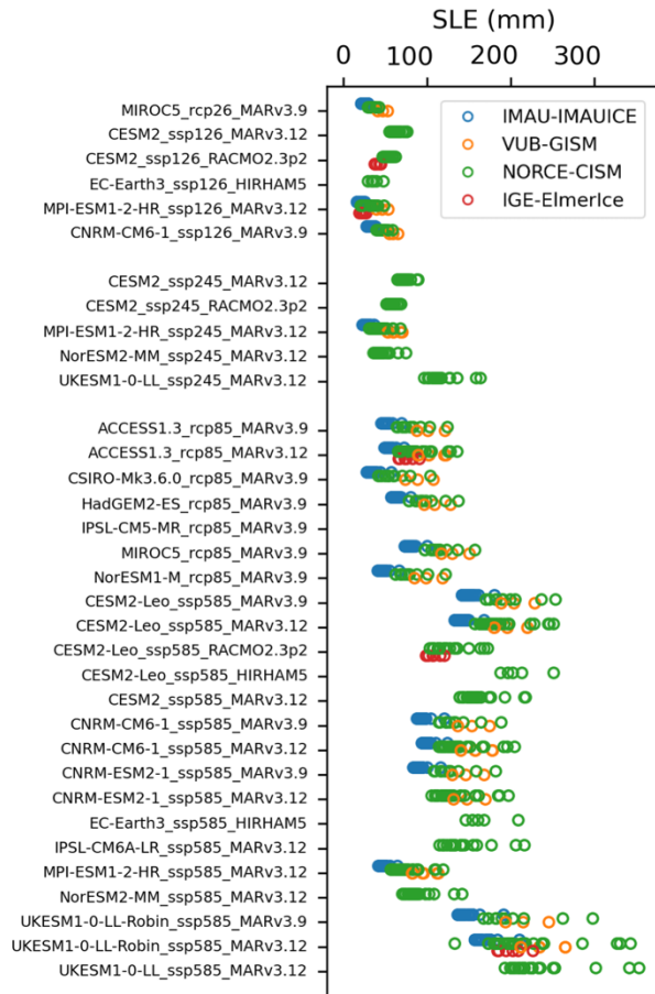
Figure 6. Overview of produced GrIS sea-level projections for the year 2100 from 4 ice sheet models (23 different model versions) and 5 retreat sensitivities (med, high, low, p95, p05).
