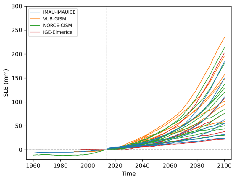
Figure 5. Projected sea-level contribution from the GrIS until 2100 from the four participating ice sheet models (one model version per group), median retreat sensitivity and forcings produced specifically for PROTECT (MARv3.12, RACMO2.3p2, HIRHAM5). The aim of this figure is to illustrate the range and distribution of the projections, not individual members.
