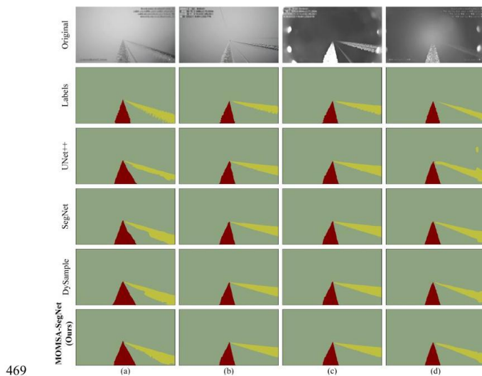
469 470 Figure 13. Comparison of segmentation performance across different models. (a) Segmentation result under daytime conditions 471 (first image), (b) Segmentation result under daytime conditions (second image), (c) Segmentation result under nighttime conditions 472 (first image), and (d) Segmentation result under nighttime conditions (second image).
