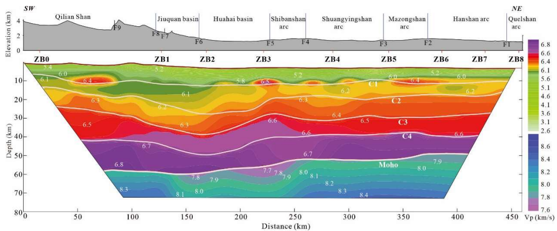
509 Fig. 5 2-D crustal-upper mantle velocity structure. Upper section: topography showing main 510 tectonic units; lower section: crustal-upper mantle velocity structure. White solid lines denote the 511 main interfaces resolved from wide-angle reflections. 512
