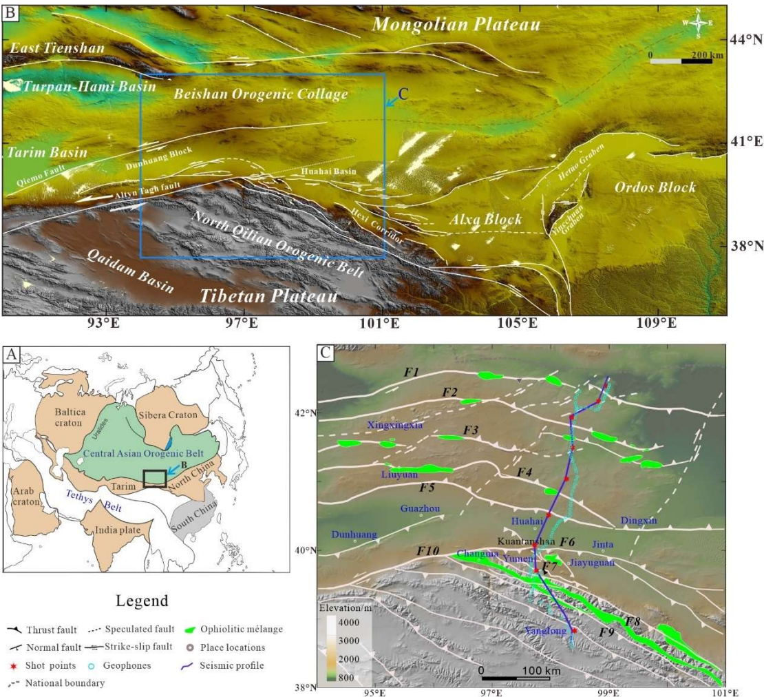
Fig. 1 (a) Simplified tectonic framework of East Asia, emphasizing the CAO and the Tethys tectonic belt (modified after Xiao et al. 2017). (b) Map of the distribution of fault system in the NE
