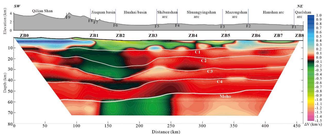
513 Fig. 6 2-D crustal- upper mantle velocity anomaly structure (layer means subtracted from 514 velocities shown in Fig. 5). Upper section: topography showing the main tectonic units; lower 515 section: crustal-upper mantle velocity anomaly structure. White solid lines denote the main 516 interfaces resolved from wide-angle reflections. 517
