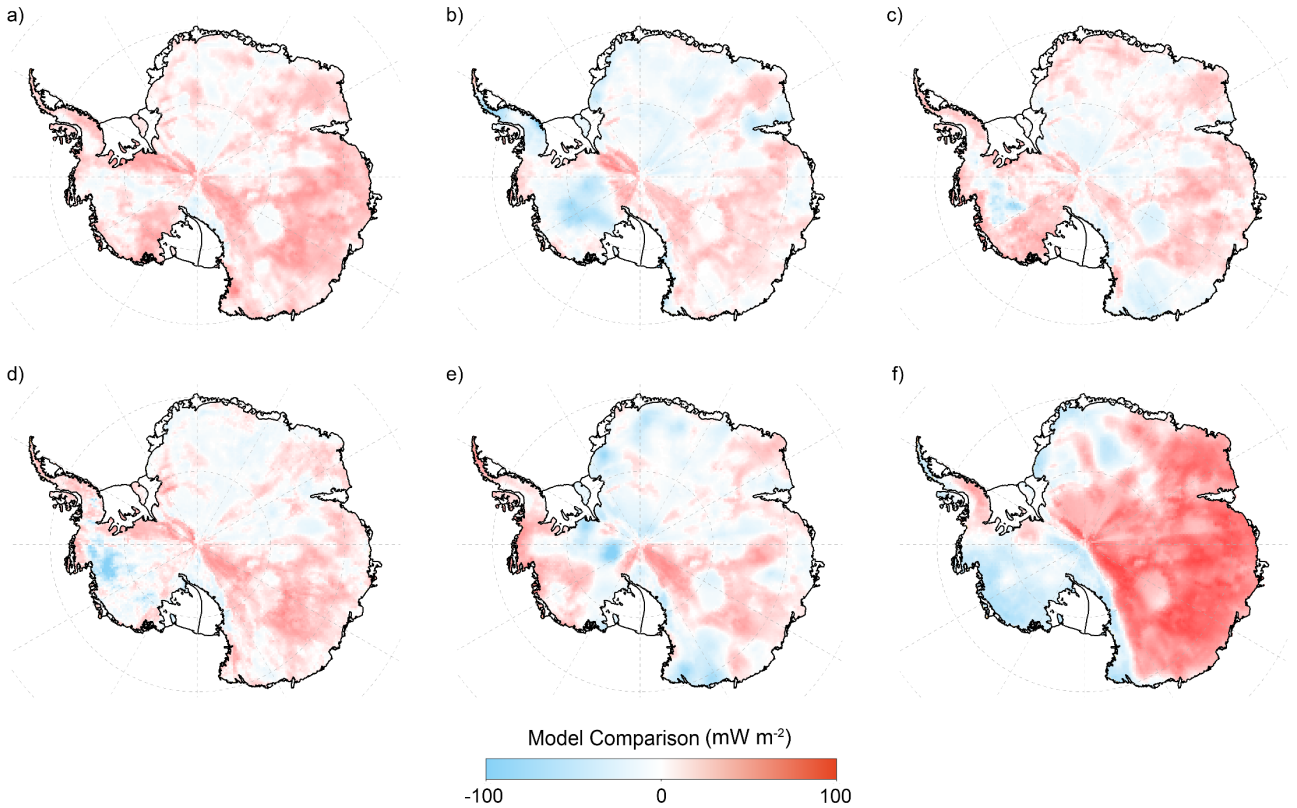
Figure 7. Spatial differences between our GHF predictions and six previously published models. a) Ours – Shen et al. (2020). (b) Ours - Martos et al. (2017). (c) Ours - Lösing et al. (2021). (d) Ours – Stål et al. (2020). E) Ours - Fox Maule et al. (2017). (f) Ours – Hazzard and Richards, (2024). The maps are generated using the Antarctic Ice Shelf and Antarctic Coastline map of Mouginot et al. (2017) as a base map to define the continental extent and grounding line boundaries.
