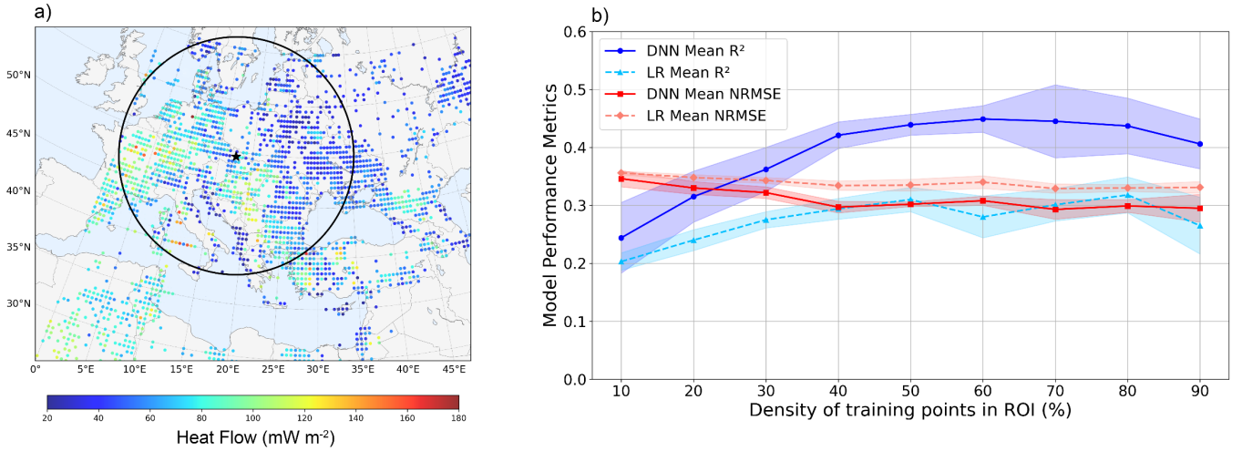
360 Figure 5. Performance of DNN and linear regression methods in experiments with different densities of ROI regions. (a). Test region where the black circle represents the ROI with maximum data density. (b). Performance comparison of DNN and linear regression under different training densities.
