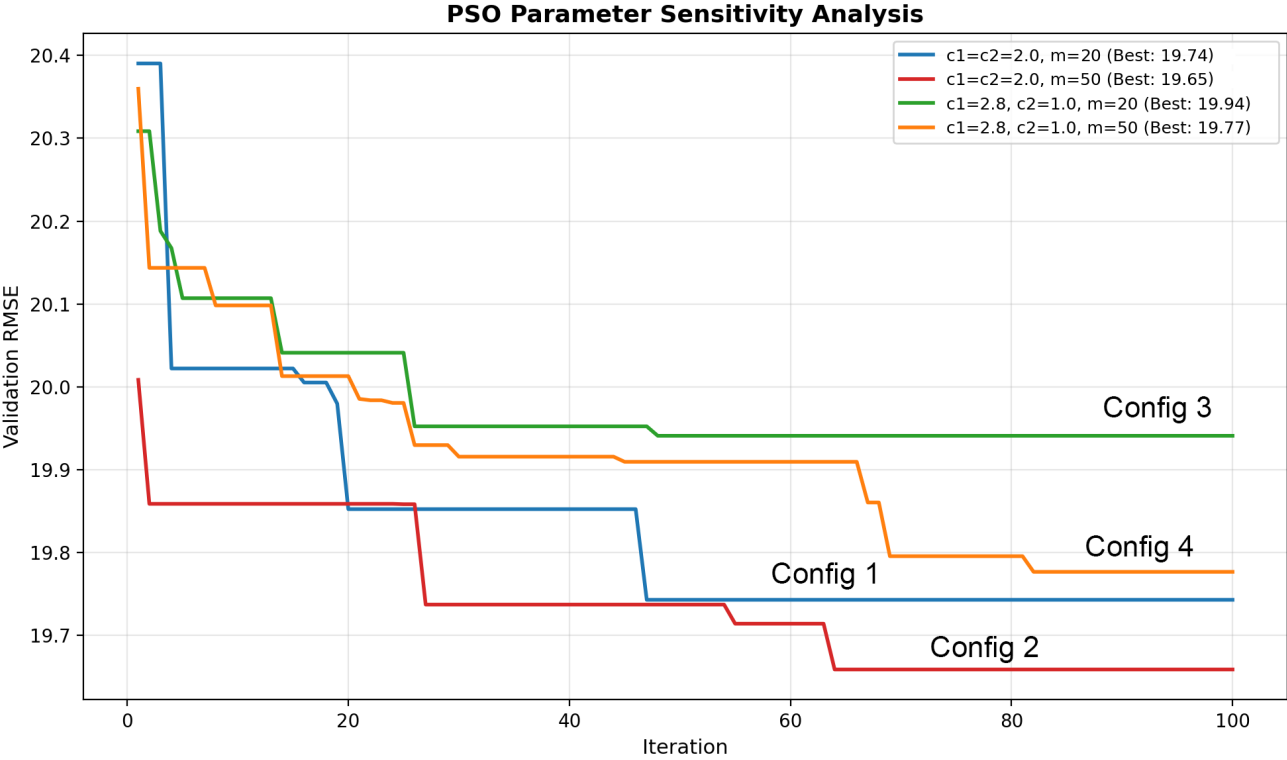
Figure 4. PSO parameter sensitivity analysis showing validation RMSE convergence curves over 100 iterations for four configurations with different acceleration coefficients ( c_1 , c_2 ) and particle numbers ( m ).
