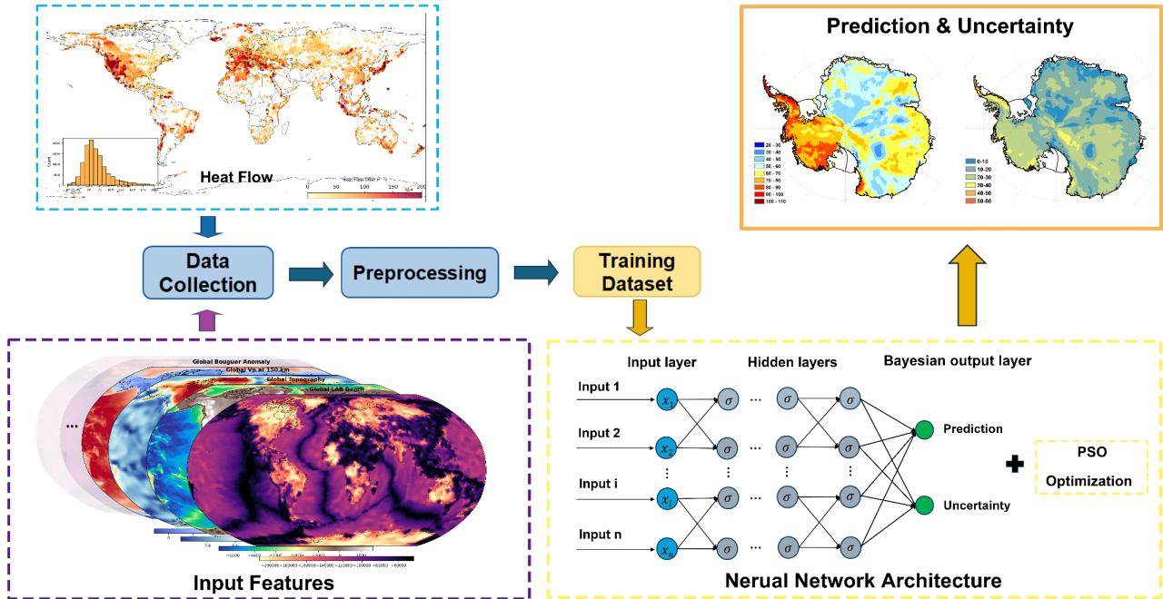
Figure 2. Schematic workflow of the PSO-Bayesian deep neural network framework for Antarctic GHF prediction. The upper-left panel shows global GHF measurements used for training. The lower-left panel displays examples of geophysical input features. The central component illustrates the neural network architecture, consisting of an input layer receiving multiple geophysical variables, hidden layers with optimized depth and width, and an output layer producing GHF predictions. The network hyperparameters are optimized using particle swarm optimization (PSO), while a Bayesian framework enables uncertainty quantification. The upper-right panel presents the final outputs: predicted GHF distribution and associated uncertainty estimates across Antarctica.
