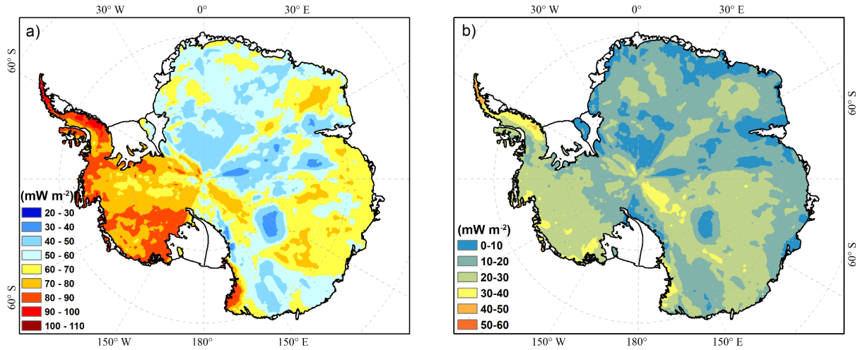
385 Figure 6. Predicted GHF distribution and associated uncertainty across Antarctica. (a) Mean GHF predictions from the five-fold cross-validation ensemble, ranging from 20 to 110 mW m -2 (standard deviation). (b) Total predictive uncertainty derived from the Bayesian framework, ranging from 0 to 60 mW m -2 . Higher uncertainties are generally associated with regions of elevated GHF predictions.
