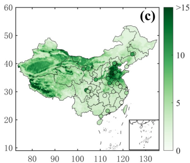
Figure 4. (a) Comparison between CrIS satellite-based column average (from ground to ~1 km) \text{NH}_3 concentration and ground site based (~1.5 m) \text{NH}_3 observations before adjustment; (b) comparison between CrIS satellite-based column average \text{NH}_3 concentration and ground site based \text{NH}_3 observations after adjustment to ground-level; (c) Spatial distribution of adjusted satellite-based \text{NH}_3 concentration and comparisons with ground site based \text{NH}_3 concentrations in 2015 (Unit: ppb), note the adjustment from CrIS satellite-based column average (ground to ~1 km) to ground-level (~1.5 m) is conducted by using the linear regression equation derived from panel a, each scatter plot represents monthly averages of all available observations for either urban or rural site.
