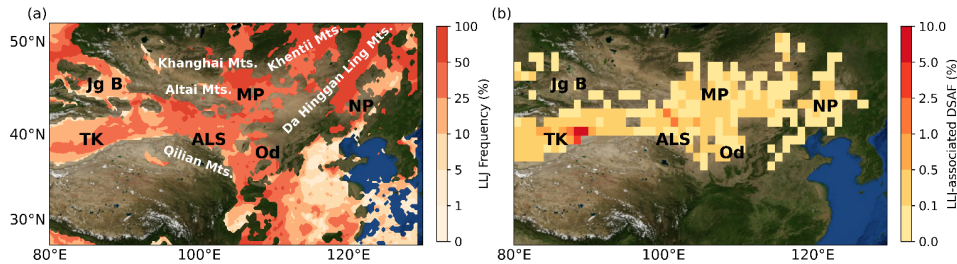
425 Figure 6. (a) Frequency (%) of the Low-level Jet (LLJ, \Delta v \geq 5 m/s between levels at 975 hPa and the jet-nose pressure) occurrence at 06:00 local solar time (LST), average from 2016 to 2023. The LLJ frequency is defined as the number of days with a diagnosed low-level jet divided by the total number of days over the 8-year study period. (b) Summer LLJ-associated dust source activation frequency (DSAF) from 2016 to 2023, quantified as the percentage of clear-sky dust events between 09:00 and 12:00 LST that coincide with a low-level jet at 06:00 LST within the same date, normalised by the total number of summer observation days. High LLJ occurrence and LLJ-associated dust source activations regions labelled in black include Jungger Basin (Jg B), the Mongolian Plateau (MP), the Alashan Plateau (ALS), the Northeast Plain (NP), the Taklimakan Desert (TK), and the Ordos Plateau (Od). Main mountains (Mts.) are labelled in white. Basemap from NASA’s Blue Marble: Shaded Relief imagery © NASA.
