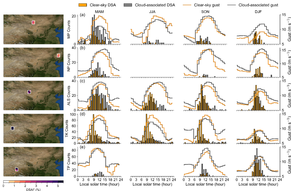
285 Figure 4. Diurnal distributions of dust source activation (DSA) counts for sample localities from the main dust-active regions in East Asia under clear-sky and cloud-associated conditions across the four seasons: spring (March, April, May; MAM), summer (June, July, August; JJA), autumn (September, October, November; SON), and winter (December, January, February; DJF). The main dust-active regions are: (a) the Mongolia Plateau (MP; 103–105°E, 43–45°N), (b) the Northeast 290 Plain (NP; 121–123°E, 43–45°N), (c) the Alashan Plateau (ALS; 100–102°E, 41–43°N), (d) the Taklimakan Desert (TK; 89– 91°E, 39–41°N), and (e) the Tibetan Plateau (TP; 91–93°E, 34–36°N). For each region, the grids with the highest dust source activations frequency (see maps on the left) are used for the analysis. Bar plots represent the hourly counts of DSA events for each season, while the overlaid curves show the corresponding mean diurnal cycle of 10 m wind gust speed on DSA days under clear-sky (yellow) and cloud-associated (grey) conditions. Basemap from NASA’s Blue Marble: Shaded Relief imagery © NASA.
