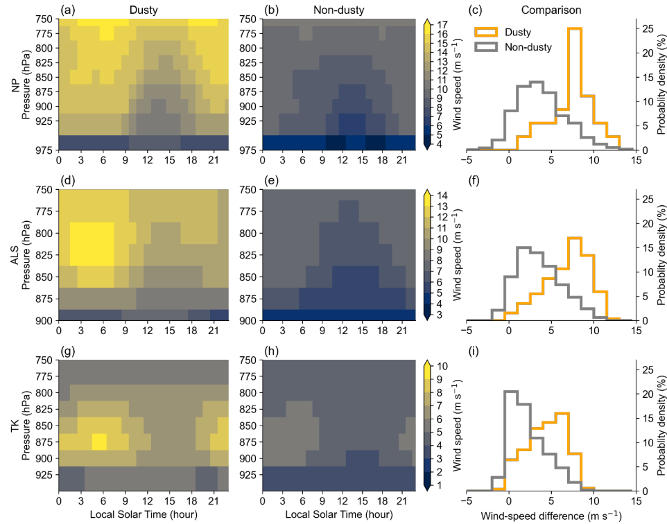
375 Figure 5. Wind speed structure at different pressure levels and times of day for dusty under clear-sky conditions and non- 380 dusty days at different hours for three of the subregions analysed in Fig. 4: (a–b) NP (the Northeast Plain, 121–123°E, 43– 45°N), (d–e) ALS (the Alashan Plateau, 100–102°E, 41–43°N), and (g–h) TK (the Taklimakan Desert, 89–91°E, 39–41°N). The rightmost column shows the wind speed difference between 975 hPa and the jet-nose pressure level at 06:00 LST (i.e., the time when the LLJ typically reaches its maximum intensity and preconditions the atmosphere for dust emission later in the morning) for dusty (yellow) and non-dusty (grey) days in: (c) NP, (f) ALS and (i) TK.
