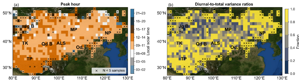
Figure 3. Peak hours of dust source activation and diurnal variance dominance across East Asia (80°E–130°E, 27°N–52°N). (a) Peak hour of dust occurrence expressed in local solar time (LST) using 3-hour bins, derived from the timing distribution of dust activation at each grid cell. (b) The proportion of diurnal-to-total variance was defined as the fraction of total temporal variance explained by the hour-of-day term in a two-factor ANOVA decomposition, where the diurnal variance is given by the hour-of-day sum of squares and the total variance by the total temporal sum of squares. Higher values indicate stronger control of dust activation timing by the diurnal cycle relative to seasonal and interaction components. Basemap imagery from NASA’s Blue Marble: Shaded Relief (© NASA).
