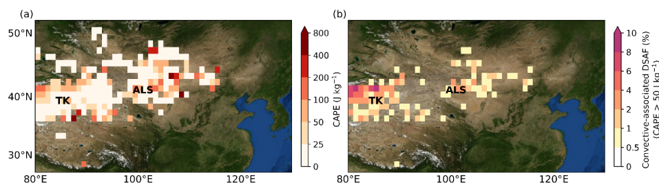
Figure 8. (a) Summer (June–August) convective available potential energy (CAPE) at 12:00 LST, shown as a 9-gridcell ( 3^\circ \times 3^\circ ) mean centred on each 1^\circ grid cell and averaged over days of cloud-associated summer afternoon (15:00–18:00 LST) 490 dust source activations. (b) Convective-associated dust source activation frequency (DSAF), estimated as the percentage of summer days (June–August) with dust source activation events observed between 15:00 and 18:00 LST under cloud- associated convective conditions (CAPE at 12:00 LST > 50 \text{ J kg}^{-1} ) from 2016 to 2023, normalised by the total number of summer observation days. Regions with high convective-associated DSA frequency are labelled in black, including the Alashan Plateau (ALS) and the Taklimakan Desert (TK). Basemap from NASA’s Blue Marble: Shaded Relief imagery © 495 NASA.
