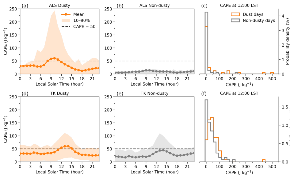
Figure 7. Mean diurnal evolution of convective available potential energy (CAPE) for dusty (under summer cloud-associated conditions during 15:00–18:00 LST) and non-dusty days over two subregions: (a–b) ALS (the Alashan Plateau, 100–102°E, 41–43°N) and (d–e) TK (the Taklimakan Desert, 83–85°E, 40–42°N). Shading indicates the 10th–90th percentile range. The dashed horizontal line marks the CAPE threshold of 50 \text{ J kg}^{-1} . Panels (c,f) present the probability distributions of CAPE at 12:00 LST for dusty (orange) and non-dusty (grey) days over ALS and TK, respectively. All CAPE values are spatially averaged over a 3^\circ \times 3^\circ grid (nine grid cells, \pm 1^\circ grid) centred on each subregion to account for the spatial offsets that commonly occur between haboob events and associated convective clouds.
