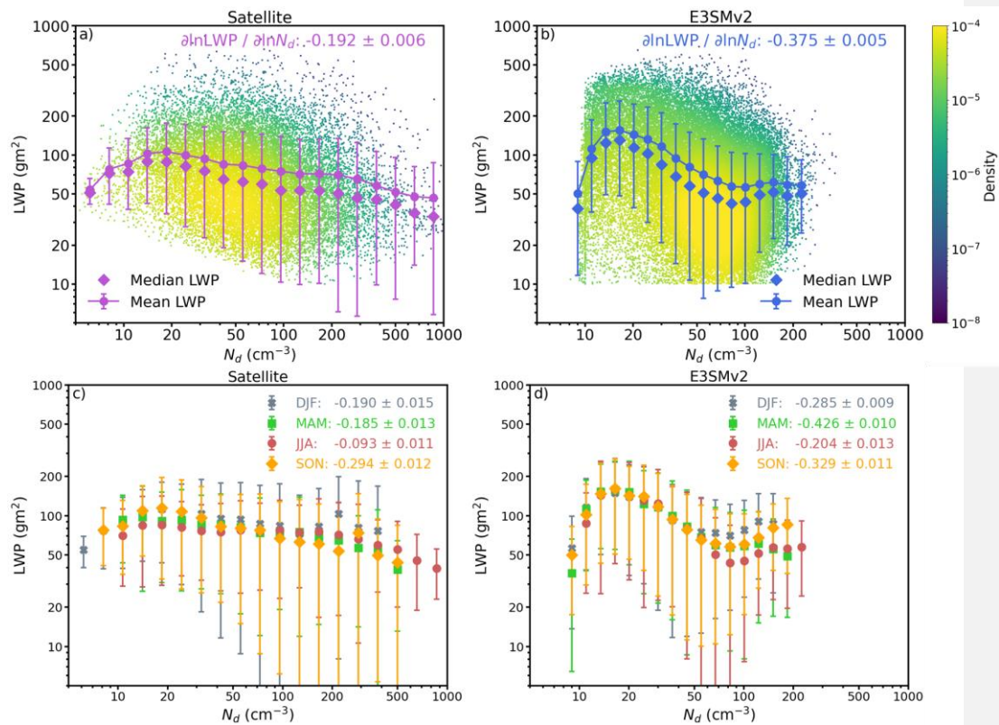
Figure 2. Top Panel: Bulk LWP binned as a function of N_d from a) satellite and b) E3SMv2, the Gaussian kernel density estimate (KDE) is shown as color-shaded scatter points area. The mean (median) LWP values in N_d bins are shown as solid-dotted lines (diamond symbols); Bottom panel: seasonality of the LWP dependences from c) satellite and d) E3SMv2, with colored symbols denote mean LWP in N_d bins. Error bars denote standard deviations of LWP in N_d bins. Slopes are ordinary least squares fits of \partial \ln(LWP) / \partial \ln(N_d) , and ‘ \pm ’ values are standard errors of the fitted slopes.
