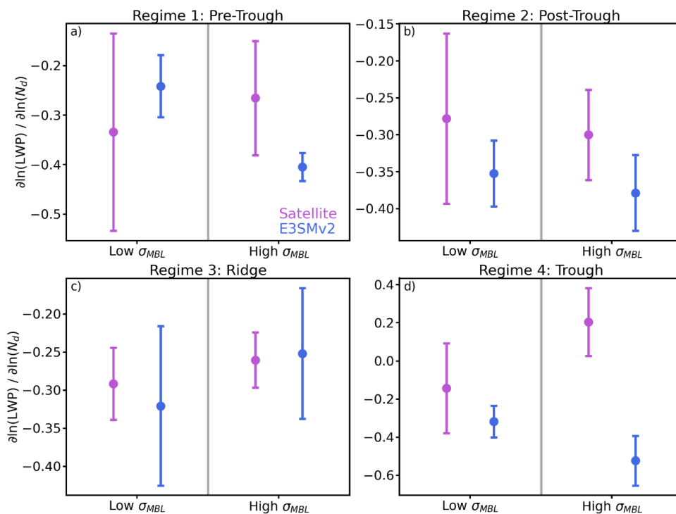
Figure 9. LWP adjustment due to N_d under low and high \sigma_{MBL} categories, separated by the median \sigma_{MBL} values (gray line) from the aggregate satellite (purple) and E3SMv2 (blue) dataset. For a) Regime 1; b) Regime 2; c) Regime 3; d) Regime 4. Error bars denote standard errors of fitted slopes in each category.
