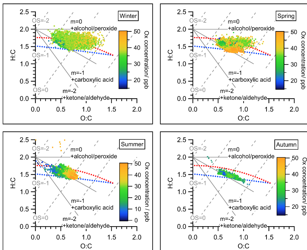
258 Figure 2: Van Krevelen triangle graph for all measurements of organic aerosol during the four seasons of 259 the JULIAC campaign. Atomic ratio regions of standard groups for alcohol/peroxide, carboxylic acid, 260 and ketone/aldehyde (Aiken et al., 2007) were marked as references. The dots in all graphs were color- 261 coded by the concentration of the oxidant Ox (NO 2 +O 3 ) to represent the intensity of secondary oxidation.
