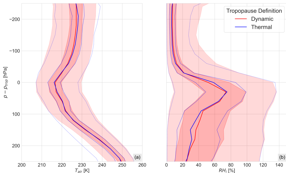
Figure B1. Vertical distribution of a) temperature and b) RH i for dynamic and thermal tropopause definitions using all considered IAGOS measurements in this study. Solid lines indicate mean values; dashed blue line and dark red shade indicate the 25 and 75% percentiles at the thermal and dynamical tropopause, respectively; similarly, dotted blue line and light red shade indicate the 1 and 99% percentiles.
