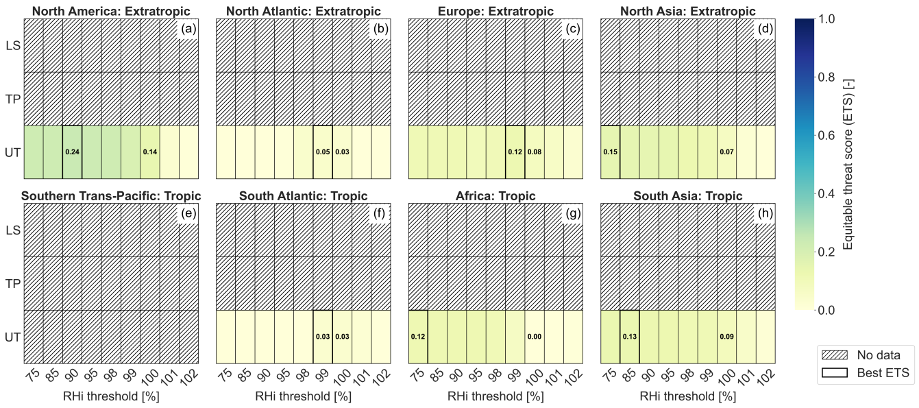
Figure 13. (a–h) Ice supersaturated region equitable threat score under cloudy conditions for different ERA5 RHi thresholds in the upper troposphere (UT), tropopause (TP) and the lower stratosphere (LS). The different conditions have been matched between IAGOS and ERA5. Only combinations with 250+ samples are considered. For each layer, we highlight the ETS for a threshold of 100% and the ETS for the threshold at which we find the maximum value.
