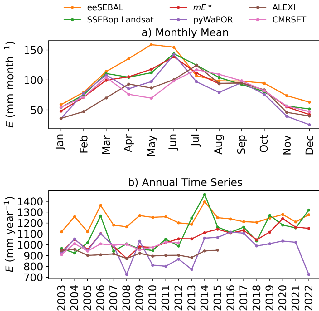
1065 Fig C2: Comparison of the posterior mean ( mE^* ) to the prior data sets describing the evaporation ( E ) variable in the Hindon basin, the top panel depicts (a) monthly mean E , and the bottom panel (b) shows the annual E time series.
