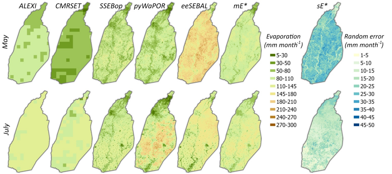
Figure 6: Prior observations and estimated posteriors of grid-scale evaporation E before the monsoon (May 2009) and for a peak rainy month (July 2009); mE^* and sE^* denote the posterior mean and standard deviation of evaporation.
