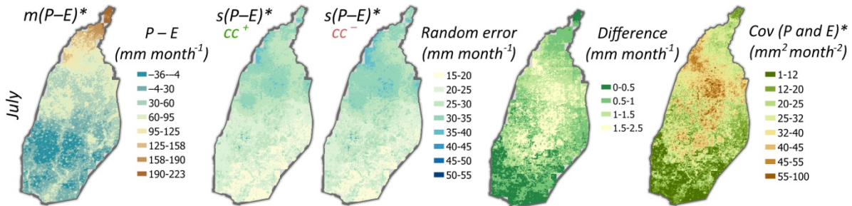
550 Figure 8: Grid-scale posterior mean m_{P-E}^* and standard deviation s_{P-E}^* of P - E , and P and E covariance for July 2009. The posterior standard deviations are computed for the two cases: with ( cc^+ ) and without ( cc^- ) accounting for posterior cross-correlations ( cc ) between P and E , while the difference cc^- - cc^+ between these two cases illustrates the impact of accounting for cross-correlations.
