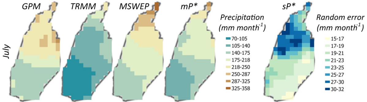
Figure 7: Prior observations and estimated posteriors of grid-scale precipitation P for the peak rainy month (July 2009); mP^* and sP^* denote the posterior mean and standard deviation of precipitation.
