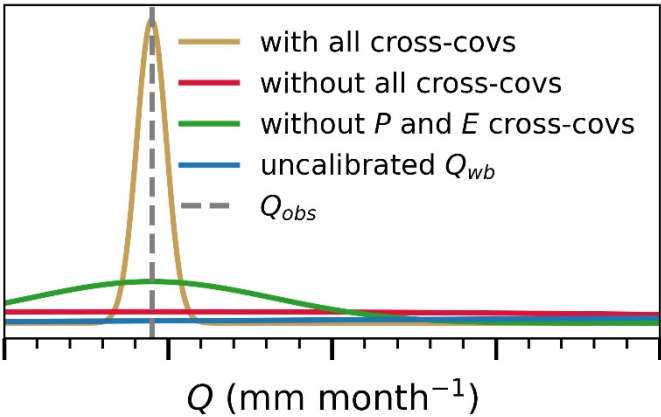
560 Figure 9: Distribution of Q in comparison to the observed Q_{obs} value (July 2009), for the following cases: (i) ignoring and accounting for posterior correlations between all water balance variables, (ii) ignoring only the posterior correlation between P and E , and (iii) Q_{wb} obtained from uncalibrated water balance data. The labels and tick marks are not shown due to data sharing restrictions.
