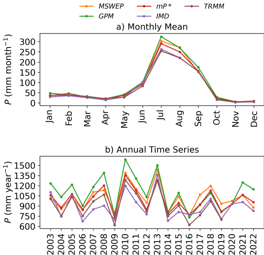
1060 Fig C1: Comparison of posterior mean ( mP^* ) to the prior data sets describing the precipitation ( P ) variable in the Hindon basin, the top panel depicts (a) monthly mean P , and the bottom panel (b) shows the annual P time series.
