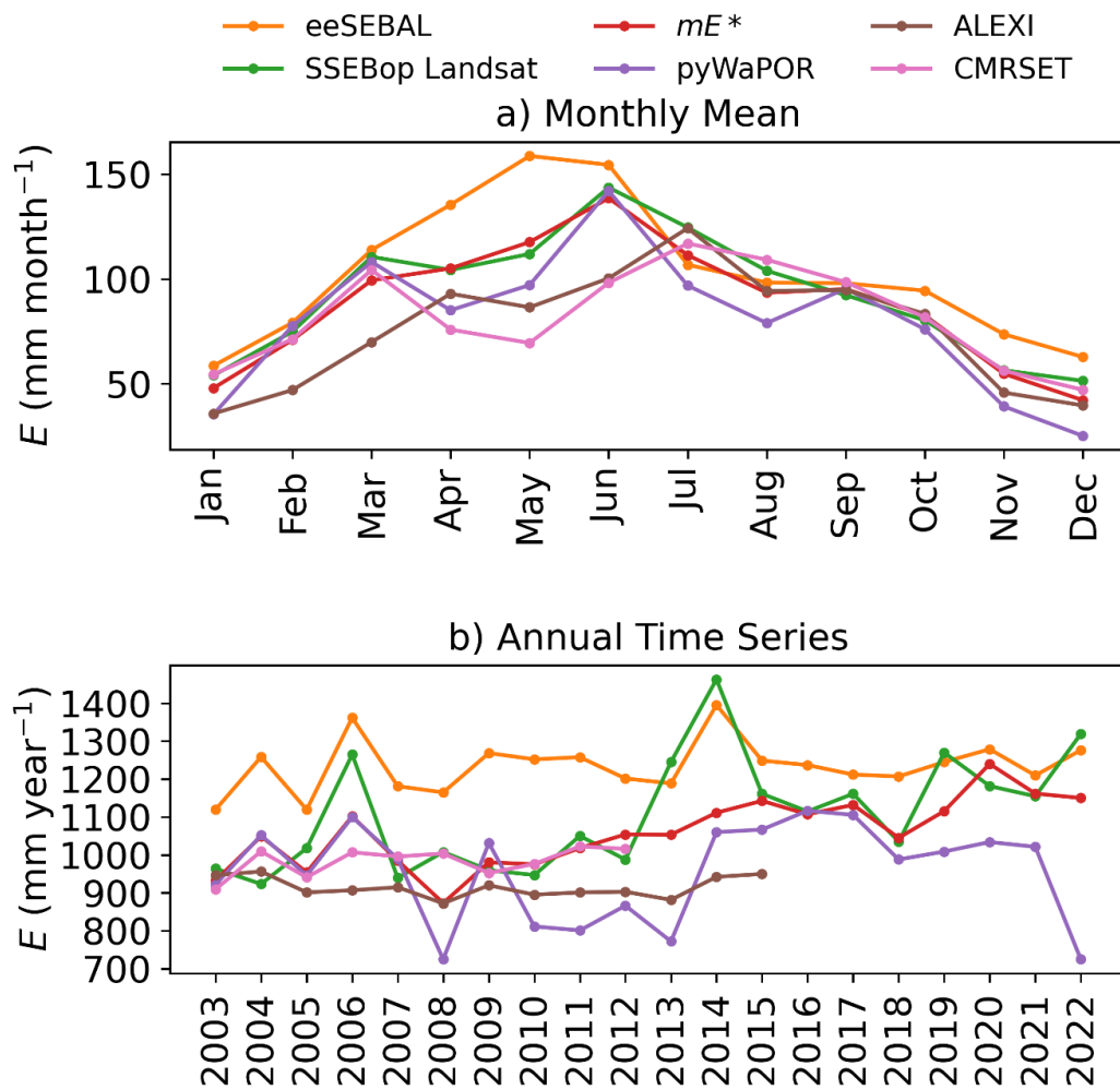
1135 Fig C2: Comparison of the posterior mean ( mE^* ) to the prior data sets describing the evaporation ( E ) variable in the Hindon basin, the top panel depicts (a) monthly mean E , and the bottom panel (b) shows the annual E time series.
