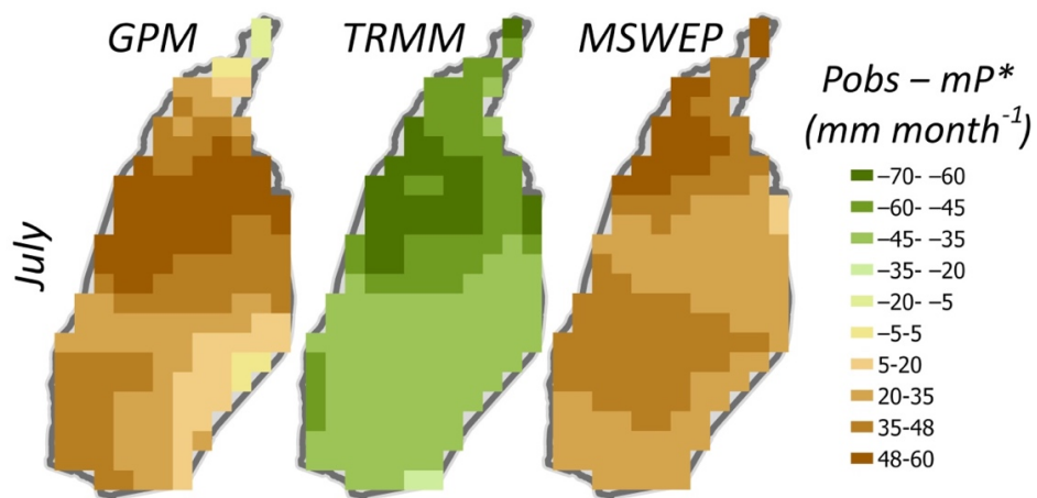
Fig C65: Spatial deviation of the precipitation ( P ) observations from the posterior mean ( P_{obs} - mP^* ) for May and July of 2009.
