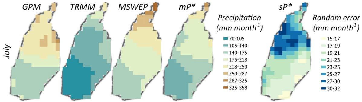
Figure 67: Prior observations and estimated posteriors of grid-scale precipitation P for the peak rainy month (July 2009); mP^* and sP^* denote the posterior mean and standard deviation of precipitation.
