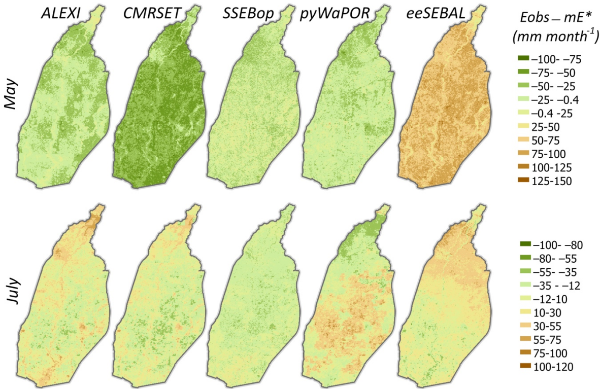
Fig C54: Spatial deviation of the evaporation ( E ) observations from the posterior mean ( E_{obs} - mE^* ) for May and July of 2009.
