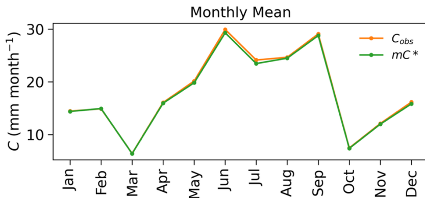
1140 Fig C3: Comparison of the monthly mean posterior mean ( mC^* ) to the prior data describing the surface water imports ( C ) variable in the Hindon basin.
