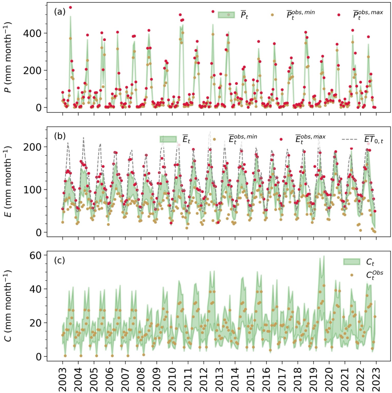
Figure 23: Monthly water balance posteriors (90% credible intervals in green) for: (a) P (precipitation), (b) E (actual evapotranspiration), and (c) C (canal water imports), and their corresponding observations (dots). Reference evapotranspiration computed here using ERA5 meteorological input variables is shown as (ET_0) . The overbars of the labels in P and E plots indicate that these values are obtained through spatial averaging of the gridded data sets for each month t . Each year's label indicates the start of the year (January).
