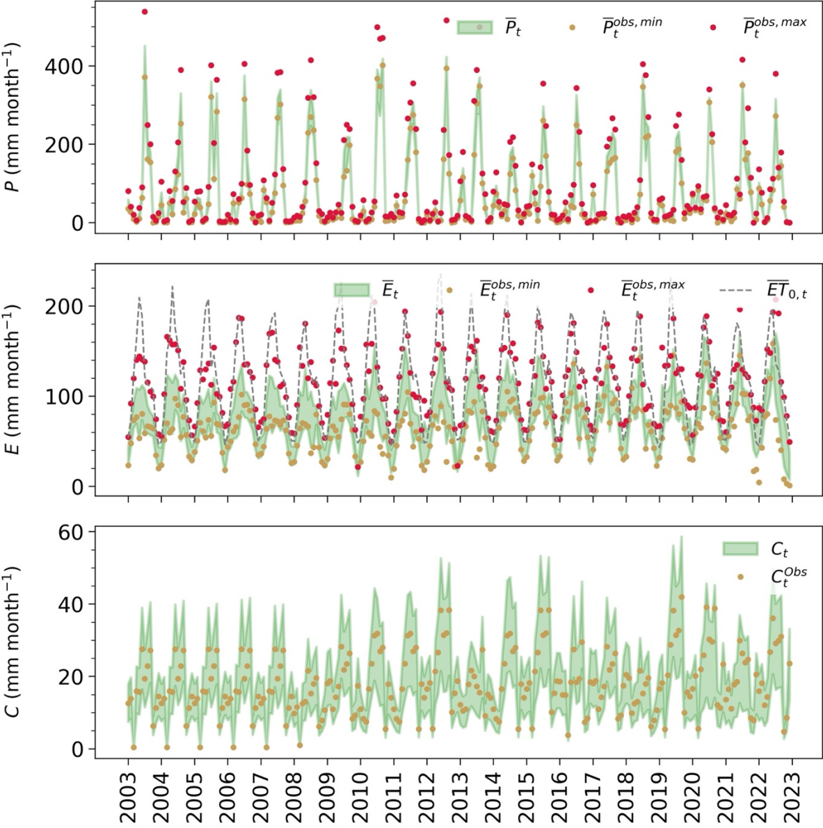
Fig C76: Posterior and prior water balance plots correspond to the case using the GRACE CSR spherical harmonic (SH) solution as an input to the probabilistic water balance model.
