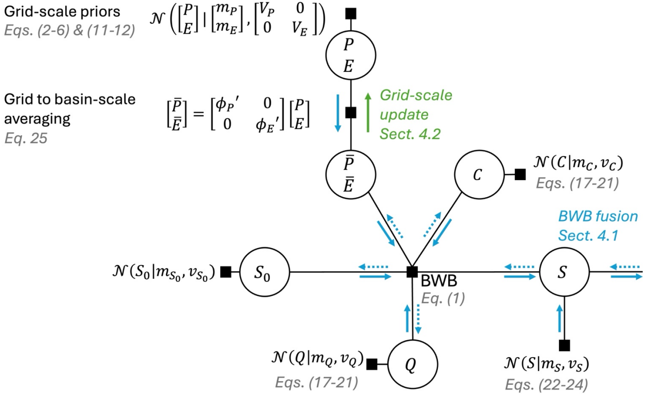
Figure 2: A factor graph showing the random variables in circles and constraints between variables as squares for a single month. Three constraints are incorporated in the water balance data fusion method, including: a prior Gaussian distribution assigned to each water balance variable (squares attached to each variable), the basin-scale water balance (BWB) constraint that links all water balance variables together, and the spatial averaging constraint that links grid-scale precipitation ( P ) and evaporation ( E ) and to basin-scale variables for precipitation ( \bar{P} ) and evaporation ( \bar{E} ). Computation of posteriors of individual variables proceeds in two steps. The first step is basin-scale water balance data fusion (BWB fusion, see Sect. 4.1). This step involves multiple forward (blue arrows along the edges) and backward (dotted blue arrows) passes over the data using the entire timeseries to compute the posteriors of all water balance variables that jointly close the water balance (Schoups and Nasser, 2021). The second step computes grid-scale posteriors for precipitation and evaporation from their basin-scale posteriors using a Kalman smoothing algorithm (green arrow, see Sect. 4.2).
