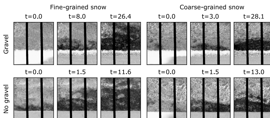
Figure 7. A summary of the 4 experiments showing the 2D optical density images at 3 times (t) given in minutes. The experiments are classified based on their snow type and whether or not they included a gravel layer. These correspond to FG_{s,g} (top left), FC_s (bottom left), CG_{s,g} (top right), and CC_s (bottom right). The vertical black-body bars are shown in black.
