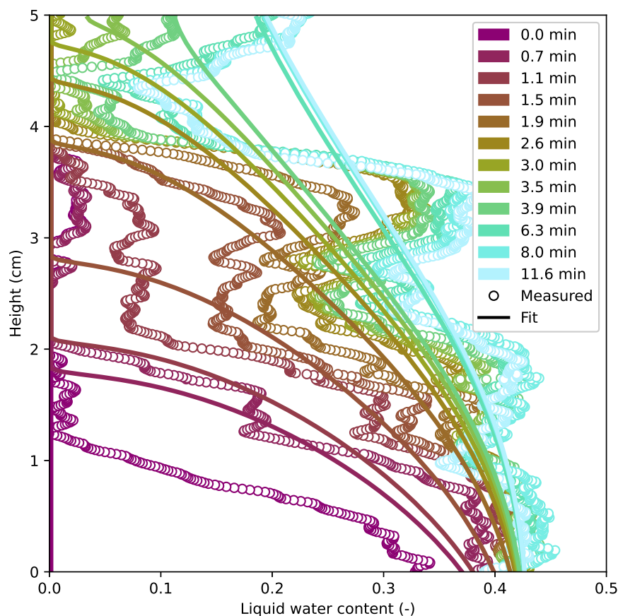
Figure A8. The measured liquid water content profiles and the accompanying inverse fit results for FG_s
