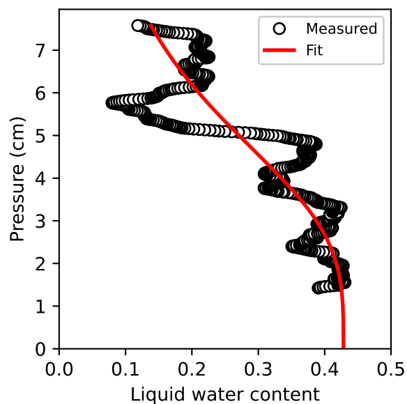
Figure A5. The 1D liquid water content of FG_s as a function of pressure head (black circles) and the fit of these points to Eq. 10 (red line).
