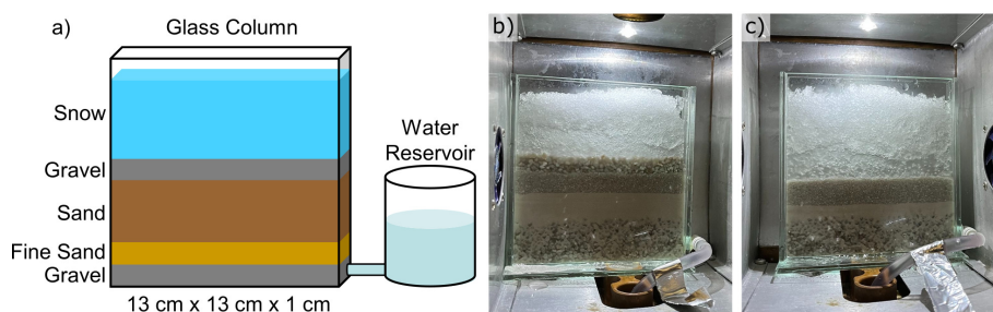
Figure 1. Schematic (a) and photos (b and c) of the column setup. The schematic shows a layering with the transitional gravel layer as does the photo in (c). The photo in (b) is for a layering without gravel. The gravel layer reproduces the effect of the vegetation layer found on grassy slopes.
