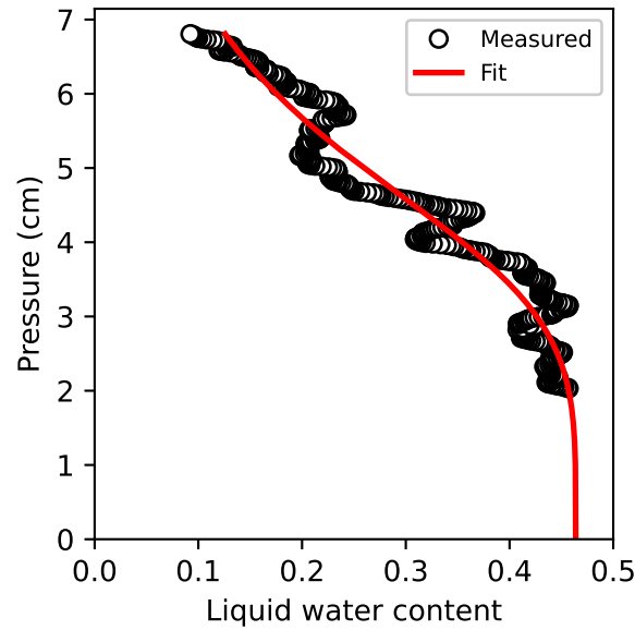
Figure 4. The 1D liquid water content of FG_{s,g} as a function of pressure head (black circles) and the fit of these points to Eq. 10 (red line).
