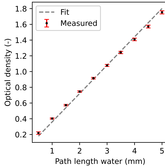
Figure 3. The measured optical density as a function of water thickness or path length (black dots) with error bars of the standard deviation (red) and linear fit (dotted gray line). Fit equation: OD = 0.360(\pm 0.002)z , where z is the path length in mm and OD is the unitless optical density
