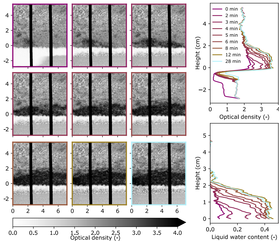
Figure A3. Summary figure of experiment CG s,g showing the 2D optical density evolution over time (left), 1D horizontally averaged optical density profile evolution over time (top right), and 1D horizontally averaged liquid water content profile of the snow over time (bottom right). The 2D images correspond to the times in the vertical profiles (right) as indicated by the color. The units for the optical density images (left) are cm for both axes. For the y-axes of all plots in this figure, a height of 0 cm was defined as the height where the continuous snow phase begins, where the effects of the gravel-snow interface are no longer present. The vertical black-body bars are shown in black in the images (left).
