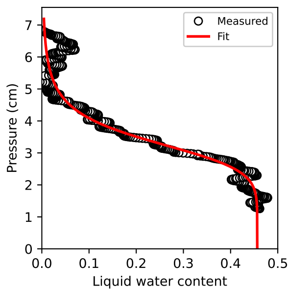
Figure A7. The 1D liquid water content of CG_s as a function of pressure head (black circles) and the fit of these points to Eq. 10 (red line).
