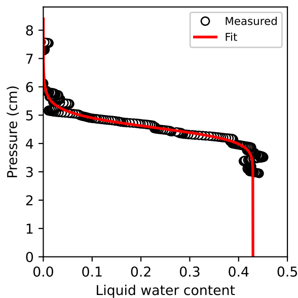
Figure A6. The 1D liquid water content of CG_{s,g} as a function of pressure head (black circles) and the fit of these points to Eq. 10 (red line).
