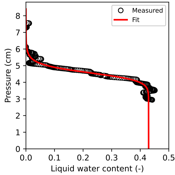
Figure A6. The 1D liquid water content of CG_{s,g} as a function of pressure head (black circles) and the fit of these points to Eq. 10 (red line) with the mean absolute error (MAE) equal to 0.023 and expressed as the volume fraction of liquid water content.
