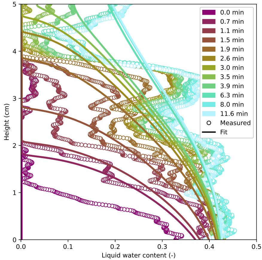
Figure A8. The measured liquid water content profiles and the accompanying inverse fit results for FGs. Note that the small liquid water content values near 4.5 cm caused a large error in the fitting as shown in Fig. A11.
