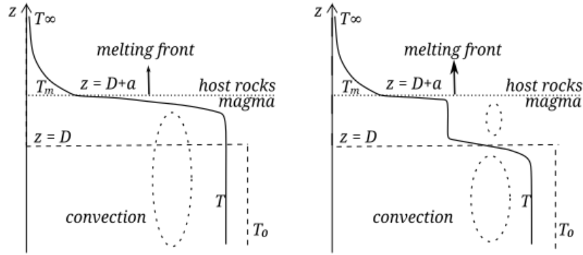
Figure 2. Sketch of geometry and mean temperature profiles, modified after (Huppert and Sparks, 1988): T_o , T_\infty , T_m are initial hot, top, and melt temperatures respectively, D the intrusion thickness and a the molten host rock layer thickness. a) Case of rhyolite intrusion similar to the composition of the host rock (scenario 1), b) Case of basaltic intrusion into rhyolitic host rock (scenario 2).
