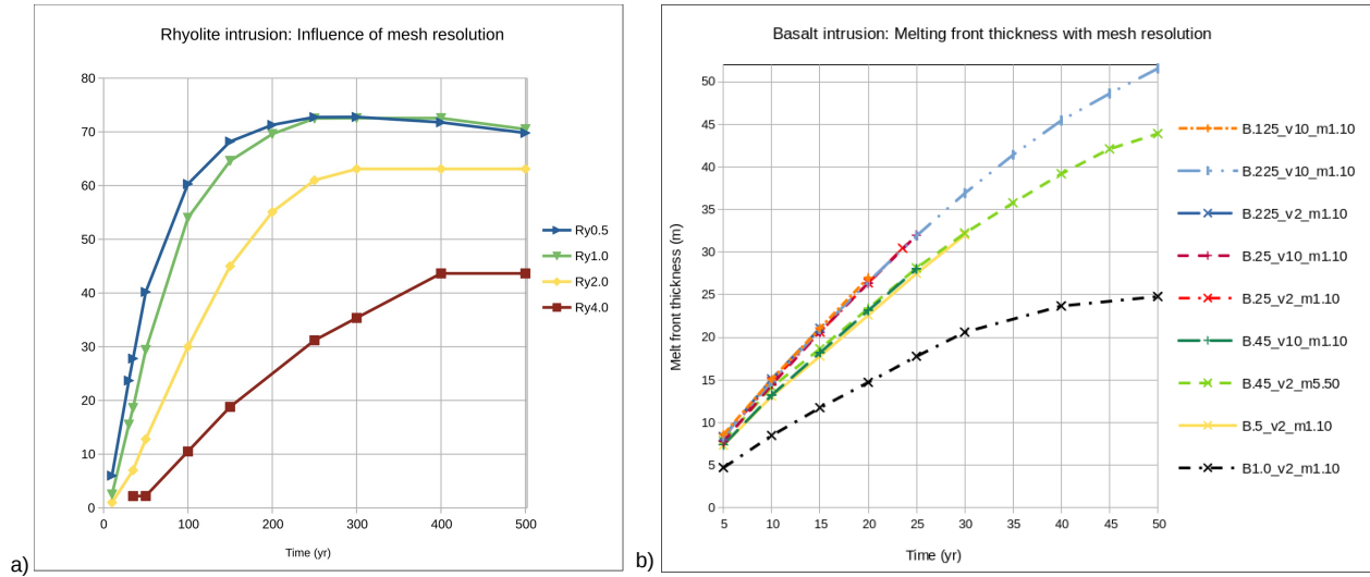
Figure 6. Mesh resolution tests for a) a rhyolite intrusion (scenario 1) and b) a basalt intrusion (scenario 2): melt zone thickness over time with respect to its initial top location. Numbers in legend refer to cell size and viscosities, see Table 3 for further details. The model cases in blue in (a) and in red in (b) are the ones displayed in Figs. 4-5, and Figs. 7-8, respectively.
