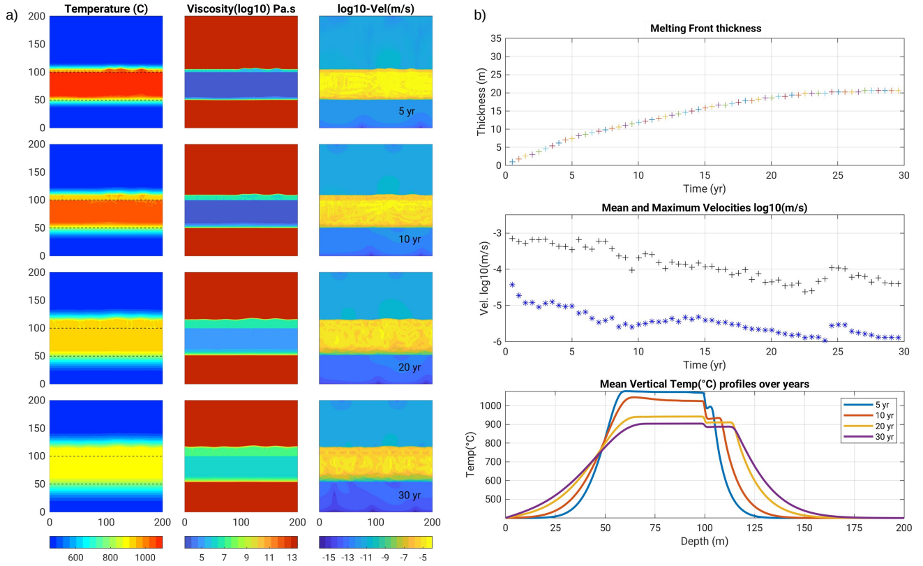
Figure C2. 50 m thick initial basalt intrusion (model BT50.4_v2_m5-100), for which secondary convection still occurs after 30 years, but only over ca. 20 meters. Legend same as previous figure. The 400 °C thermal jump after 30 years now occurs over ca. 25 m, corresponding to 16°C/m. Hence a 50 m thick intrusion may be just sufficient to explain the observed thermal gradient during the IDDP-1 drilling.
