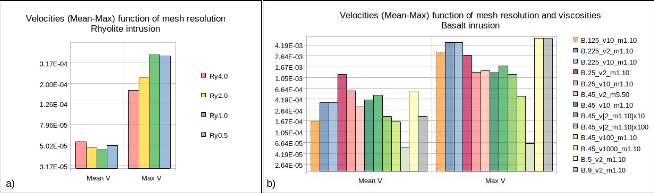
Figure B1. Mean and maximum velocities for model cases (ordinates in exponential scale of m/s). a) Rhyolite intrusion, for 4 different mesh resolutions. b) Basalt intrusion, for different mesh resolutions and different extrema viscosities. Only cases that could exceed 15 years are displayed. See Table 3 for details.
