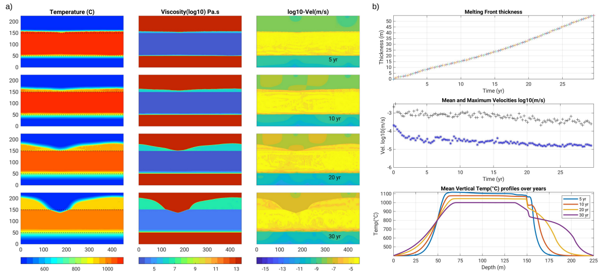
Figure B6. Case with a 100 m thick basalt intrusion and a weak host rock (maximum kinematic viscosity reduced to 5 \cdot 10^9 m^2/s , model B0.5_v2_m0.5-0.5): the latter destabilizes within ca. 15 years, producing diapirism of the partially molten host rock and smoothing out of the thermal gradient. This case may represent a mechanically weakened host rock due to hydrothermal fluid circulations, a hypothesis ruled out for the IDDP-1 context also based on petrological information (see Discussion section).
