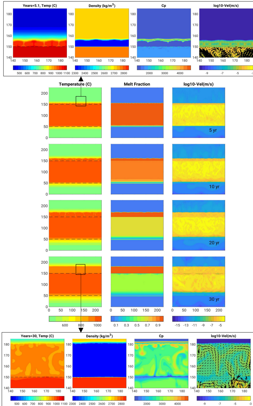
Figure B2. Basalt intrusion scenario (2) with greater mesh cell size 0.45 m (model B.45_v2_m5-50) than the case displayed in Figure 7 with cell size 0.25 m, for comparison: behavior is similar. Similar legend except that zoom snapshots are after 5 years and 30 years here.
